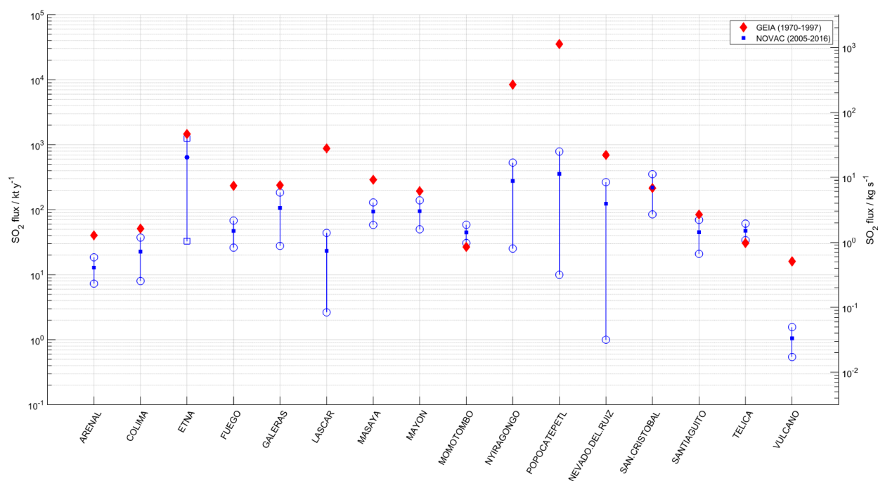
605 Figure 6. Comparison of emission statistics for 16 volcanoes of the NOVAC and GEIA datasets. For NOVAC the simple averages of annual mean (filled blue dots) and \pm 1 standard deviations (un-filled blue dots) for the years 2005-2016 are depicted. The values for GEIA are obtained from Andres and Kasgnoc (1998), for passive degassing and sporadically degassing volcanoes only.
