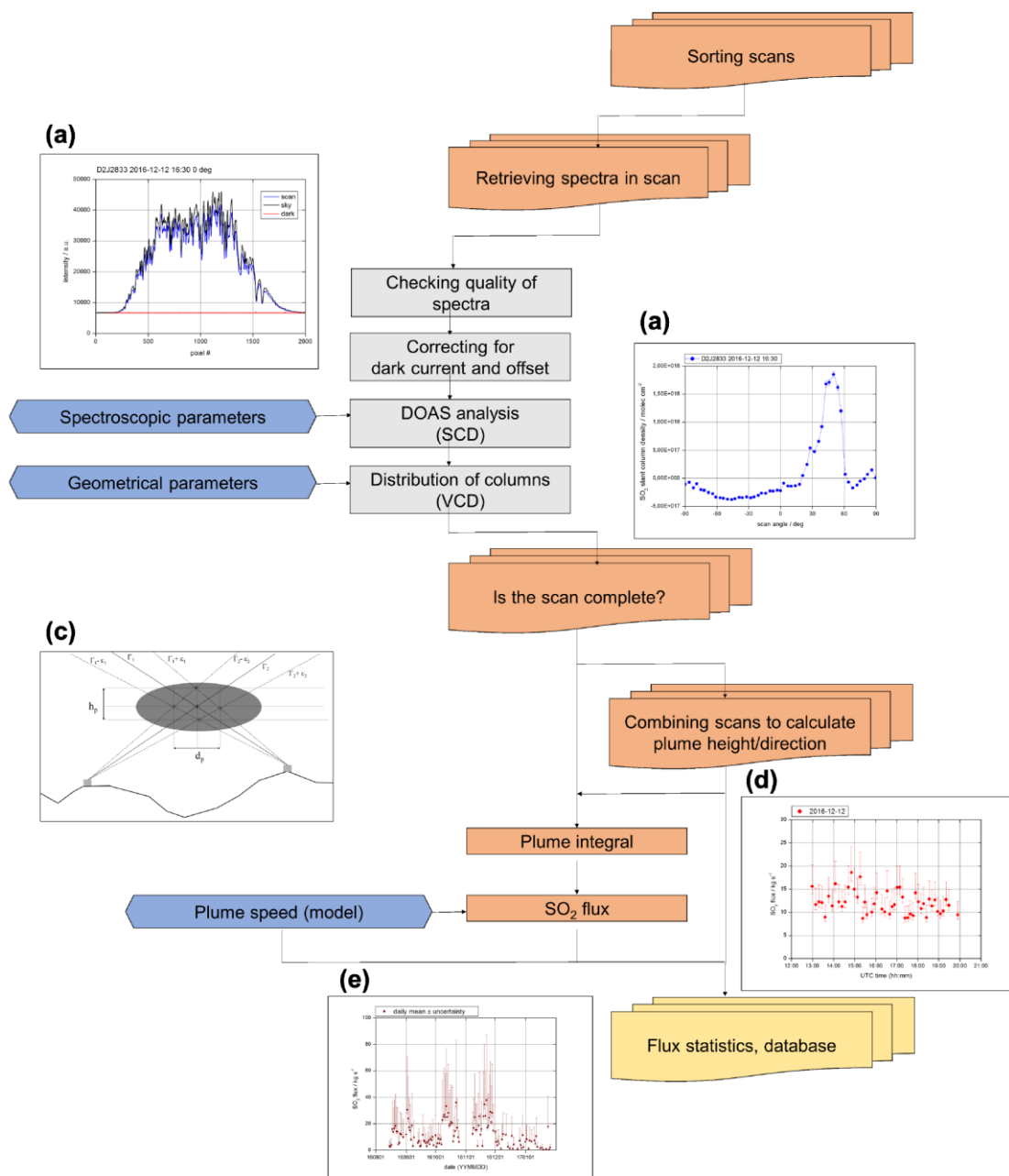
Figure 2. Schematics of the algorithm used to derive time-average emission of volcanoes in the NOVAC database. (a) Scattered sunlight spectra are checked for quality and combined to correct instrumental effects and to derive differential slant column densities of \text{SO}_2 through the non-linear DOAS method. (b) A collection of column densities in the scan is used to determine the baseline column density, the angular position of the centre of mass of the plume and to estimate the completeness of the scanned plume. (c) Pairs of scans taken close in time by different instruments are used to derive plume altitude and direction. Plume speed is obtained from a meteorological model to derive the flux, including uncertainty. (d) Individual flux measurements are chosen considering uncertainty, completeness and other criteria. (e) When at least five valid measurements exist on a given day, statistics are computed and reported in the NOVAC database.
