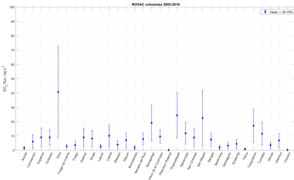
Figure 4. Statistics of daily SO 2 emission from 32 volcanoes in NOVAC from 1 March 2005 to 31 January 2017. Blue markers show the average of all measured fluxes for each volcano during this period and the error bars show the corresponding 25 and 75% quantiles.
