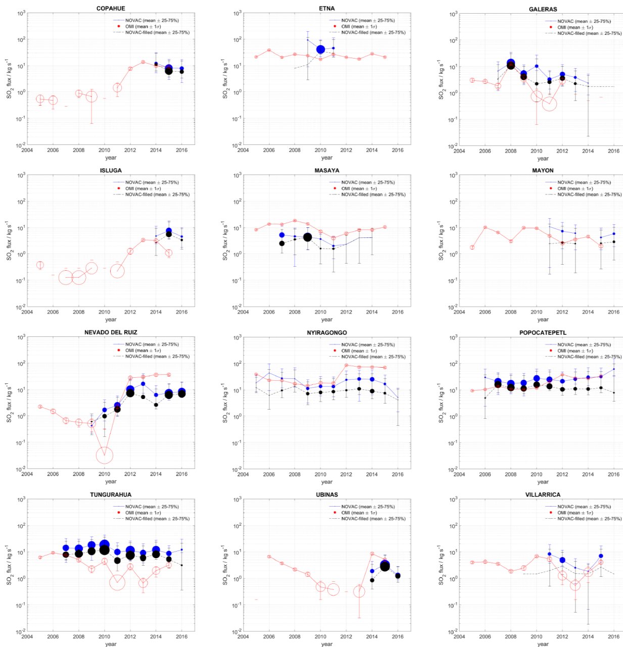
595 Figure 5. Time series of annual SO 2 emission from 12 volcanoes in NOVAC for which corresponding results from OMI are available for the period 2005-2016. Dots show the annual mean emission rate with size proportional to the number of valid measurements used for the average. The bars indicate 25 and 75% quantiles of the daily means on each year. The series shown in blue correspond to observed plumes, while in black is the emission adjusted for periods of low degassing, when no plumes were observed (see text for details). The series in red is the mean annual emission rate obtained from OMI measurements, with size proportional to the precision of the estimation and bars showing ±1 standard deviation (more details in Carn et al., 2017). For details of the data in numerical format see Supplementary Information SI2. 600
