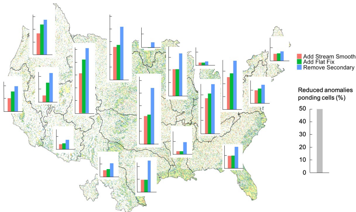
425 Figure 10: The background map is the ponding depth from runoff test at hour 20 with the final slope; barplots are the percentage decrease of anomalies ponding cells (ponding depth over 0.1m) outside the main stream network relative to the baseline (No Smooth case) in HUC2s. The scale of barplot in each HUC is the same with the grey bar shown in the right of figure.
