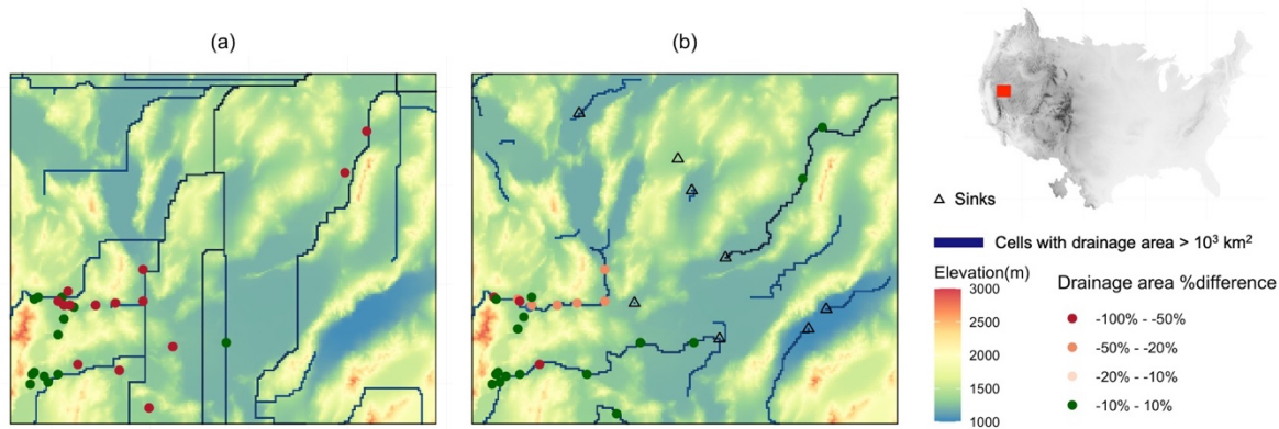
315 Figure 5: (a) and (b) Maps illustrating the effect of sinks in drainage network derivation, a selected domain in Great Basin (the highlighted red box in the upper-right CONUS map). In (a) and (b), the background is the elevation map; blue cells are the cells with drainage area over 1,000 km 2 from processing; colored dots represent the percentage difference of drainage area between processed and USGS observations (a)without sinks and (b)with pre-defined sinks
