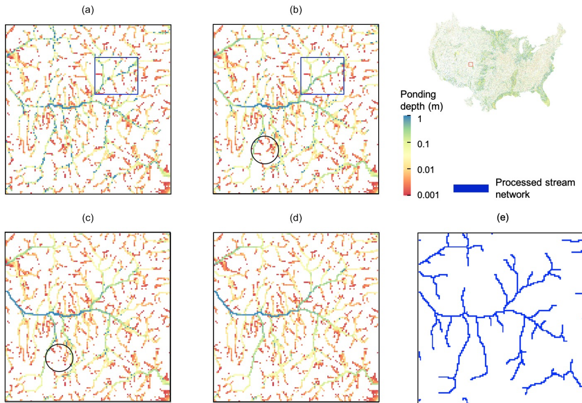
395 Figure 8: The ponding depth from runoff tests from four slope cases (a) No Smooth (b) Add Stream Smooth (c) Add Flat Fix (d) Remove secondary. (e) stream network from Priority Flood approach with drainage area over 100km 2 . The circles and boxes are examples to be explained in detail in the text.
