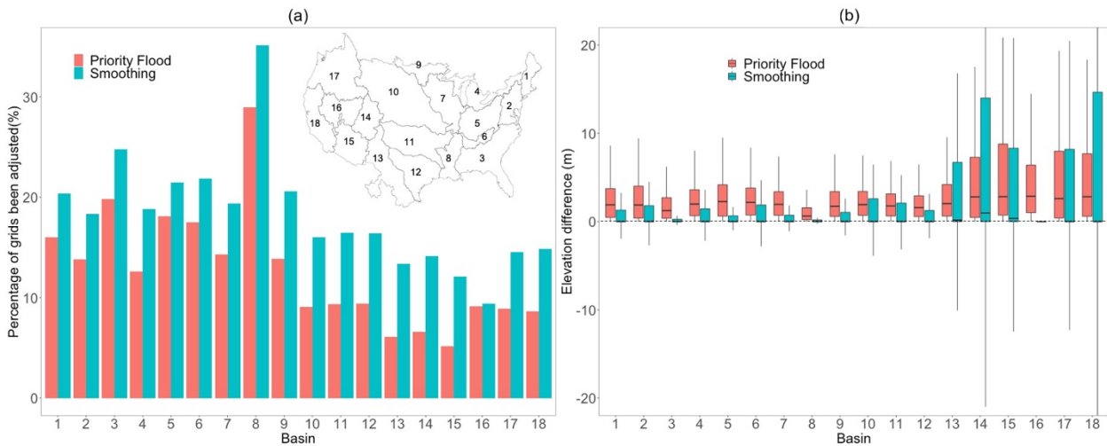
455 Figure 12: (a) the percentage of grids been processed in two processing parts in HUC2 basins; (b) the elevation difference after the two processing parts
