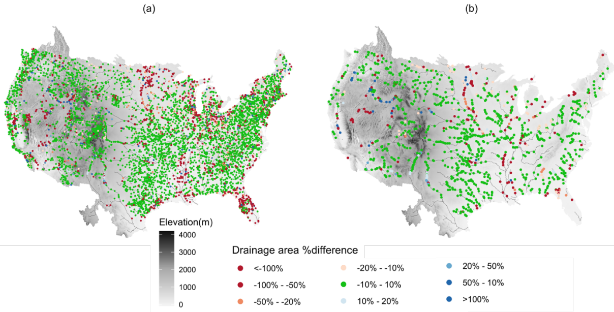
285 Figure 3: Drainage area comparison between processed with no initial stream network and USGS gage measurements. (a) all gages 290 for comparison; (b) gages with drainage area over 5000 km 2
