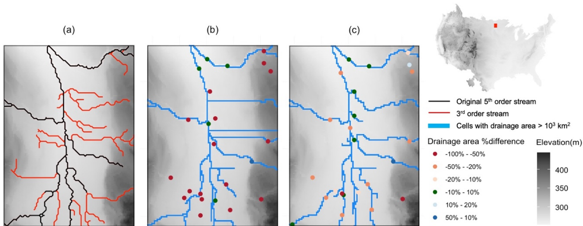
335 Figure 6: (a), (b) and (c) Maps illustrating the impact of stream order used for the drainage mask on the resulting drainage network for a selected valley in the northern portion of CONUS (highlighted in the red box in the upper-right CONUS map). The background map is the elevation. (a) the 3 rd (red) and 5 th (black) order stream network. (b) and (c) are results from 5 th order stream network and 3 rd stream network respectively. Blue cells in (b) and (c) are cells with drainage area over 1,000 km 2 after processing. Colored dots in (b) and (c) represent the percentage different of drainage area (colored dots) between topographic processed and USGS.
