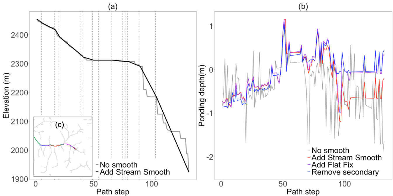
410 Figure 9: (a) The elevation along an example stream segment (shown in c) before and after smoothing applied along the stream; the stream is divided into segments by dashed lines; (b) the pondering depth along the main stem from the runoff tests with four slope cases; (c) the main stem with segments plotted by different colors
