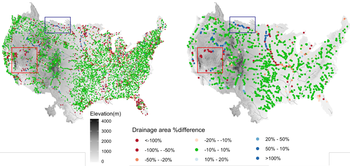
Figure 4: Drainage area comparison between processed with initial 5 th order stream network and USGS gage measurements. (a) all gages for comparison; (b) gages with drainage area over 5000 km 2
