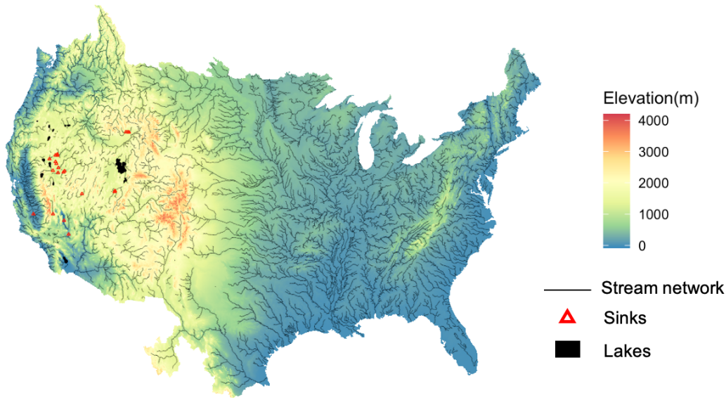
Figure 1: Map of the DEM datasets, stream network, lakes and sinks used for processing the 1km dataset.
