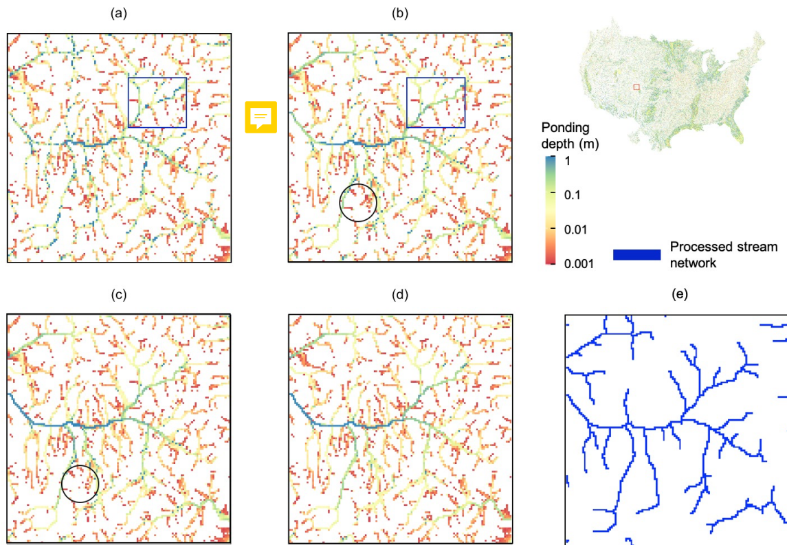
395 Figure 8: The ponding depth from runoff tests from four slope cases (a) No Smooth (b) Add Stream Smooth (c) Add Flat Fix (d)Remove secondary. (e) stream network from Priority Flood approach with drainage area over 100km 2 . The circles and boxes are examples to be explained in detail in the text.
