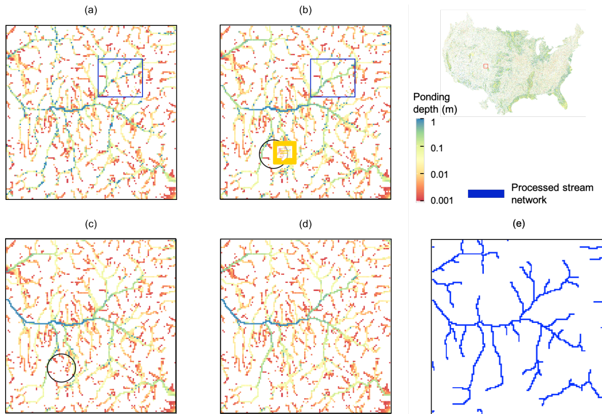
385 Figure 8: the spatial distribution of ponding depth from runoff tests from four slope cases (a) No Smooth (b) Add Stream Smooth (c) Add Flat Fix (d) Remove secondary slope. (e) stream network from Priority Flood approach with drainage area over 100km 2
