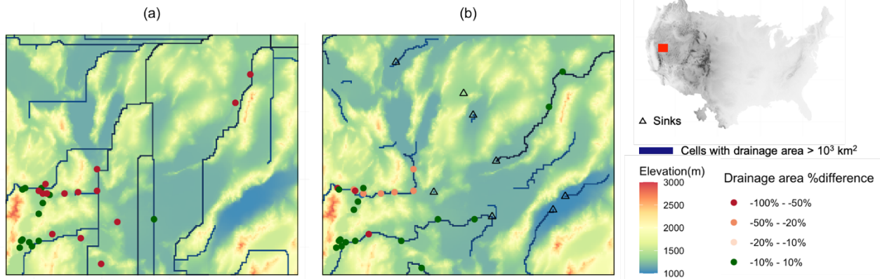
310 Figure 5: input topographic map (background of (a) and (b)) of a portion in the Great Basin shown as the red box in the upper-right CONUS map; the drainage network (blue cells (a) and (b)); the percentage different of drainage area (colored dots) between processed and USGS observations (a) without sinks and (b) with pre-defined sinks
