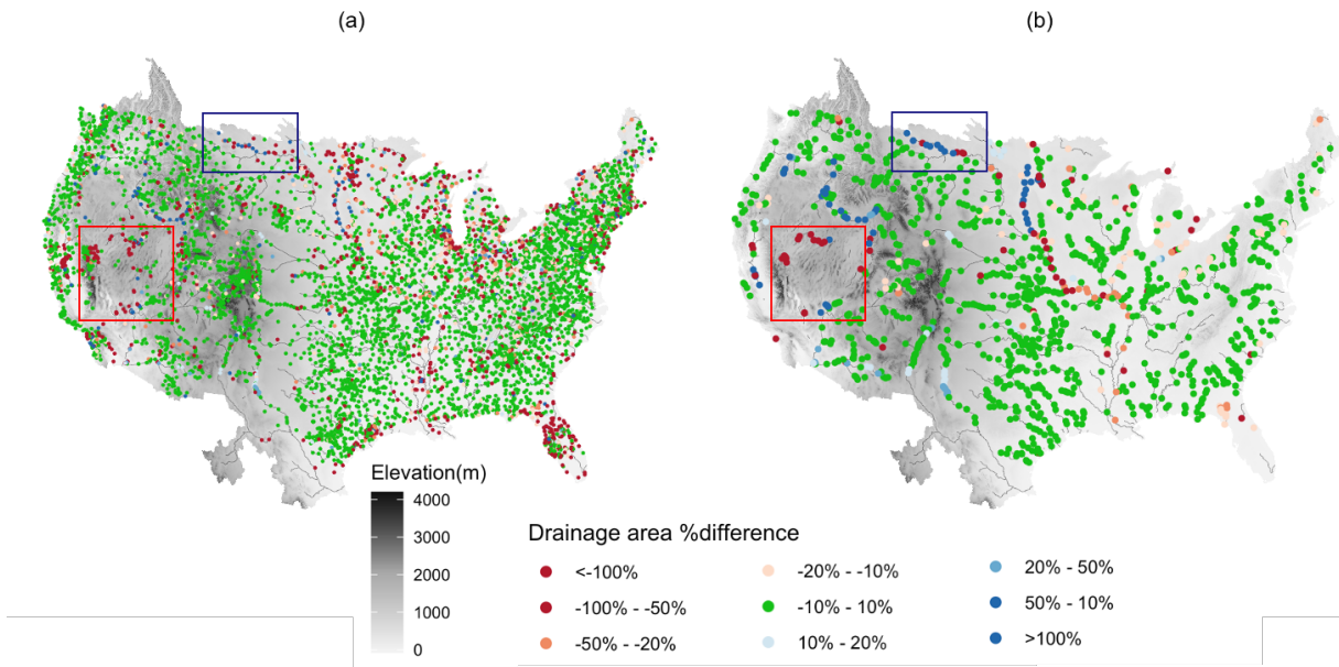
290 Figure 4: Drainage area comparison between processed with initial 5 th order stream network and USGS gage measurements. (a) all gages for comparison; (b) gages with drainage area over 5000 km 2
