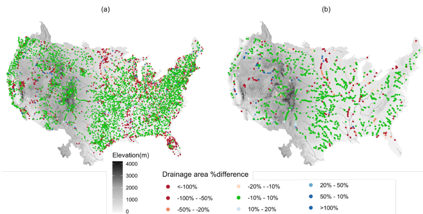
370 Figure 3: Drainage area comparison between processed with no initial stream network and USGS gage measurements. (a) all gages for comparison; (b) gages with drainage area over 5000 km 2
