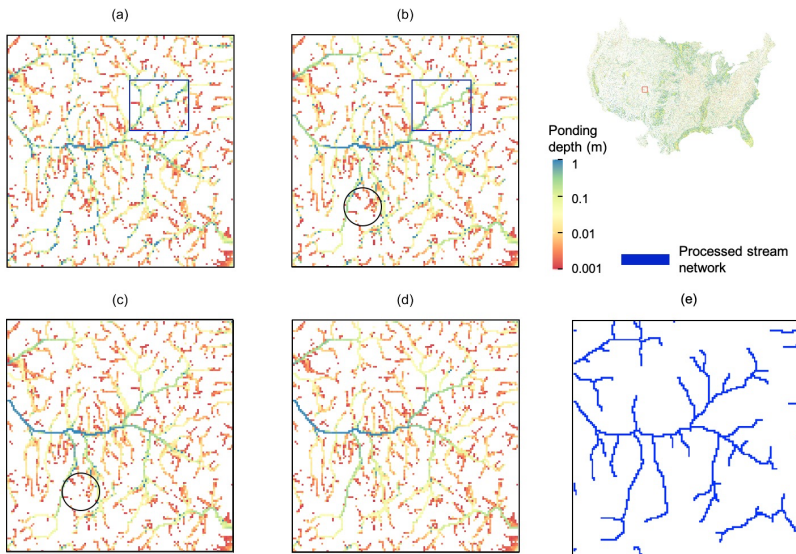
505 Figure 8: The ponding depth from runoff tests from four slope cases (a) No Smooth (b) Add Stream Smooth (c) Add Flat Fix (d) Remove secondary. (e) stream network from Priority Flood approach with drainage area over 100km 2 . The circles and boxes are examples to be explained in detail in the text.
