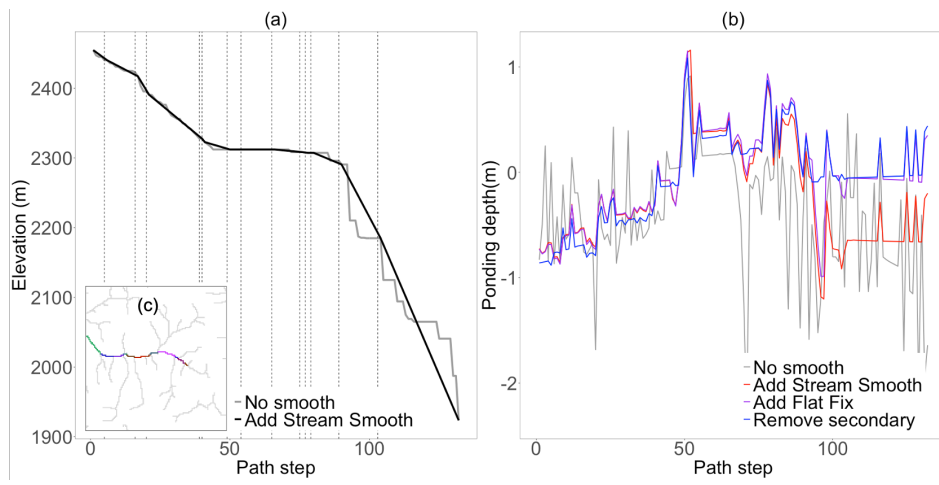
Fig. 1. Figure 9: (a) the elevation along an example stream segment (shown in c) before and after smoothing applied along the stream divided into segments by dashed lines; (b) the ponding depth along the ma
