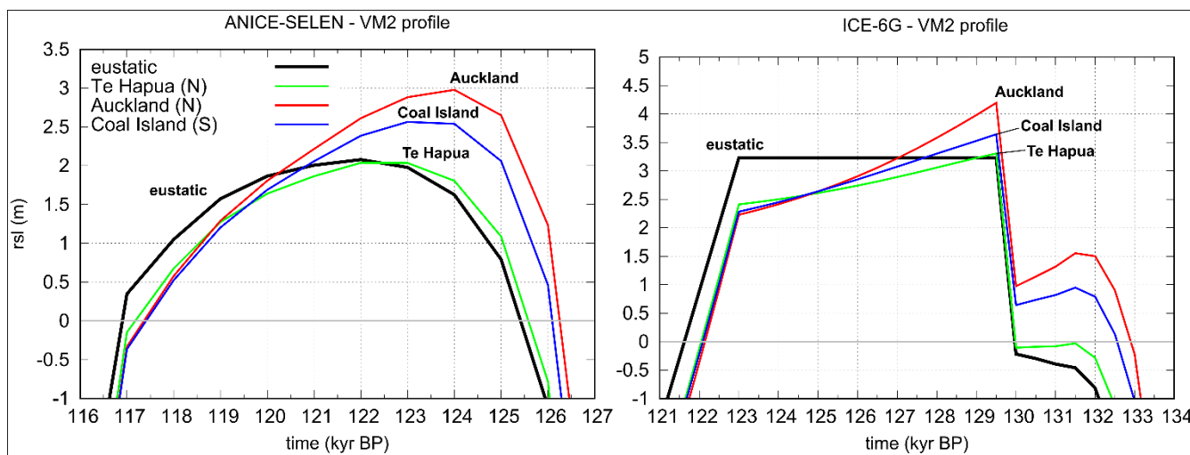
Figure 5: Local RSL curves for MIS 5e sea level at the northernmost tip of North Island (Te Hapua; latitude -34.39, longitude 173.02), Auckland (latitude -36.85, longitude 174.76), and the southernmost tip of South Island (Coal Island; latitude -46.21, longitude 166.66) generated from ANICE-SELEN and ICE-6G models. Similar to the Holocene, sea level peaks earlier and higher in the North Island. The Northland region (Te Hapua) RSL curve is nearest to eustatic. Deviations of the RSL curves from eustatic within the models is driven by ocean syphoning, suggesting it serves as a primary driver of variability in the timing and height of peak sea level across New Zealand. Note the different scale to x- and y- axes between model outputs.
