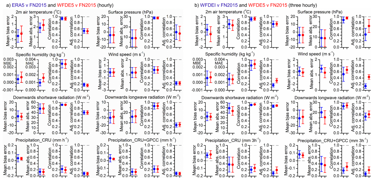
Figure 2. Average metrics (mean \pm 95% confidence interval of the mean) for: a) ERA5 v FN2015 (blue) and WFDE5 v FN2015 (red) at hourly time steps (see Table A17); b) WFDEI v FN2015 (blue) and WFDE5 v FN2015 (red) at three-hourly time steps (see Table A18).
