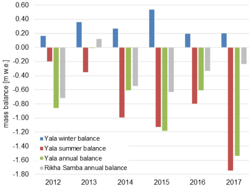
Figure 4: Winter, summer and annual mass balance of Yala Glacier and annual balance of Rikha Samba Glacier, calculated based on the respective gradients. In the mass-balance years 2011/12 and 2014/15, the sum of winter and summer balances differ significantly from the annual balances, likely due to a lack of data in higher elevations. The summer balance from 2011/12 and winter balance from 2014/15 have not been reported to the WGMS.
