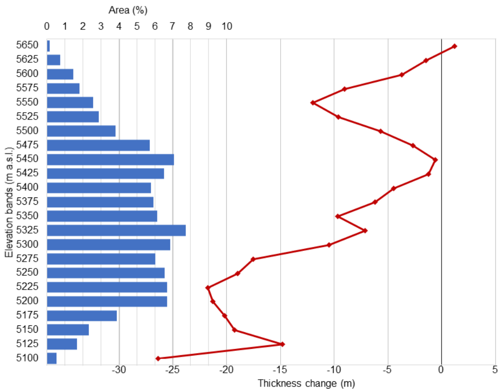
535 Figure 8: The mean thickness changes of Yala Glacier for 25 m elevation bands with hypsography, from 2000 to 2012. The reduced thickness change at an elevation of 5125 m is likely a result of the thinner ice thickness in the steeper part of the glacier in 2000. The increased thinning between 5525 and 5575 m a.s.l. might be caused by increased ablation at steep slopes and ice cliffs.
