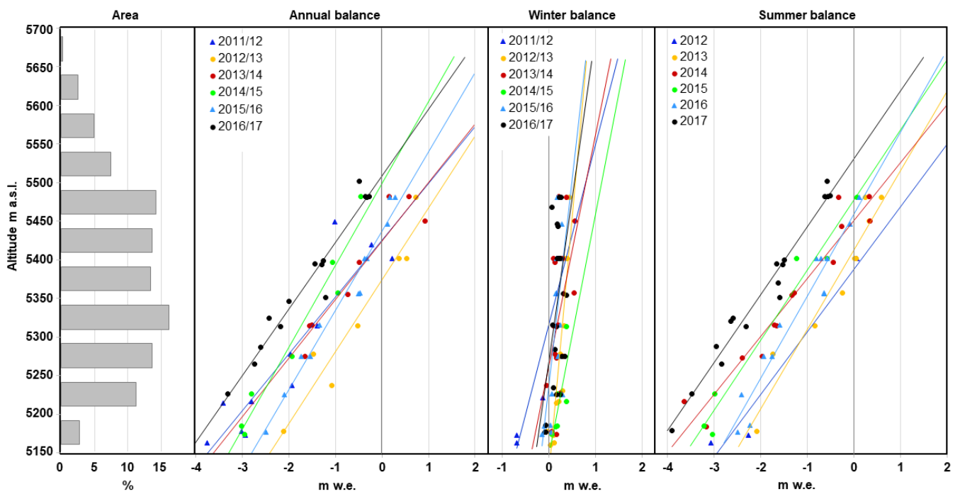
Figure 2: Mass balances and gradients for the annual, winter and summer mass balance for Yala Glacier from 2011–2017, and the glacier hypsography (far left).
