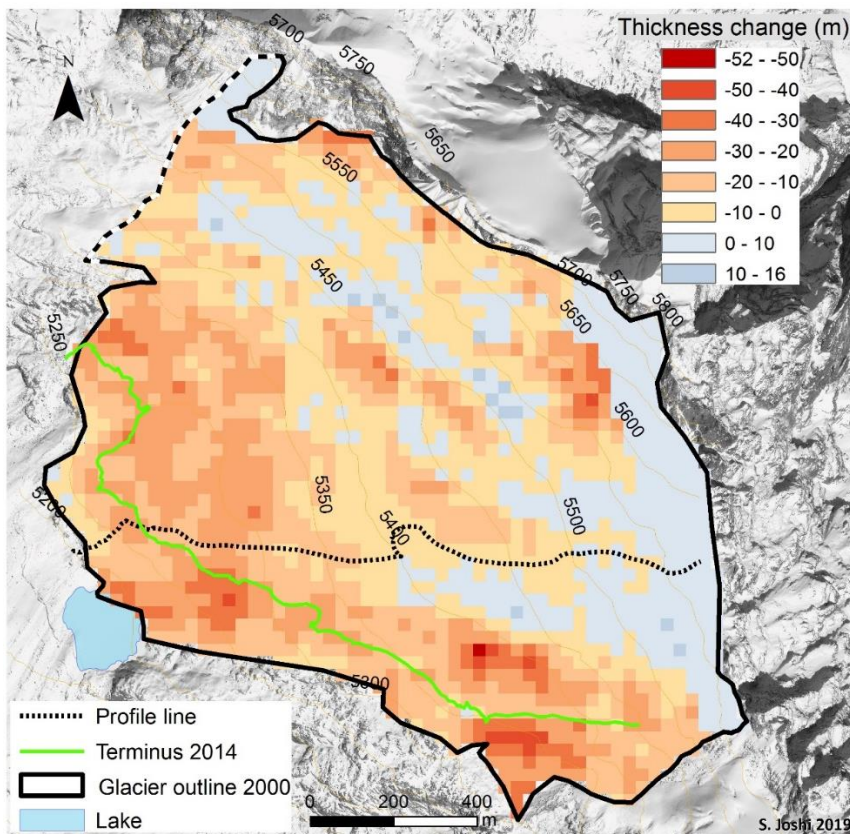
530 Figure 7: Thickness changes of Yala Glacier in metres after DEM differencing of GeoEye-1 (Jan 2012) and SRTM3 (Feb 2000) DEM and dGNSS profile in 2012.
