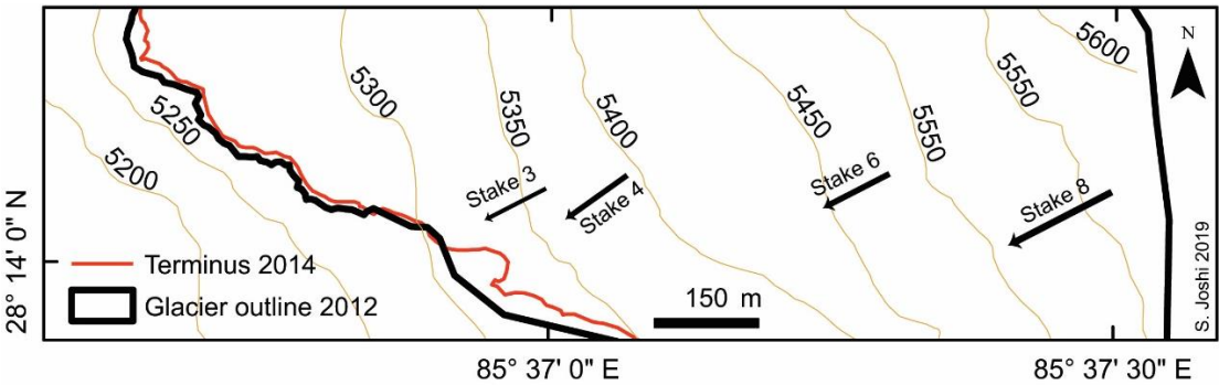
Figure 11: Glacier flow from 8 May 2012 to 5 May 2014 at the stakes 3, 4, 6 and 8, with annual rates between 4.6 and 7.8 m a -1 . The black arrows show the flow direction and the lengths indicate the annual speed of glacier surface flow, which is depicted 10 times longer than the real flow (Figure adapted from Sugiyama et al., 2013).
