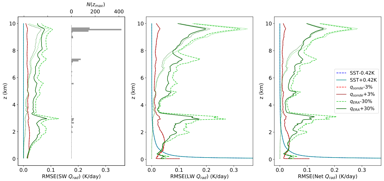
Figure 7. Root-mean-square error estimates in shortwave (left), longwave (center) and net heating rates (right) for perturbations in SST skin (blue), ERA5 humidity profiles (green) and sonde humidity measurements (red) for the 1314 daytime profiles that have valid data starting at 40 m. Dashed curves show negative perturbations, solid curves show positive perturbations and dotted green curves show ERA5 humidity perturbations restrained to the 1117 daytime profiles that have valid data at all levels between 40 m and 8 km. The horizontal grey bars on the left panel show the frequency distribution in the maximum level measured ( z_{max} ).
