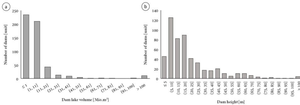
Figure 5 – Lake volume (a) and dam height (b).
