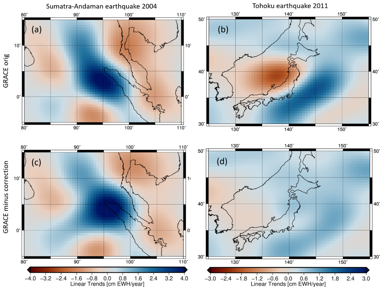
Figure 87: Linear trends (01/2003 – 12/2016) of TWS changes (cm EWH/year), before and after removing earthquake signals of the Sumatra-Andaman earthquake from 2004 ((a) before, (c) after) and the Tohoku earthquake from 2011 ((b) before, (d) after).
