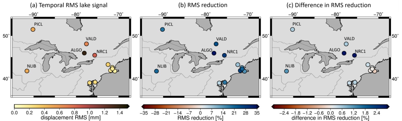
Figure 119: Temporal RMS of the vertical displacement caused by the forward-modelled lake/reservoir signal of RECOG-LR (left), reduction of RMS of GNSS time series after subtracting modelled deformation (middle) and difference in RMS reduction when subtracting GRACE after removing and relocating RECOG-LR vs. using the uncorrected GRACE signal.
