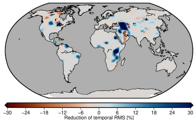
(b) RMS reduction of GRACE time series
