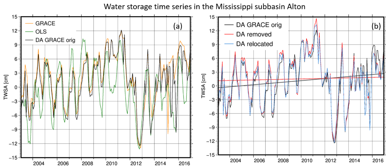
Figure 10: Time series of TWSA in the Alton subbasin: original GRACE observations (orange), Ensemble mean of open loop WaterGAP simulations (green), model results after assimilating the original GRACE-derived TWSA (without applying any corrections, black), model results after assimilating the removed product (red) and after assimilating the relocated product (blue).
