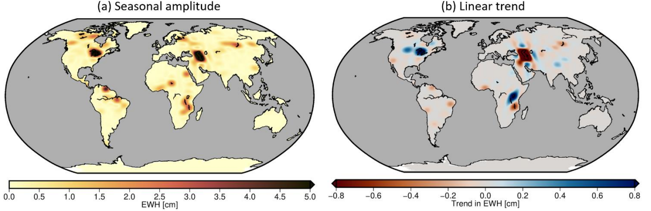
Figure 43: RECOG-LR on a global scale with its (a) mean seasonal amplitude and (b) trend.
