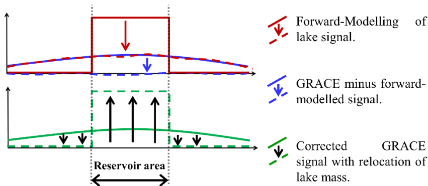
Figure 3: Scheme of forward-modelling approach. Removal (top) and relocation (bottom) of lakes and reservoirs.
