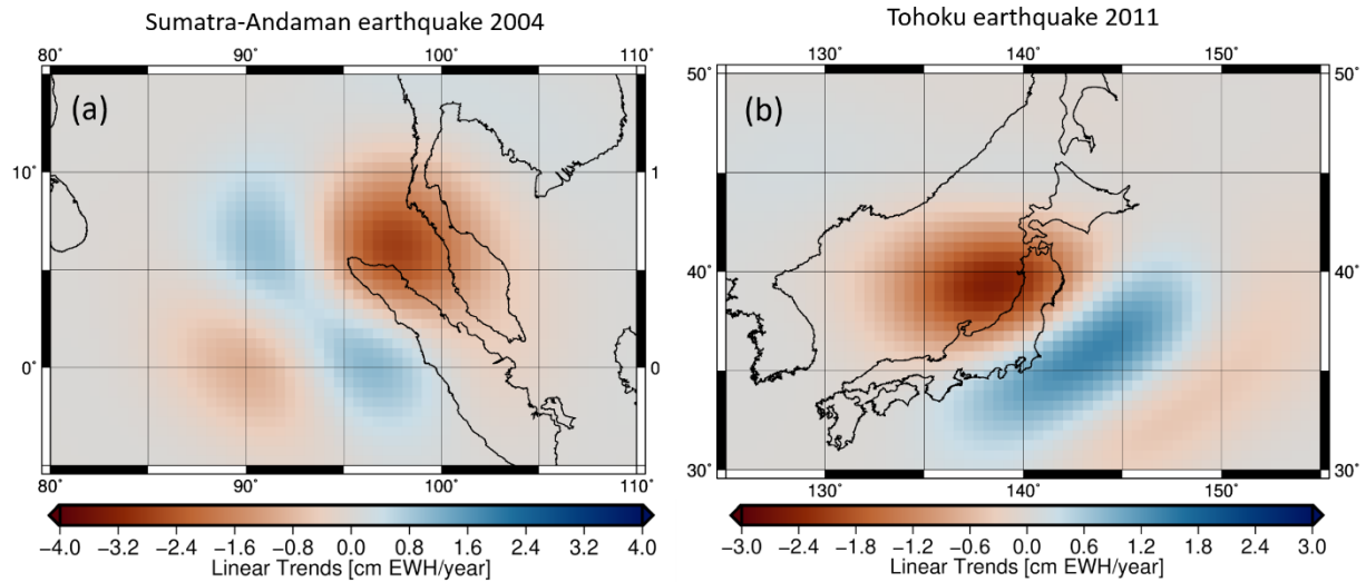
Figure 54: Linear trends (01/2003 – 12/2016) of TWS changes (cm EWH/year), of the earthquake correction that includes the (a) Sumatra-Andaman earthquake from 2004 and the (b) Tohoku earthquake from 2011.
