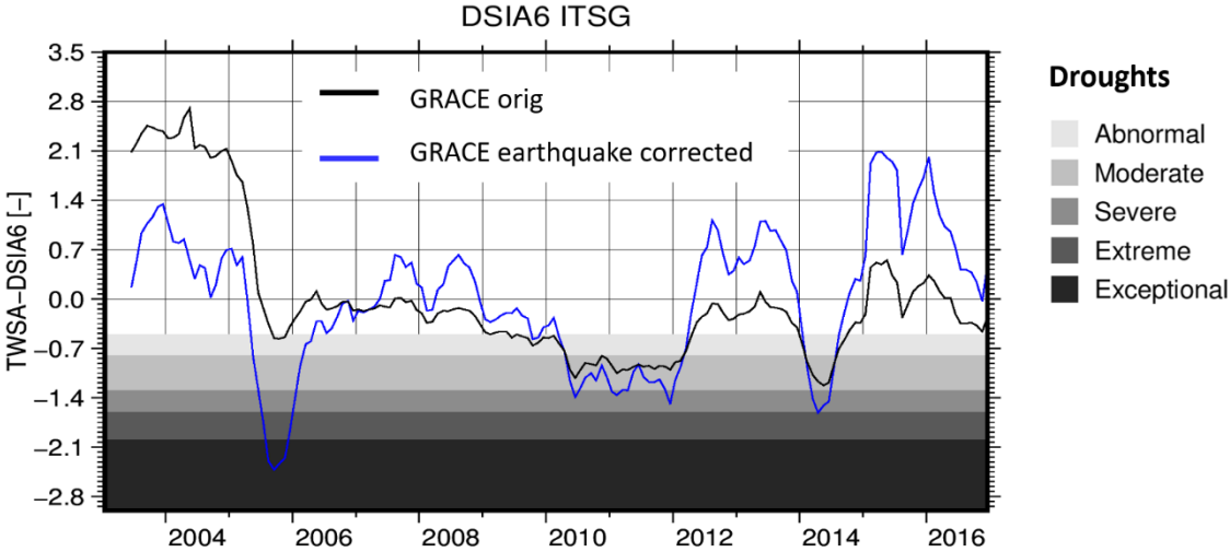
Figure 120: GRACE-derived TWSA-DSIA6 over the Malaysian peninsular (West Malaysia) shown without (black) and with (blue) earthquake correction.
