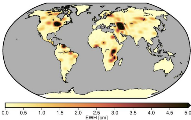
(a) Temporal RMS of lake/reservoir correction
