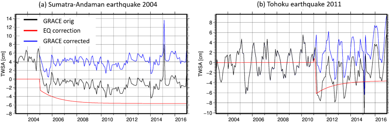
Figure 98: Spatially averaged GRACE TWS anomalies for the original (black) and earthquake corrected (blue) GRACE data and its correction (red) for (a) the Malaysian peninsular (West Malaysia) and (b) Japan.
