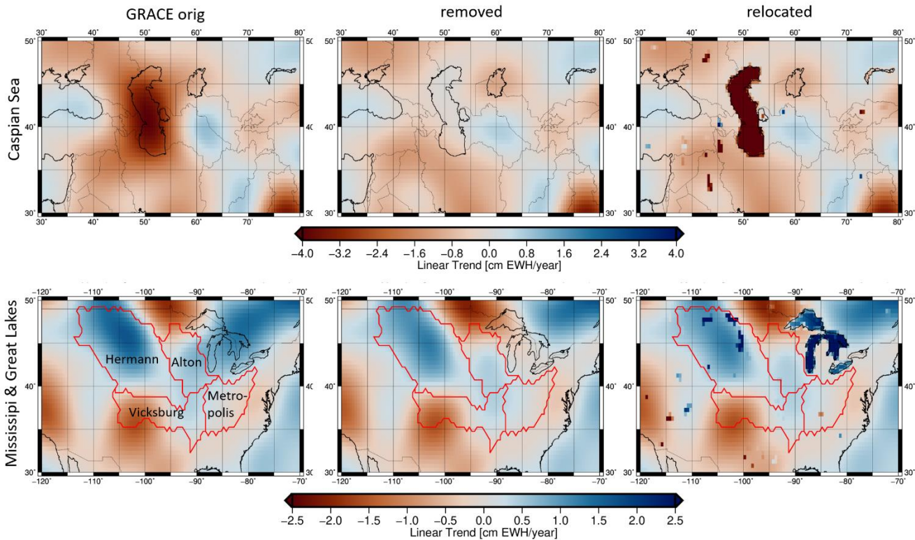
Figure 76: Linear trend of GRACE-TWS anomalies (01/2003 – 12/2016) in the Caspian Sea region (top) and in the Mississippi basin and around the Great Lakes (bottom) without any correction (left), after removing the influence of lakes (middle) and after relocating the lake signal (right). Please note that the Aral Sea has been excluded from RECOG-LR RL01 due to its strongly varying surface area, which is not yet captured in the database.
