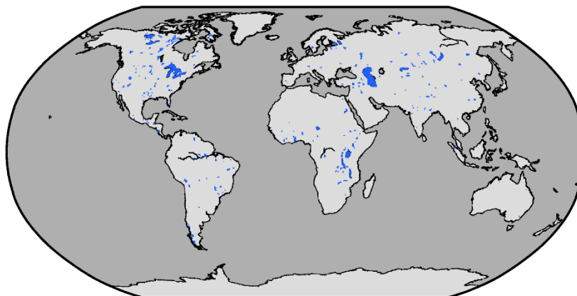
Surface water bodies included in RECOG-LR RL01
