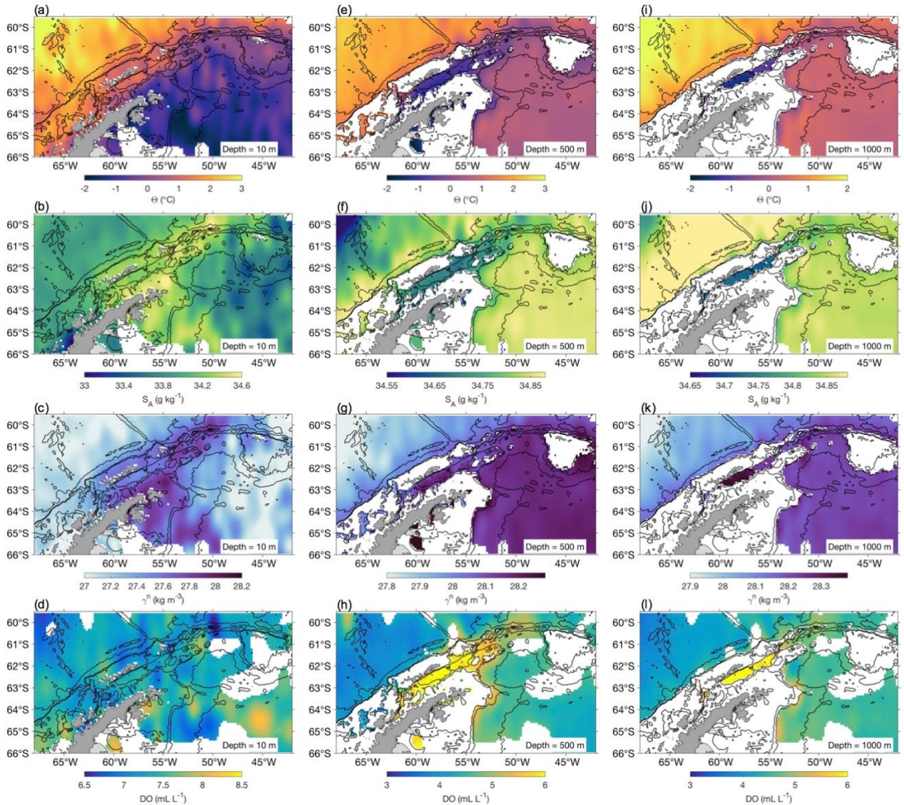
Figure 6. Surface maps of NAPv1.0 at 10 m (left panels), 500 m (middle panels) and 1000 m (right panels) depth for summer. (a, e, i) Conservative temperature ( \Theta ; °C). (b, f, j) Absolute salinity ( S_A ; g kg -1 ). (c, g, k) Neutral density ( \gamma^n ; kg m -3 ). (d, h, l) Dissolved oxygen (DO; mL L -1 ). ETOPO1 isobaths of 500 m, 1000 m, 3000 m and 5000 m are depicted by the black lines. Coastline from SCAR Antarctic Digital Database.
