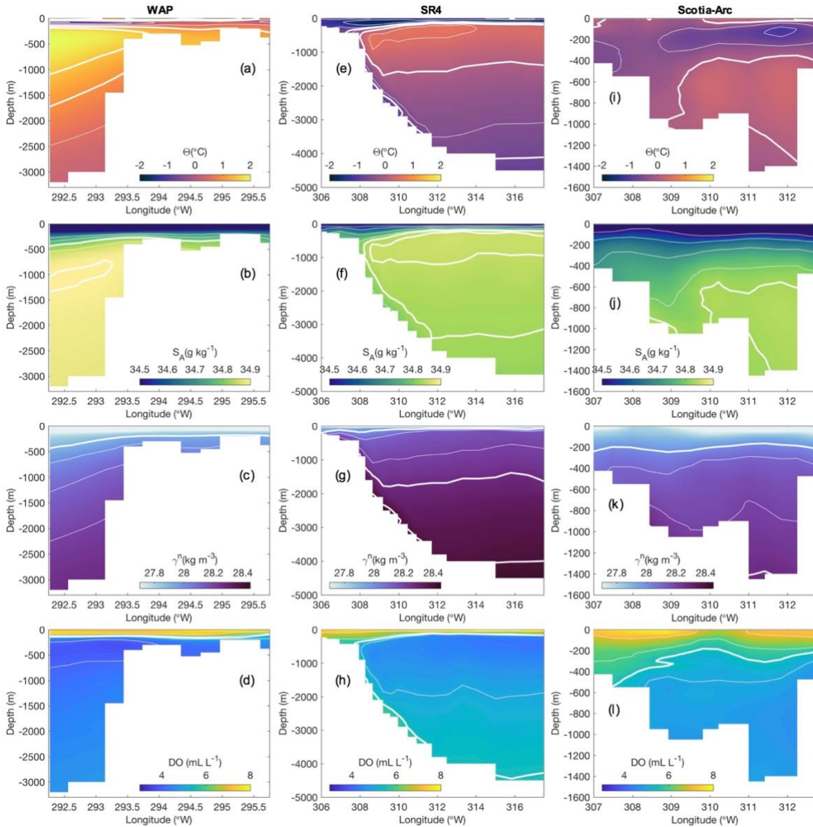
Figure 11. Summer vertical sections along the Western Antarctic Peninsula (WAP; a-d; magenta line in Fig. 1a), WOCE SR4 across the Weddell Gyre (e-h; green line in Fig. 1a), and Scotia-Arc line over the South Scotia Ridge (i-l; cyan line in Fig. 1a). (a) Conservative temperature ( \Theta ; ^{\circ}\text{C} ) with isotherms of 1^{\circ}\text{C} and 1.5^{\circ}\text{C} ( -1.5^{\circ}\text{C} to 1.5^{\circ}\text{C} every 0.5^{\circ}\text{C} ) shown by the thick (thin) white line. (b) Absolute salinity ( S_A ; \text{g kg}^{-1} ) with isolines of 34.8 \text{ g kg}^{-1} and 34.9 \text{ g kg}^{-1} ( 34.7 \text{ g kg}^{-1} to 34.9 \text{ g kg}^{-1} every 0.05 \text{ g kg}^{-1} ) shown by the thick (thin) white line. (c) Neutral density ( \gamma^n ; \text{kg m}^{-3} ) with isoline of 27.9 \text{ kg m}^{-3} ( 28.0 \text{ kg m}^{-3} to 28.2 \text{ kg m}^{-3} every 0.1 \text{ kg m}^{-3} ) shown by the thick (thin) white line. (d) Dissolved oxygen ( \text{DO} ; \text{mL L}^{-1} ) with isoline of 5.5 \text{ mL L}^{-1} ( 4 \text{ mL L}^{-1} to 8 \text{ mL L}^{-1} every 1 \text{ mL L}^{-1} ) shown by the thick (thin) white line. (e) \Theta with isotherms of -0.7^{\circ}\text{C} and 0^{\circ}\text{C} ( -1.5^{\circ}\text{C} to 1.5^{\circ}\text{C} every 0.5^{\circ}\text{C} ) shown by the thick (thin) white line. (f) S_A with isolines of 34.83 \text{ g kg}^{-1} and 34.85 \text{ g kg}^{-1} ( 34.5 \text{ g kg}^{-1} to 34.8 \text{ g kg}^{-1} every 0.1 \text{ g kg}^{-1} ) shown by the thick (thin) white line. (g) \gamma^n with isolines of 28.0 \text{ kg m}^{-3} , 28.27 \text{ kg m}^{-3} and 28.4 \text{ kg m}^{-3} ( 28.0 \text{ kg m}^{-3} to 28.2 \text{ kg m}^{-3} every 0.1 \text{ kg m}^{-3} ) shown by the thick (thin) white line. (h) Same as panel (d). (i) \Theta with isotherms of 0^{\circ}\text{C} ( -1.5^{\circ}\text{C} to 1.5^{\circ}\text{C} every 0.5^{\circ}\text{C} ) shown by the thick (thin) white line. (j) S_A with isoline of 34.83 \text{ g kg}^{-1} ( 34.5 \text{ g kg}^{-1} to 34.8 \text{ g kg}^{-1} every 0.1 \text{ g kg}^{-1} ) shown by the thick (thin) white line. (k) \gamma^n with isolines of 28.0 \text{ kg m}^{-3} and 28.27 \text{ kg m}^{-3} ( 28.0 \text{ kg m}^{-3} to 28.2 \text{ kg m}^{-3} every 0.1 \text{ kg m}^{-3} ) shown by the thick (thin) white line. (l) Same as panel (d).
