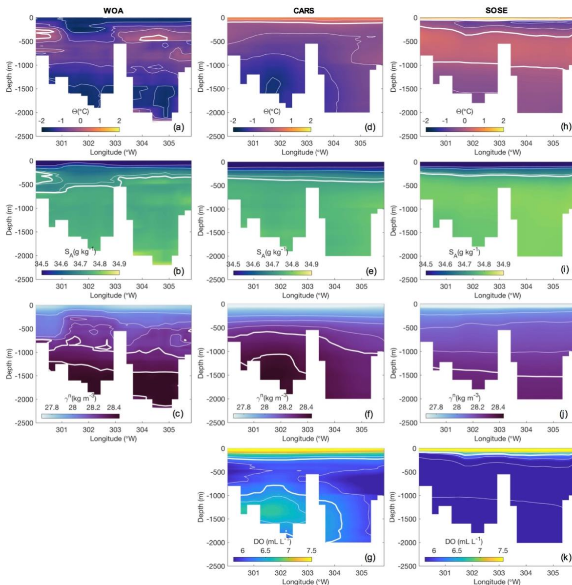
Figure 13. Summer vertical sections along the Bransfield Strait from WOA, CARS, SOSE. (a) WOA conservative temperature ( \Theta ; ^{\circ}\text{C} ). Isotherm of 0^{\circ}\text{C} is shown by the thick white line. Thin lines show the isotherms of -1.5^{\circ}\text{C} to 1.5^{\circ}\text{C} every 0.5^{\circ}\text{C} . (b) WOA absolute salinity ( S_A ; \text{g kg}^{-1} ). Isolines of 34.72 \text{ g kg}^{-1} is shown by the thick white line. Thin lines show the isolines of 34.5 \text{ g kg}^{-1} and 34.7 \text{ g kg}^{-1} every 0.1 \text{ g kg}^{-1} . (c) WOA neutral density ( \gamma^n ; \text{kg m}^{-3} ). Isolines of 28.27 \text{ kg m}^{-3} and 28.4 \text{ kg m}^{-3} is shown by the thick white line. Thin lines show the isolines of 28 \text{ kg m}^{-3} and 28.2 \text{ kg m}^{-3} every 0.1 \text{ kg m}^{-3} . (d) Same as panel (a), but for CARS. (e) Same as panel (b), but for CARS. (f) Same as panel (c), but for CARS. (g) CARS dissolved oxygen (DO; \text{mL L}^{-1} ). The isolines of 6.3 \text{ mL L}^{-1} is shown by the thick white lines. Thin lines show the isolines of 5.5 \text{ mL L}^{-1} and 7.0 \text{ mL L}^{-1} every 0.5 \text{ mL L}^{-1} . (h) Same as panel (a), but for SOSE. (i) Same as panel (b), but for SOSE. (j) Same as panel (c), but for SOSE. (k) Same as panel (g), but for SOSE.
