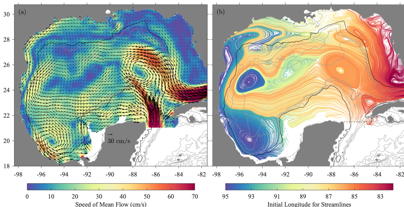
Figure 3. Panel (a) is the surface circulation in the Gulf of Mexico as in Fig. 2, but for the GulfFlow-1/12° product smoothed within 50 km radius circles as described in the text. Panel (b) shows streamlines of the mean flow in (a), colored according to their initial longitude.
