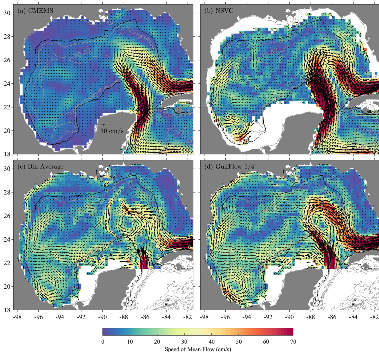
Figure 2. The mean surface circulation in the Gulf of Mexico in quarter-degree bins from (a) CMEMS satellite altimetry, (b) the drifter-based climatology of Laurindo et al. (2017), (c) a direct bin-averaging of all data in the GulfDriftersAll dataset, and (d) the time mean of monthly data from the GulfFlow-1/4° product, equivalent to a two-step temporal averaging of the GulfDriftersAll dataset. The colored shading gives the speed of the time-mean flow, also proportional to the length of the arrows. The scale for the arrows is shown in panel (a). For presentational clarity, arrows are shown on a decimated three-quarter degree grid. Bathymetric contours in this and following plots are as in Fig. 1.
