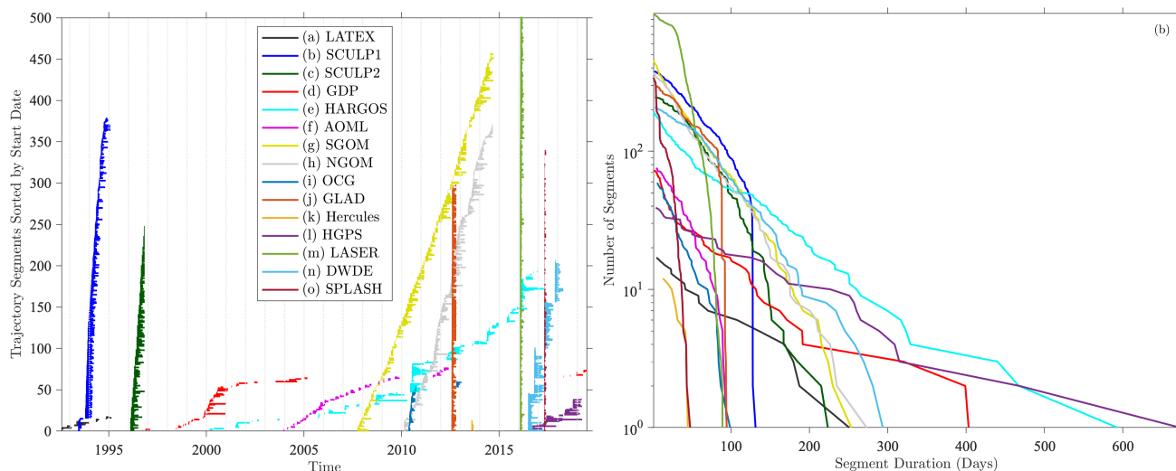
Figure 5. Temporal ranges (a) and durations (b) of drifter trajectory segments from the various sources, after the processing described in Sect. 4.1. In panel (a), each small horizontal line marks the temporal range of a different drifter trajectory. The y -axis is the trajectory segment number within each data source, sorted in order of the date of the first measurement point. For display purposes, the upper limit of the y -axis is set to 500 trajectories, although the LASER experiment has nearly 1000 trajectories. In panel (b), the lines show the number of trajectories exceeding a specified duration with a logarithmic y -axis. The lower limit of the y -axis is one, and gives the duration of the longest trajectory segment in each dataset.
