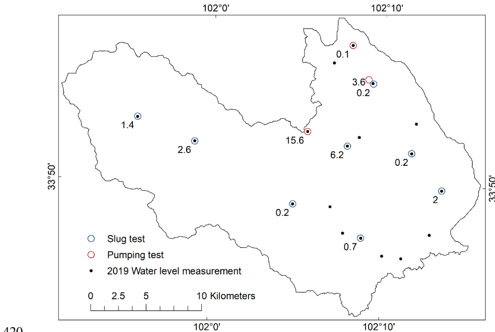
Figure 10. Hydraulic conductivity (m d -1 ) obtained from aquifer tests in Maqu catchment.
