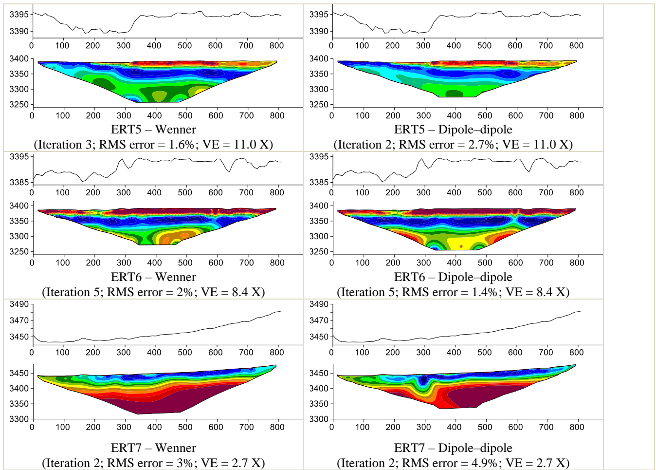
Figure A2. ERT measurements and corresponding ground surface elevation and vertical exaggeration (VE).
