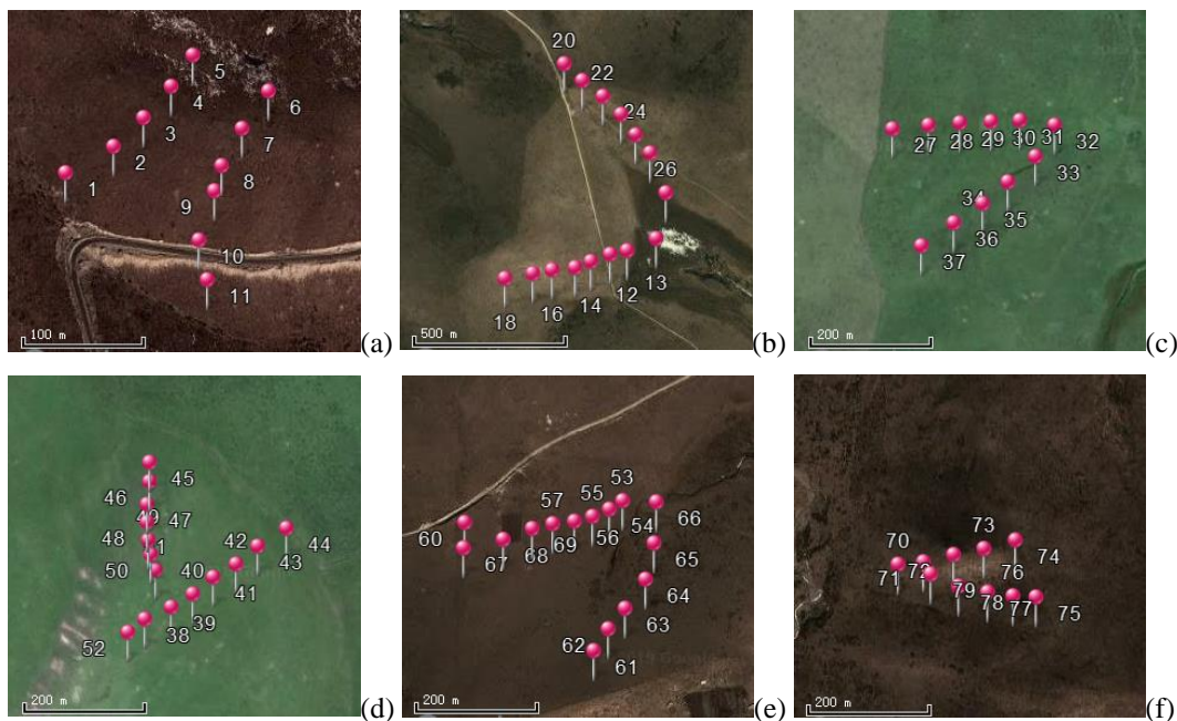
Figure 4. (a), (b), (c), (d), (e), and (f) are the exact locations of soil thickness measurements at the sites a, b, c, d, e, f, respectively shown in Fig. 3, in the *.KML formatted image from © Google Earth.
