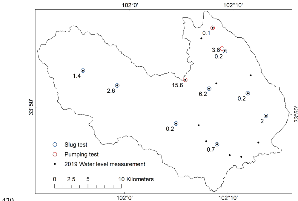
420 Figure 10. Hydraulic conductivity (m d -1 ) obtained from aquifer tests in Maqu catchment.
