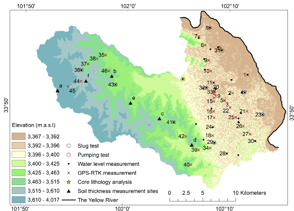
Figure 3. Locations of the hydrogeological surveys, ground surface elevation measurements, core lithology analysis, and soil thickness measurements. The numbers from 1 to 46 (due to limited space, several numbers are not shown in the figure) indicate the measurement sequence of GPS-RTK.
