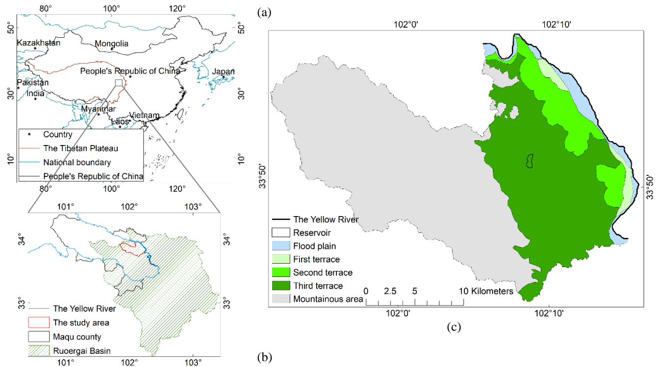
130 Figure 1. The geographical location of Maqu catchment, Maqu county, and Ruoergai basin on TP and geomorphologic map: (a) the geographical location and boundary of the TP (Zhang et al., 2014a; Zhang et al., 2014b); (b) the geographical location of the Maqu catchment, Maqu county, and Ruoergai basin (Li and Gao, 2019); (c) the geomorphologic map of Maqu catchment.
