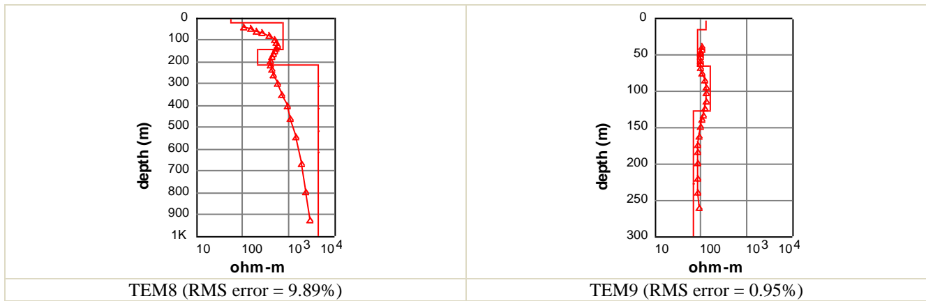
515 Figure 12. Apparent resistivity with depth. The red triangles connected by the red line represent the measured apparent resistivity values, and the red line without triangles represents the inverted 1-D geoelectric model.
