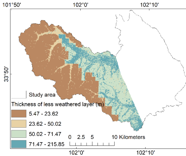
Figure 8. The estimated thickness of the less weathered layer in the west: (a) based on the ensemble model estimated depth to bedrock from Yan et al. (2020); (b) based on the depth to bedrock from Shangguan et al. (2017).
