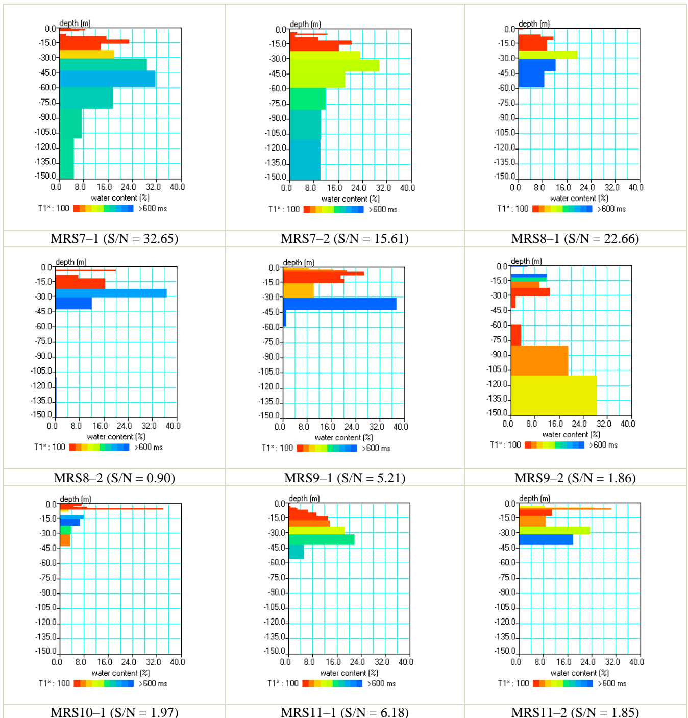
Figure A3. Water content and T1 derived from MRS measurements.
