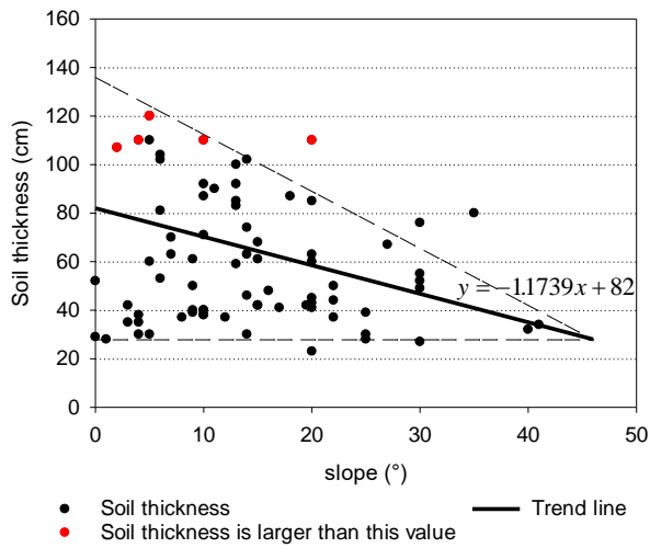
Figure 7. Soil thickness: (a) soil thickness (cm) vs. slope (°); (b) estimated soil thickness using eq. 9.
