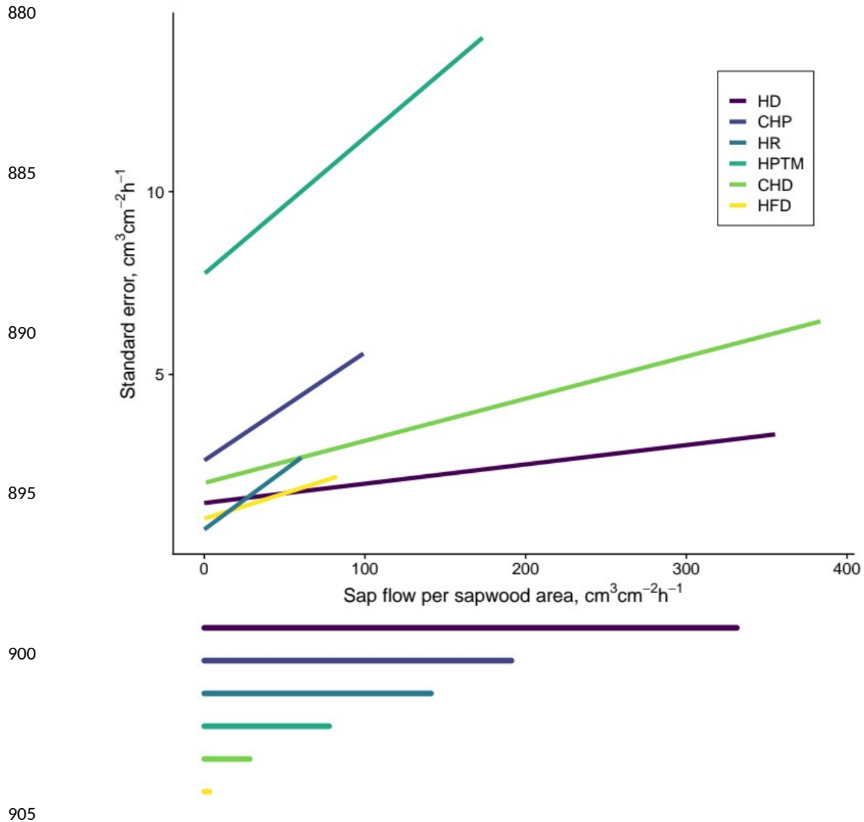
Figure B1. Methodological uncertainty estimation in sap flow density measurements based on the data from the global metaanalysis of sap flow calibrations in Flo et al. (2019). The main panel shows predicted standard error based on method-specific linear mixed models of reference flow as a function of measured flow including the individual calibration as a random intercept factor. The span of the horizontal lines below the main panel corresponds to the maximum sap flow density in SAPFLUXNET (estimated as the 99% quantile of sub-daily measurements) for that specific method.
