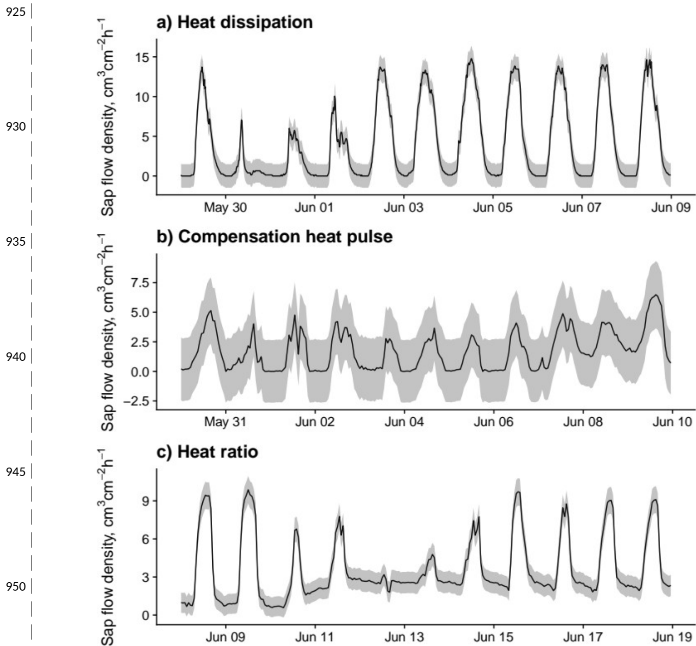
Figure B2. Sub-daily time series of sap flow and methodological uncertainty estimations (one standard error) according to the model in Fig. B1 for 10-day periods in trees measured with (a) heat dissipation, (b) compensation heat pulse and (c) heat ratio sensors. Data for (a) from a Pinus sylvestris tree in dataset ESP VAL SOR; data (b) from a Pinus sylvestris tree in GBR DEV CON; data for (c) from an Eucalyptus victrix in AUS KAR.
