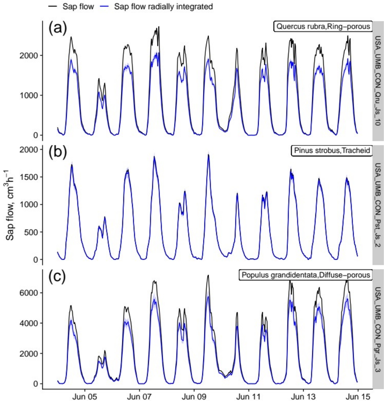
965 | Figure B4. Effects of a generic radial integration on sap flow data originally supplied without any radial integration procedure. Radial integration and uncertainty estimation (blue bands show the 68% prediction interval based on 100 bootstrap samples) were applied using the wood type-specific radial profiles provided in Berdanier et al. (2016), for a ring-porous species (a) a tracheid-bearing species (b) and a diffuse-porous species (c), all belonging to the USA_UMB_CON dataset.
