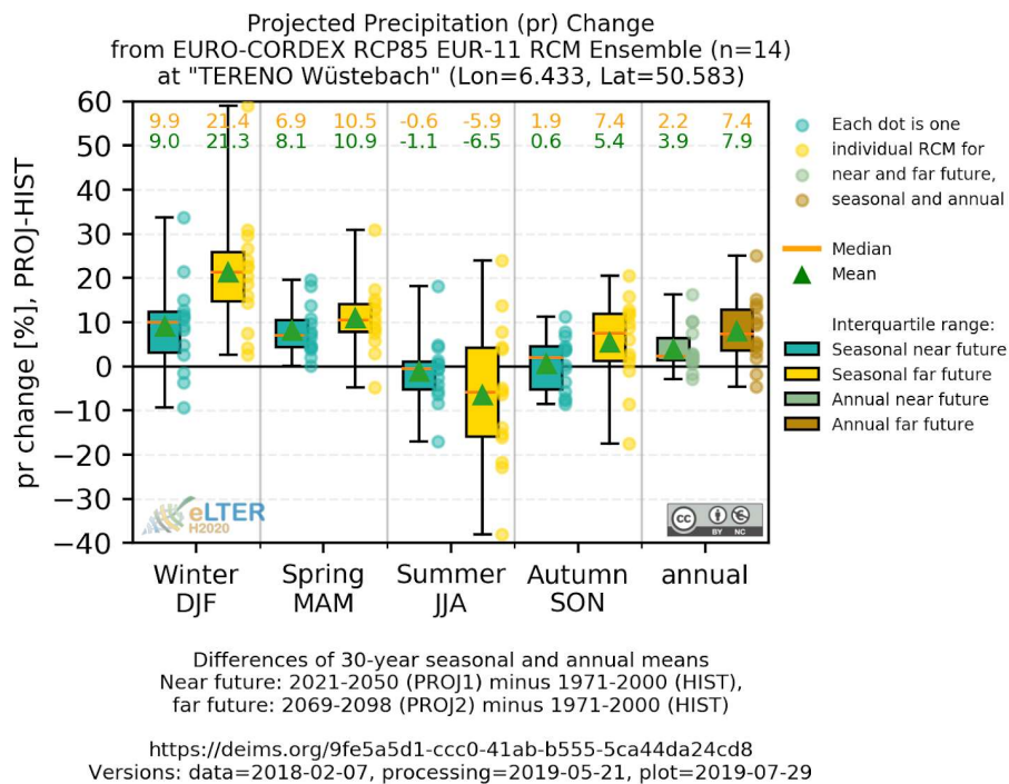
Figure 3 Example eLTER EURO-CORDEX climate scenario data visualisation for one of the TERENO sites in Western Germany:
