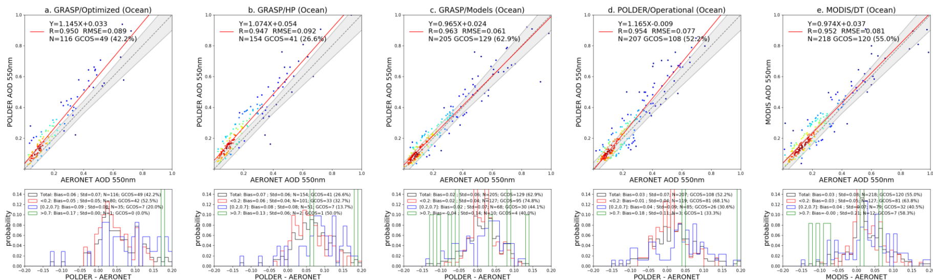
Figure 9: Validation of PARASOL/GRASP, PARASOL/Operational and MODIS/DT AOD at 550 nm over ocean in 2008. (a) GRASP/Optimized; (b) GRASP/HP; (c) GRASP/Models; (d) Operational; (e) DT. The gray dashed line and the red solid line are the 1:1 reference line and the linear regression line. The gray envelope indicates GCOS requirement: max (0.04 or 0.1AOD). The probability density functions of differences (Satellite-AERONET) are present in the lower panel. The black, red, blue and green solid lines indicate all AOD conditions: any AOD, AOD<0.2, 0.2≤AOD≤0.7 and AOD>0.7 respectively.
