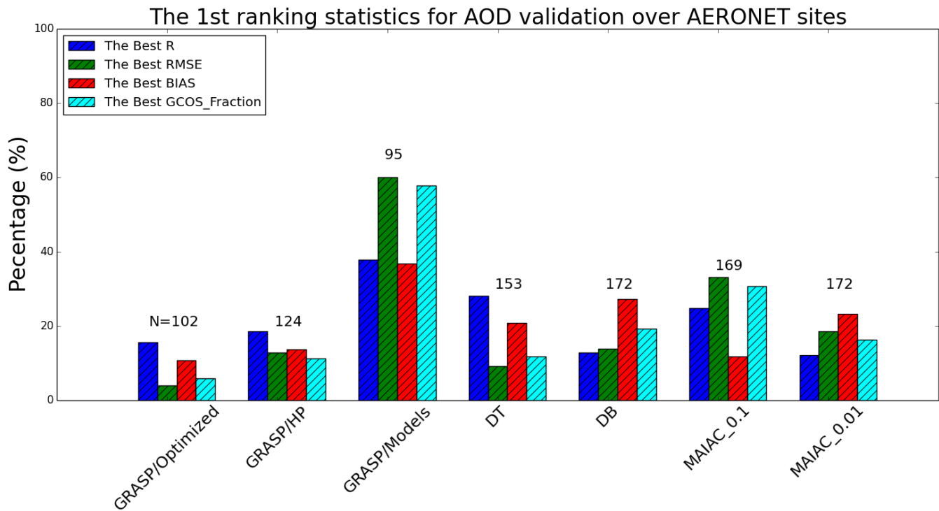
Figure 17: Percentage of the AERONET sites where each product shows the best statistical metric (R, RMSE, BIAS and GCOS Fraction) between 7 PARASOL/GRASP and MODIS AOD products. The number on top of each product is the number of sites where this product has sufficient matchup points for the comparison.
