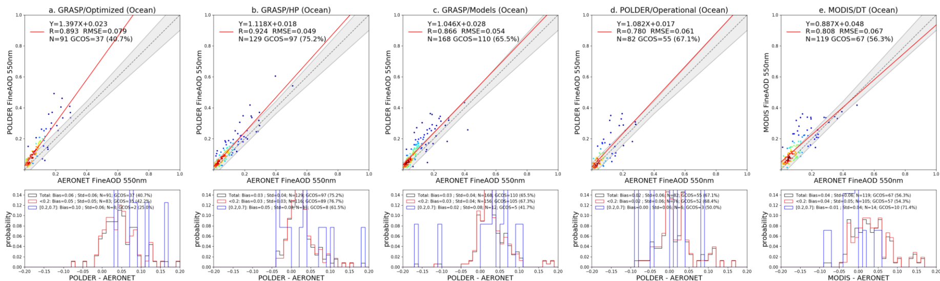
1870 Figure 14: Validation of PARASOL/GRASP (a. GRASP/Optimized; b. GRASP/HP and c. GRASP/Models), (d) PARASOL/Operational and (e) MODIS/DT fine mode AOD at 550 nm over ocean in 2008. The gray envelope indicates GCOS requirement applied for AODF: max (0.04 or 0.1AODF). The probability density functions of differences (Satellite-AERONET) are present in the lower panel. The black, red, blue and green solid lines indicate all AODF conditions: any AODF, AODF < 0.2 , 0.2 \leq AODF \leq 0.7 and AODF > 0.7 respectively.
