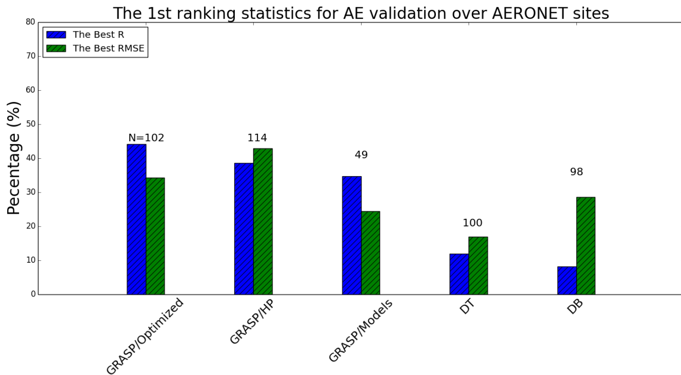
Figure 19: Percentage of the AERONET sites where each product shows the best statistical metric (R and RMSE) between 5 PARASOL/GRASP and MODIS AE products. The number on top of each product is the number of sites where this product has sufficient matchup points for the comparison.
