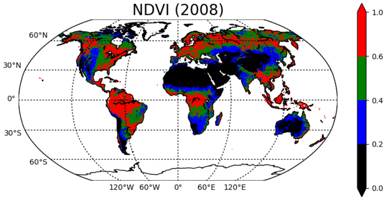
1850 Figure 10: Spatial distribution of annual mean NDVI for 2008 from GRASP/Models L3 products.
