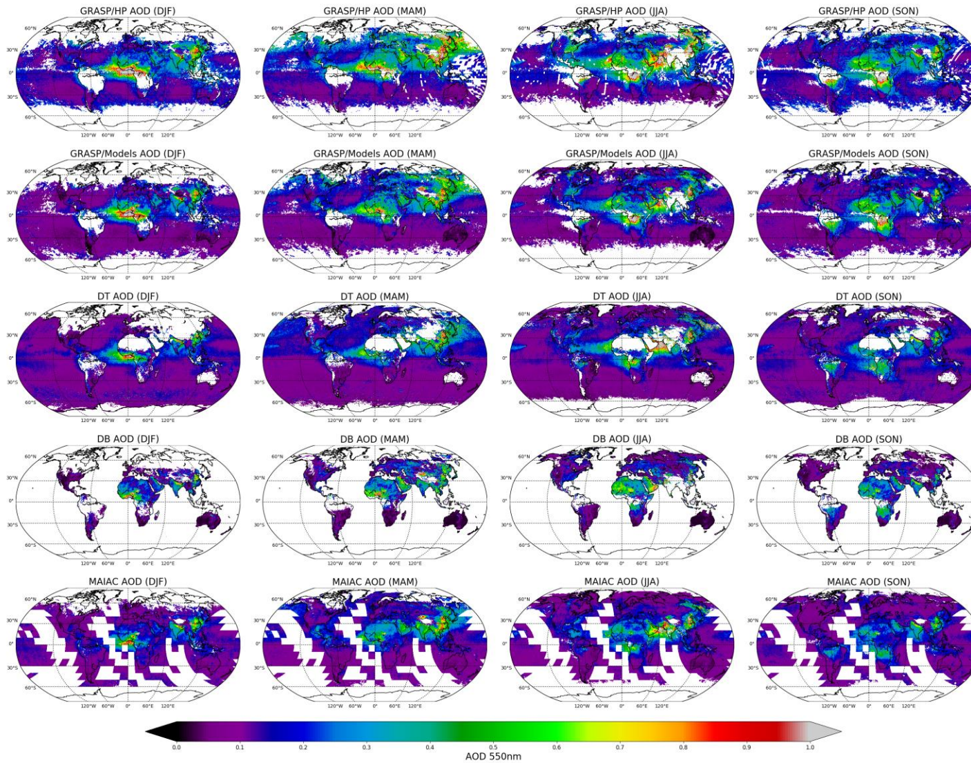
Figure 21: Spatial distribution of 0.1^\circ \times 0.1^\circ seasonal AOD (550 nm) from PARASOL (GRASP/HP and GRASP/Models) and MODIS (DT, DB, and MAIAC) products. DJF – December / January / February; MAM – March / April / May; JJA – June / July / August; SON – September / October / November.
