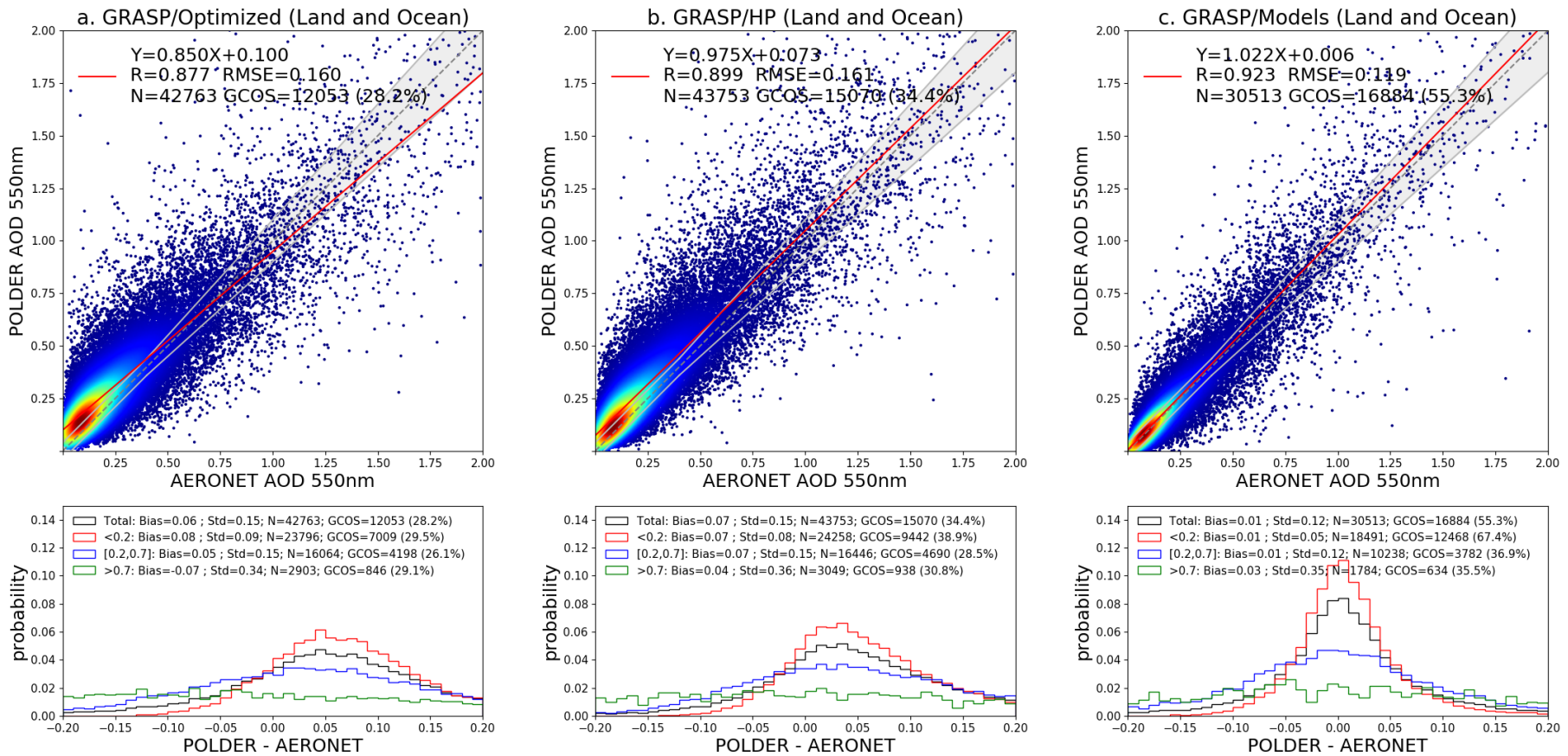
Figure 2: Evaluation of three archives PARASOL/GRASP AOD at 550 nm against AERONET, (a) GRASP/Optimized; (b) GRASP/HP; (c) GRASP/Models. The gray dashed line and the red solid line are the 1:1 reference line and the linear regression line. The gray envelope indicates GCOS requirement: max (0.04 or 0.1AOD). The probability density functions of differences (POLDER-AERONET) are present in the lower panel. The black, red, blue and green solid lines indicate all AOD conditions: any AOD, AOD<0.2, 0.2≤AOD≤0.7 and AOD>0.7 respectively.
