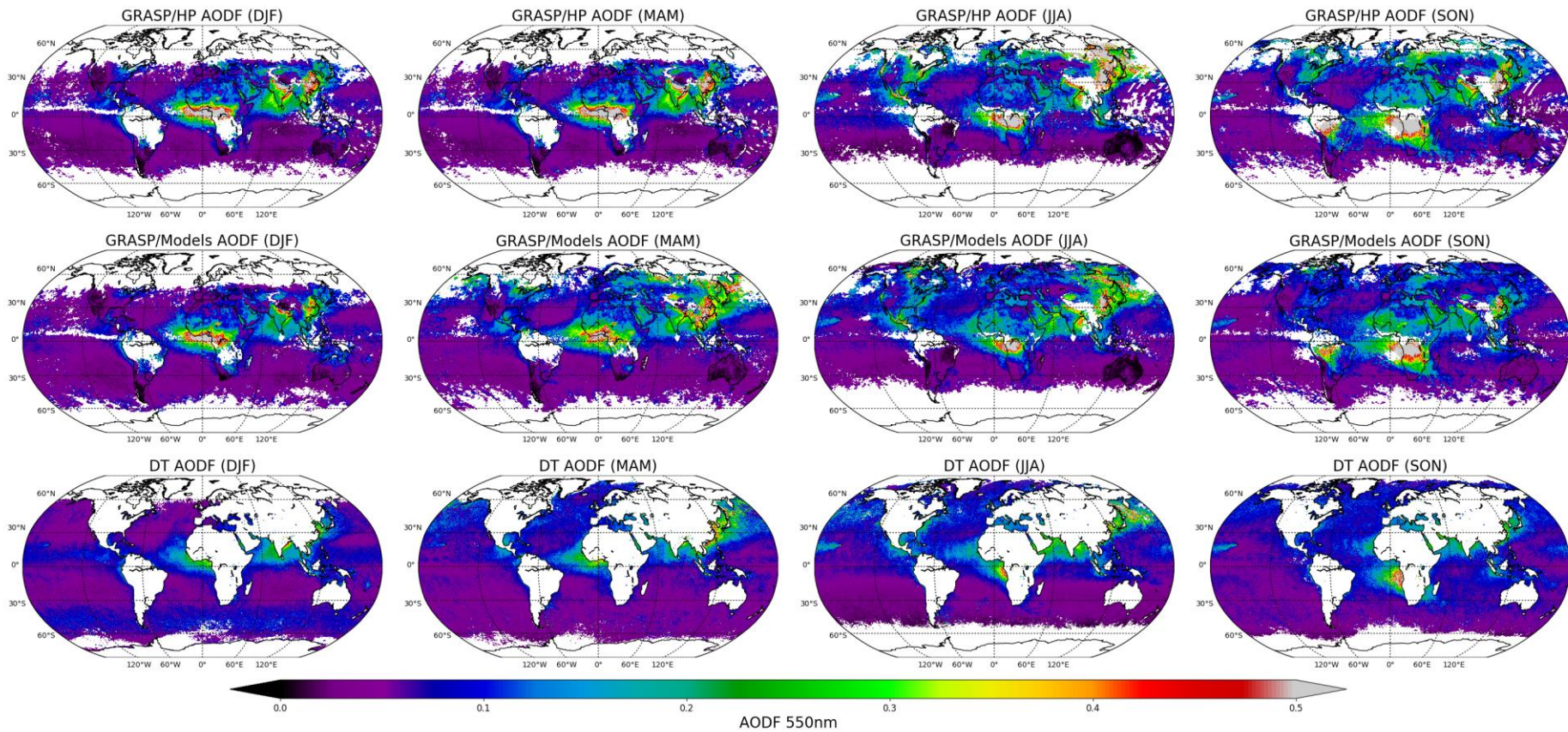
1920 Figure 25: Spatial distribution of 0.1^\circ \times 0.1^\circ seasonal AODF (550 nm) from PARASOL (GRASP/HP and GRASP/Models) and MODIS (DT) products.
