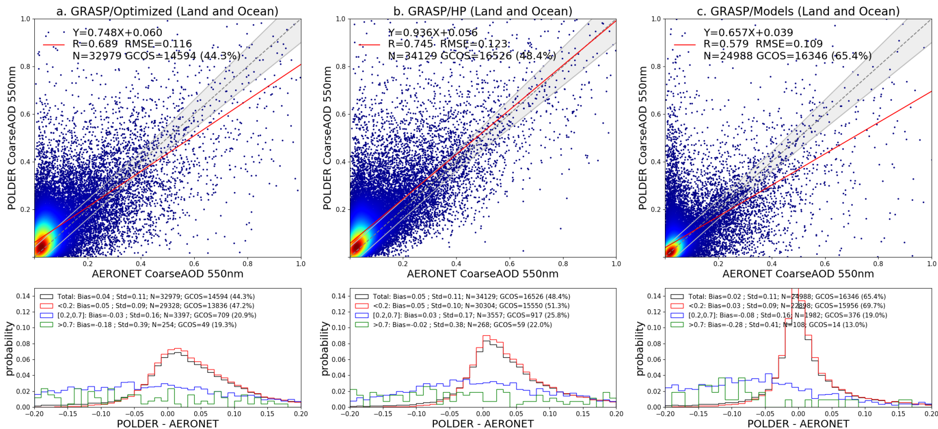
1825 Figure 5: The same as Figure 4, but for AODC at 550 nm.
