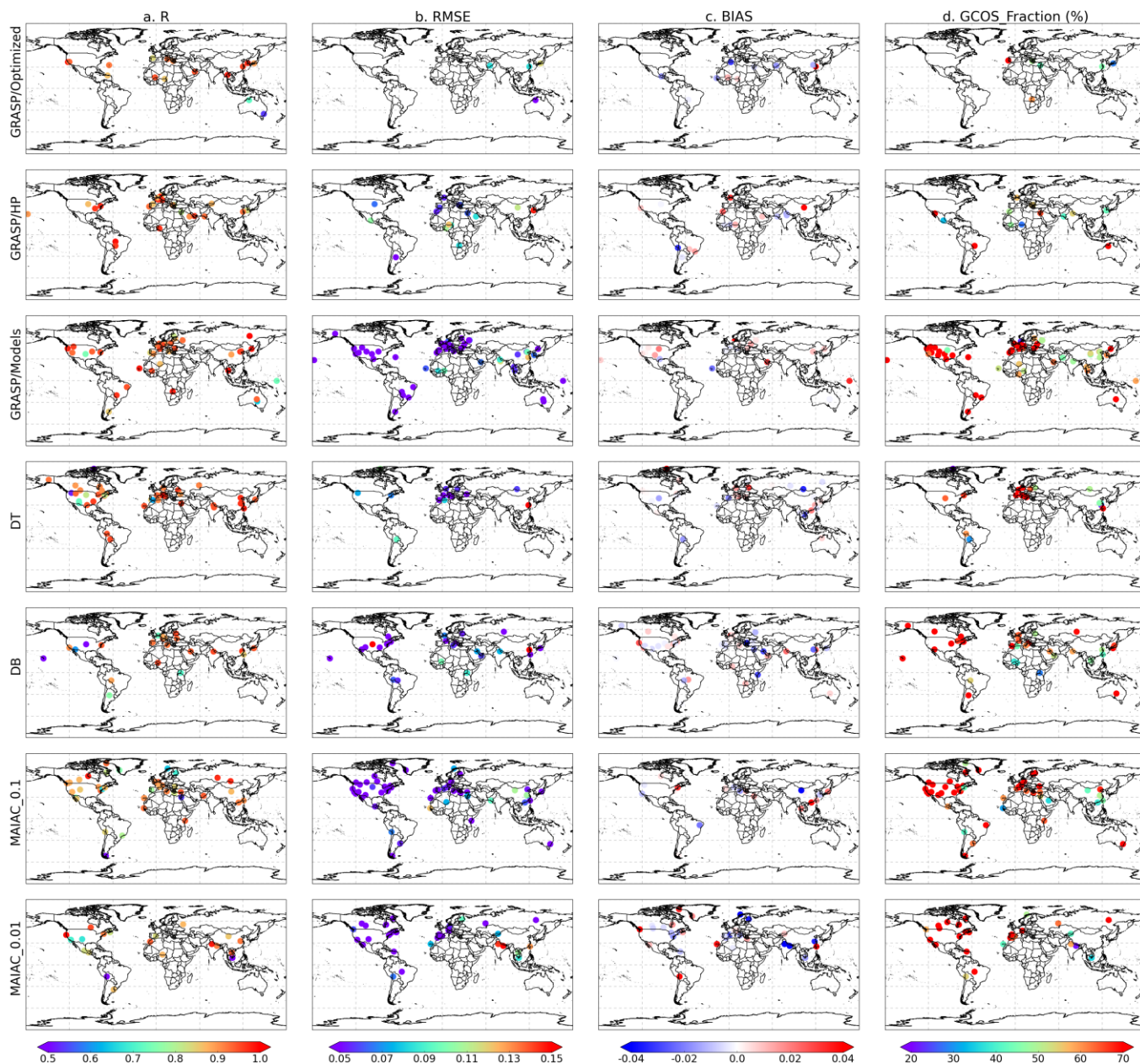
Figure 18: Maps showing statistical metrics (a) R; (b) RMSE; (c) BIAS; (d) GCOS Fraction (%) for 1895 the best performed AOD products (1 st ranking statistics among 7 PARASOL/GRASP and MODIS products) over each AERONET site. Note that only the 1 st ranking statistics over each site are present in the maps.
