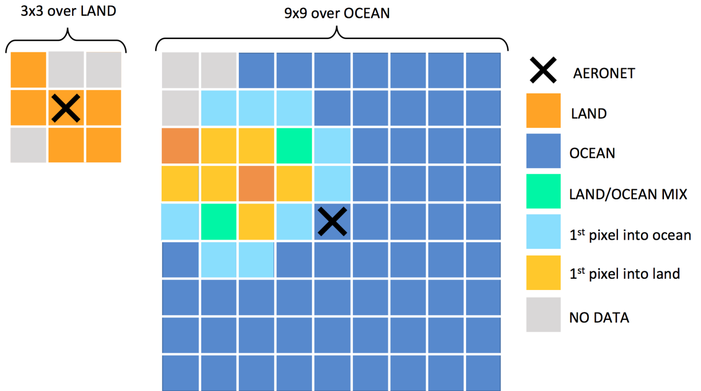
Figure 1: Schematic diagram for satellite data selection over (left) land and (right) ocean.
