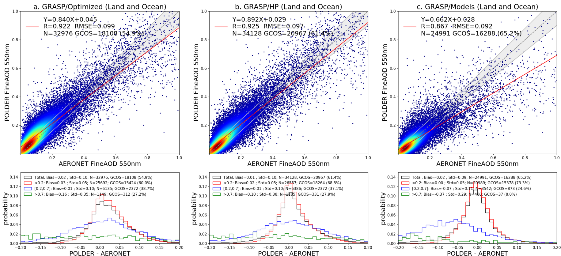
Figure 4: Evaluation of all archive PARASOL/GRASP AODF at 550 nm with AERONET SDA AODF, (a) GRASP/Optimized; (b) GRASP/HP; (c) GRASP/Models. The gray dashed line and the red solid line are the 1:1 reference line and the linear regression line. The gray envelope indicates GCOS requirement applied for AODF: max (0.04 or 0.1AODF). The probability density functions of differences (POLDER-AERONET) are present in the lower panel. The black, red, blue and green solid lines indicate all AODF conditions: any AODF, AODF < 0.2 , 0.2 \le AODF \le 0.7 and AODF > 0.7 respectively.
