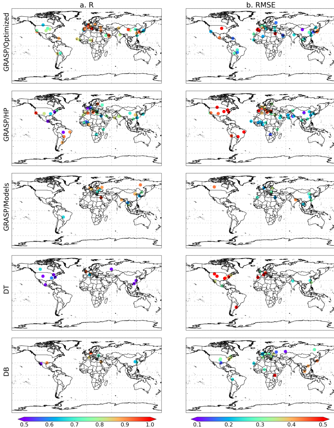
Figure 20: Maps showing statistical metrics (a) R; (b) RMSE; for the best performed AE products (1 st ranking statistics among 5 PARASOL/GRASP and MODIS products) over each AERONET site.
