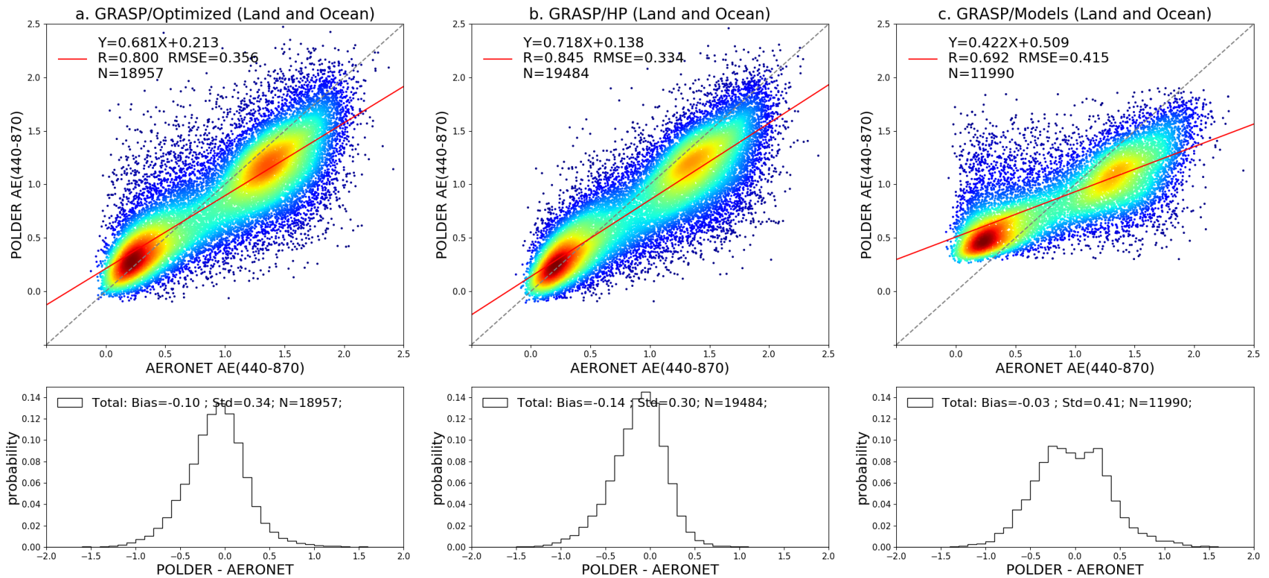
1815 Figure 3: Evaluation of all archive PARASOL/GRASP AE (440/870) against AERONET, (a) GRASP/Optimized; (b) GRASP/HP; (c) GRASP/Models. The gray dashed line and the red solid line are the 1:1 reference line and the linear regression line. The probability density functions of differences (POLDER-AERONET) are present in the lower panel.
