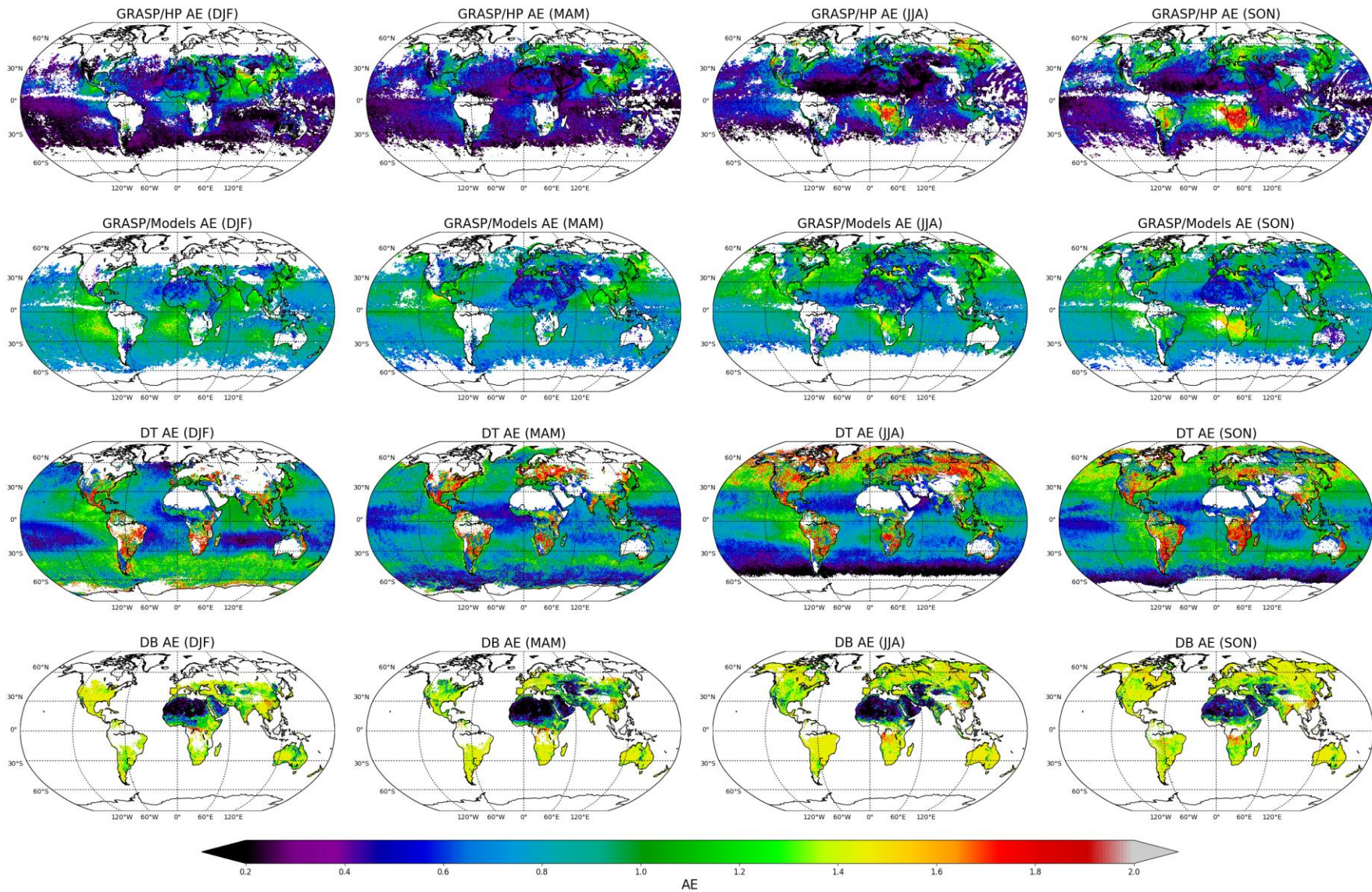
1915 Figure 23: Spatial distribution of 0.1^\circ \times 0.1^\circ seasonal AE from PARASOL (GRASP/HP and GRASP/Models) and MODIS (DT and DB) products.
