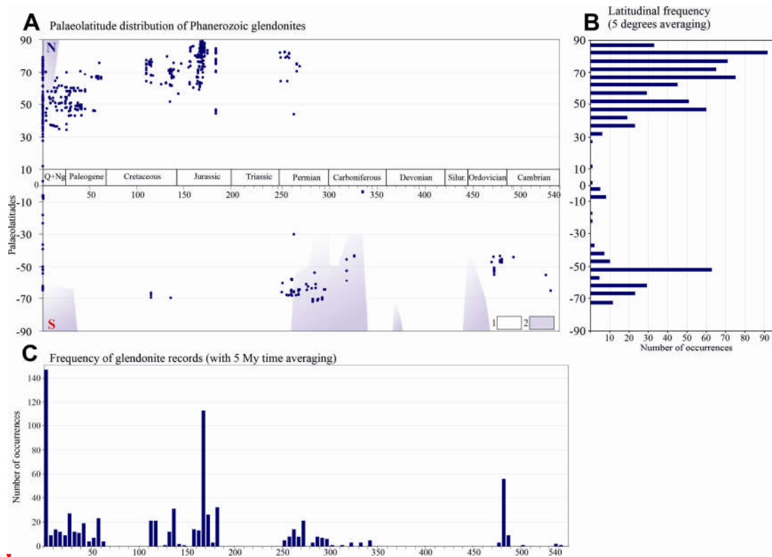
Fig. 5. Palaeolatitudinal distribution of glendonite and ikaite records through time. A – palaeolatitudinal occurrence; 1 – non-glacial intervals, 2 - glaciations (after Frakes et al., 2005); B – latitudinal frequency of glendonite occurrences (with 5 degrees averaging); C – frequency of glendonite occurrence through time (with 5 Ma averaging).
