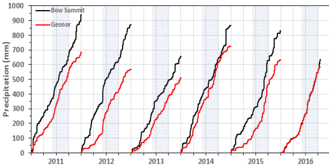
5 Figure 7: Annual cumulative precipitation at Bow Summit and Peyto Main, 2011 to September 2016, with highlighting of main summer rainfall months.
