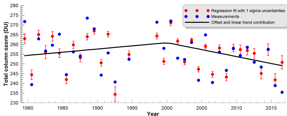
Figure 18. The July mean total column ozone at 19.5^{\circ} S, 164.375^{\circ} W (blue dots) together with the regression model values (red dots) and their 1\sigma uncertainties, and the contribution to the regression model from the offset and two trend basis functions.
