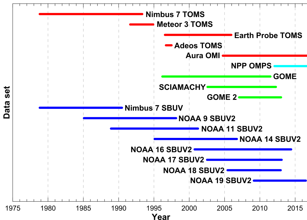
Figure 1. A graphical representation of the different satellite-based data sets used in this study and their periods of coverage.
