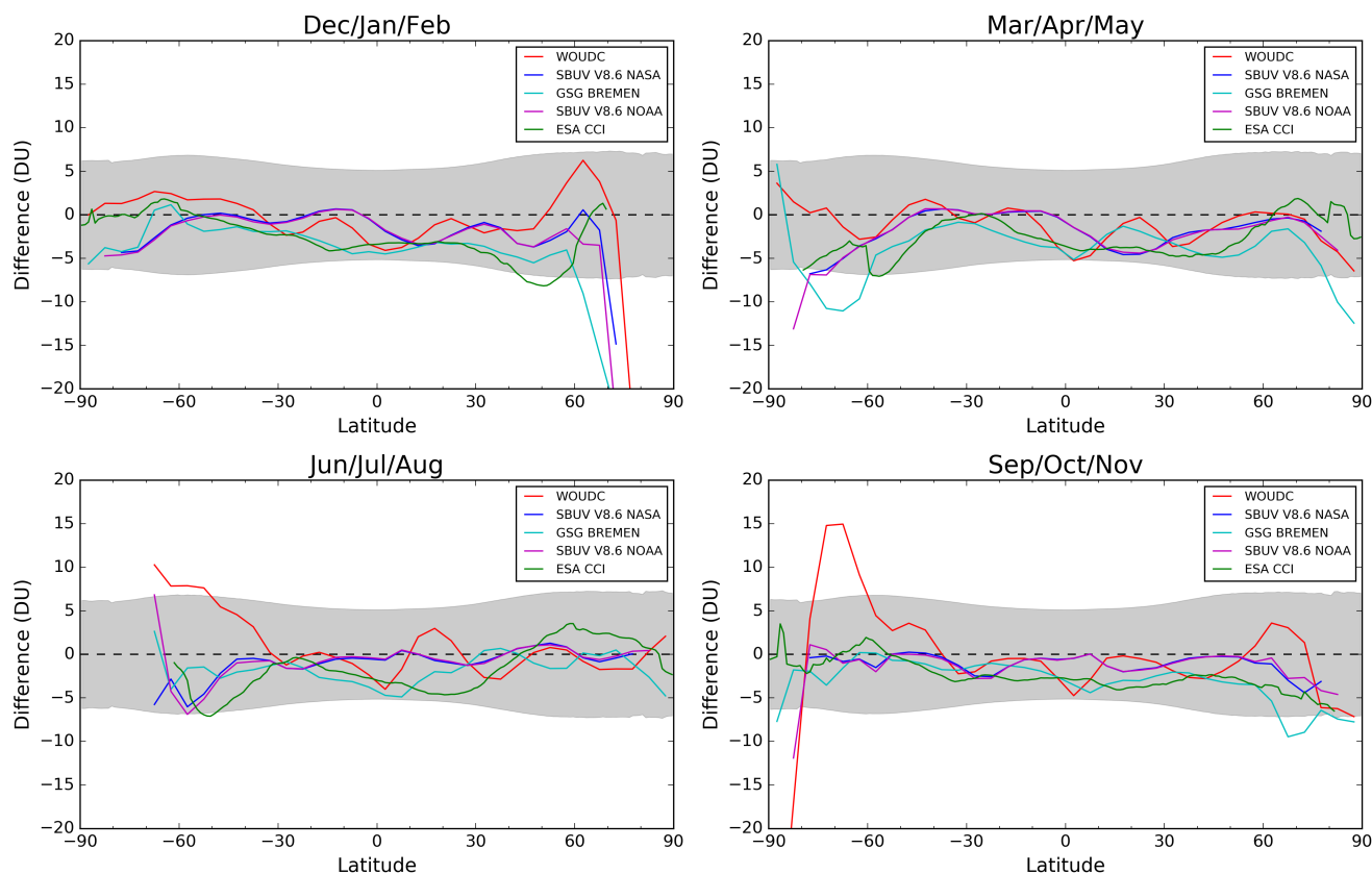
Figure 7. TCO differences (NIWA-BS TCO minus validation database) as a function of latitude plotted as seasonal means over the entire period of data available. The 1\sigma uncertainty range in the NIWA-BS TCO is shown in grey.
