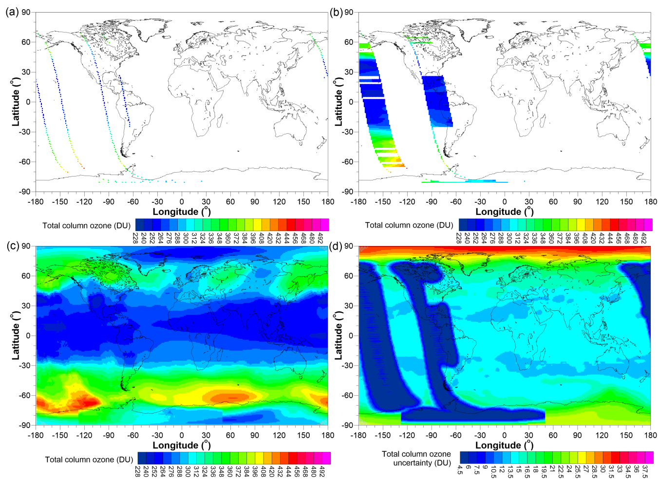
Figure 15. (a) The original unfilled TCO field on 31 October 1978, (b) the conservatively filled field, (c) the final filled field, and (d) the uncertainties on the final filled field.
