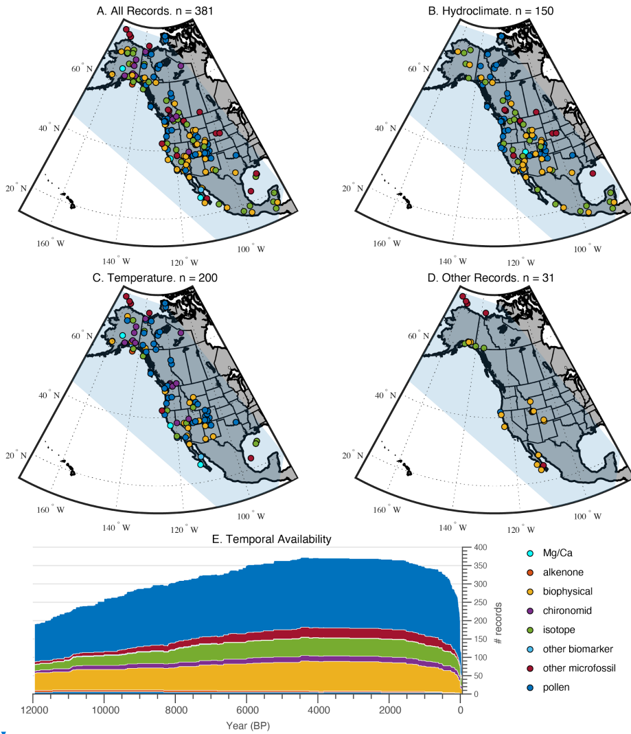
Figure 1. Spatiotemporal distribution of the western North American Holocene paleoclimate database. A) The database includes 381 proxy records from a variety of archive and proxy types. Records include those in calibrated climate units (e.g. °C) and records in their native proxy units (e.g. \delta^{18}O ). B) Distribution of records sensitive to hydroclimate including precipitation, flood frequency, and P-E (n = 150). C) Spatial distribution of the subset of records sensitive to temperature (n = 200), and D) the spatial distribution of
