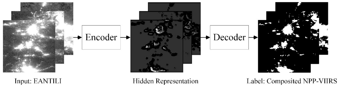
Figure 3: The framework of the auto-encoder model
