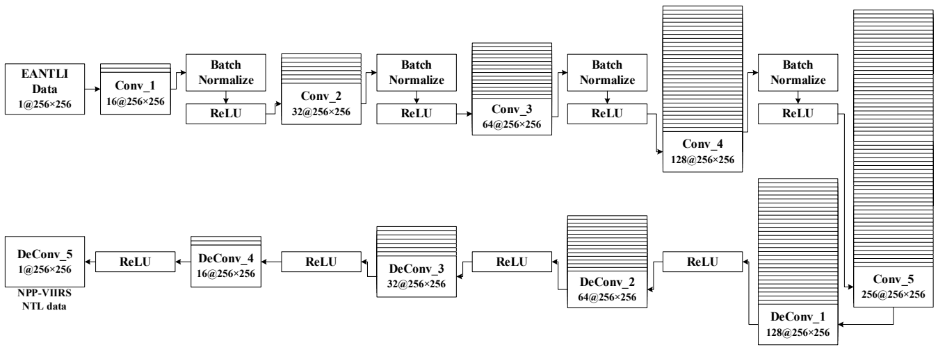
605 Figure 4: The overall architecture of our proposed auto-encoder with CNN
