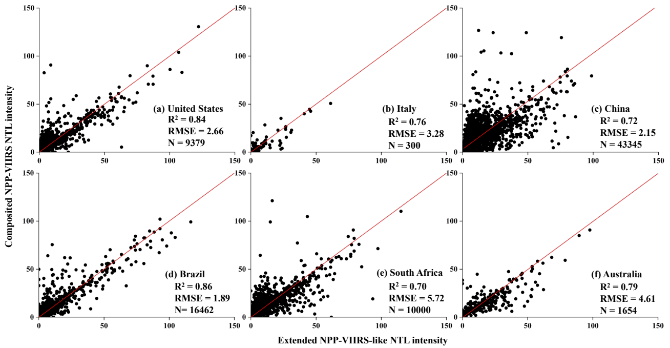
Figure 6: The comparison between composed NPP-VIIRS NTL data and extended NPP-VIIRS-like NTL data in 2012 (unit: nano-Wcm 2 sr -1 ) at the pixel level in six countries. Solid line denotes the 1:1 line and N is the number of sample points (cities).
