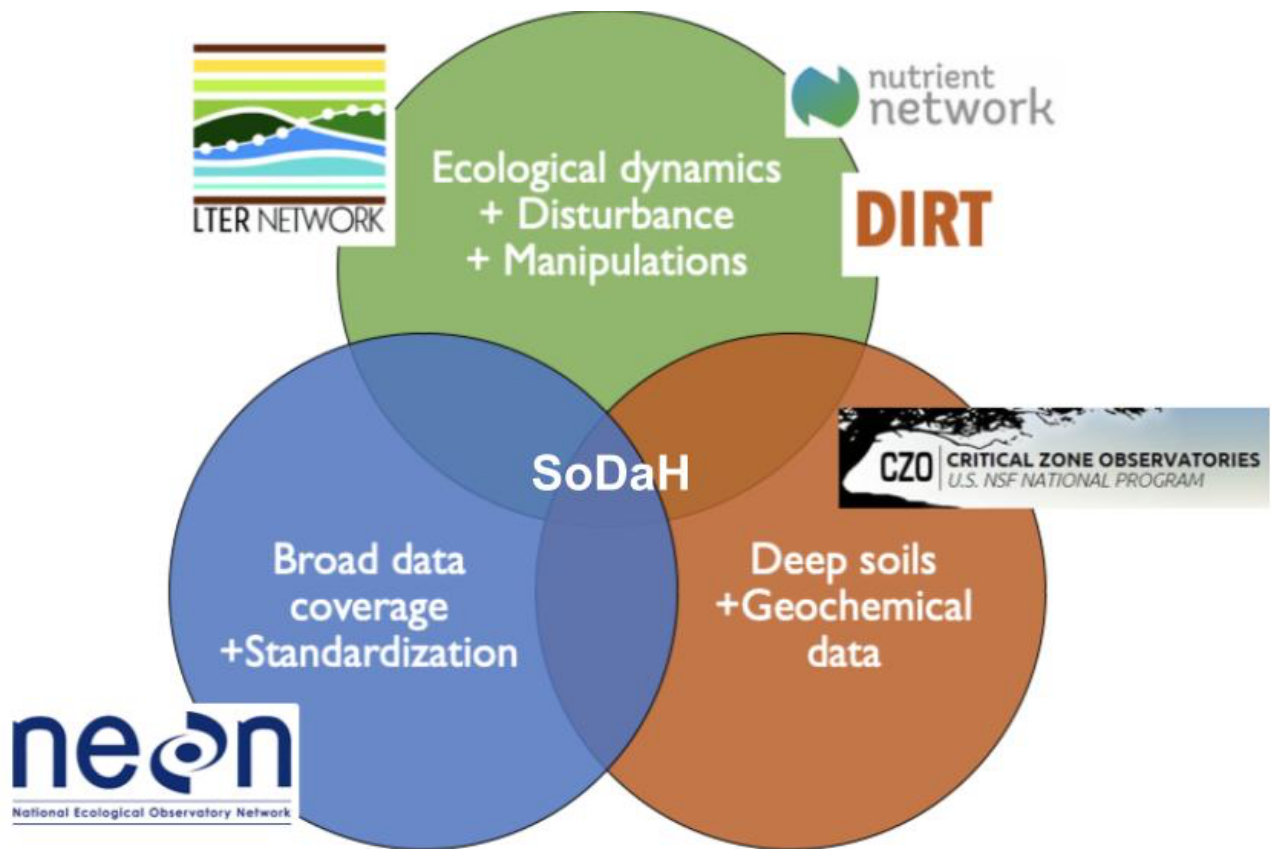
495 Figure 1: Conceptual diagram that summarizes the strengths and research foci of different experimental networks contributing to SoDaH, modified from Weintraub et al. 2019.
