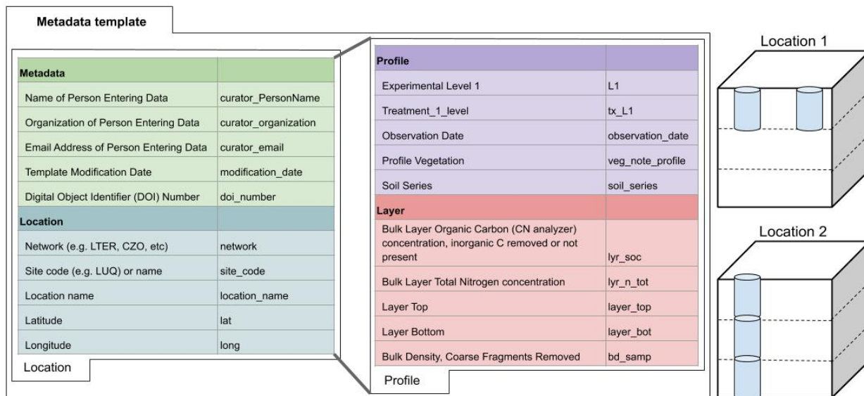
500 Figure 2: Diagram showing hierarchical relationship between data fields in the Soils Data Harmonization (SoDaH) database, which includes metadata, location, profile and layer fields. Each data field lists a short description of some of the variables used along with the variable name used in the database. To facilitate data contributions these data fields were grouped into Location and Profile tabs on the metadata template used by data contributors. The right side of the figure illustrates data from two 505 hypothetical locations (e.g., a LTER and CZO site, respectively) where Location 1 includes data from two profiles that each have information from one layer. Location 2 provides data from one profile that has information from three layers. Any location may provide data from multiple profiles or layers. With data harmonization data for each profile and layer will inherit metadata and location data that are provided in the location tab.
