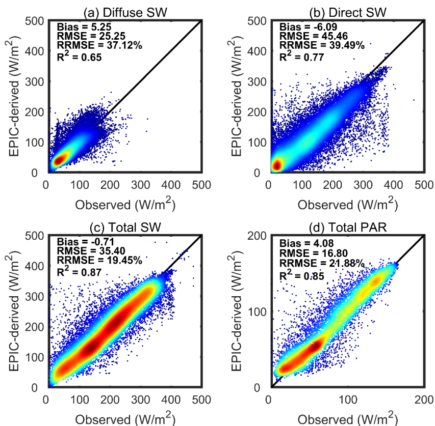
180 Figure 3. Evaluation of EPIC-based daily SW/PAR estimates against ground-based observations.
