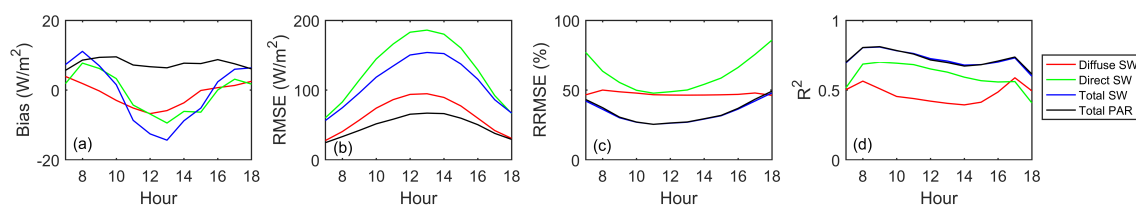
Figure 5. Evaluation of EPIC-based hourly SW/PAR estimates at different local hours from 7:00 to 18:00.
