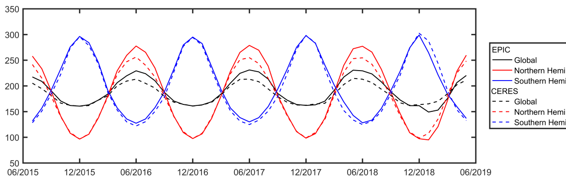
Figure 10. Temporal variations of EPIC- and CERES-based monthly total SW for the land surface of global, northern- and southern-hemispheres.
