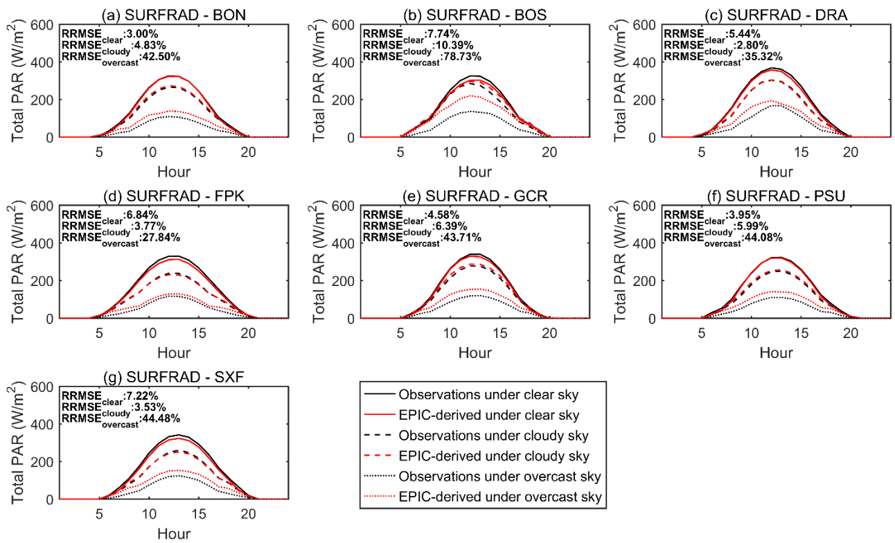
Fig. S3. Averaged diurnal variations of EPIC- and ground-based total PAR flux ( W/m^2 ) under different sky conditions at 7 SURFRAD sites.
