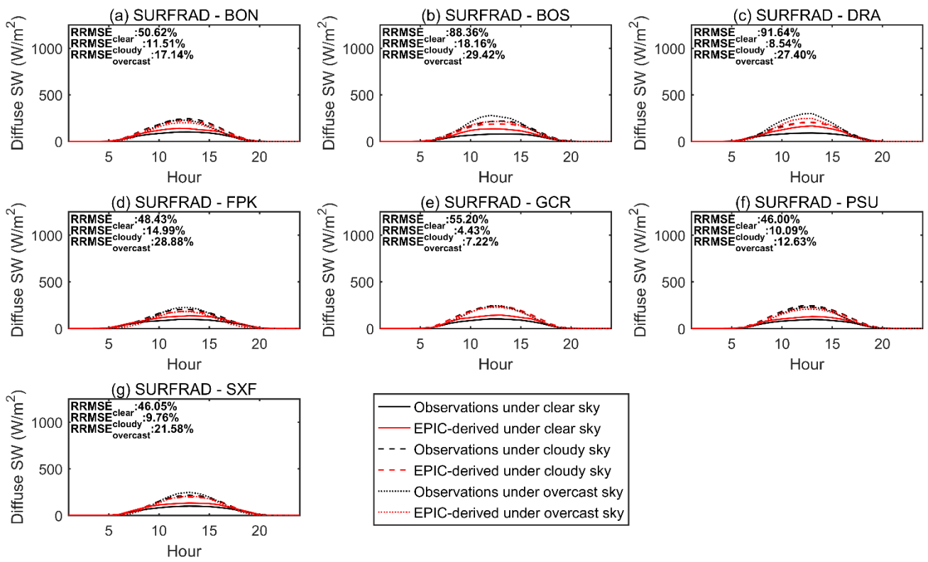
Fig. S1. Averaged diurnal variations of EPIC- and ground-based diffuse SW radiation flux ( W/m^2 ) under different sky conditions at 7 SURFRAD sites.
