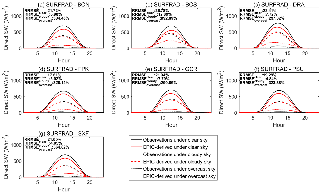
Fig. S2. Averaged diurnal variations of EPIC- and ground-based direct SW radiation flux ( \text{W/m}^2 ) under different sky conditions at 7 SURFRAD sites.
