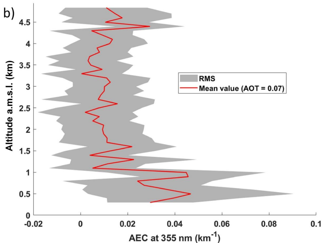
Figure 7. a) Calibration coefficient R_c of the volume depolarization ratio (VDR) derived from flight altitude above 4.5 km on 25 January 2020 (flight F04). b) Vertical profile of the average aerosol extinction coefficient (AEC) with its root mean square variability (RMS) for the flight range on 25 January 2020. It corresponds to the Level-3 aerosol product. The aerosol optical thickness (AOT) is also reported.
