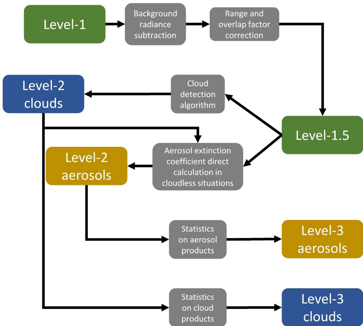
Figure 4. Lidar data processing diagram starting from raw data (1) and calibrated data (Level-1.5) to products (Level-2 and Level-3). The grey cells summarize the actions to be implemented for the data processing. The green color refers to data level in the pre-processing phase. Level-2 and Level-3 are subdivided in clouds (blue) or aerosols (orange) products.
