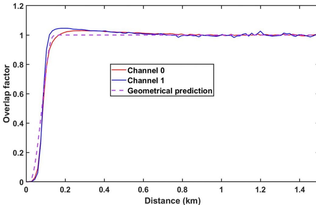
15 Figure 8. Overlap factor of ALiAS on board ATR-42 during EUREC 4 A.
