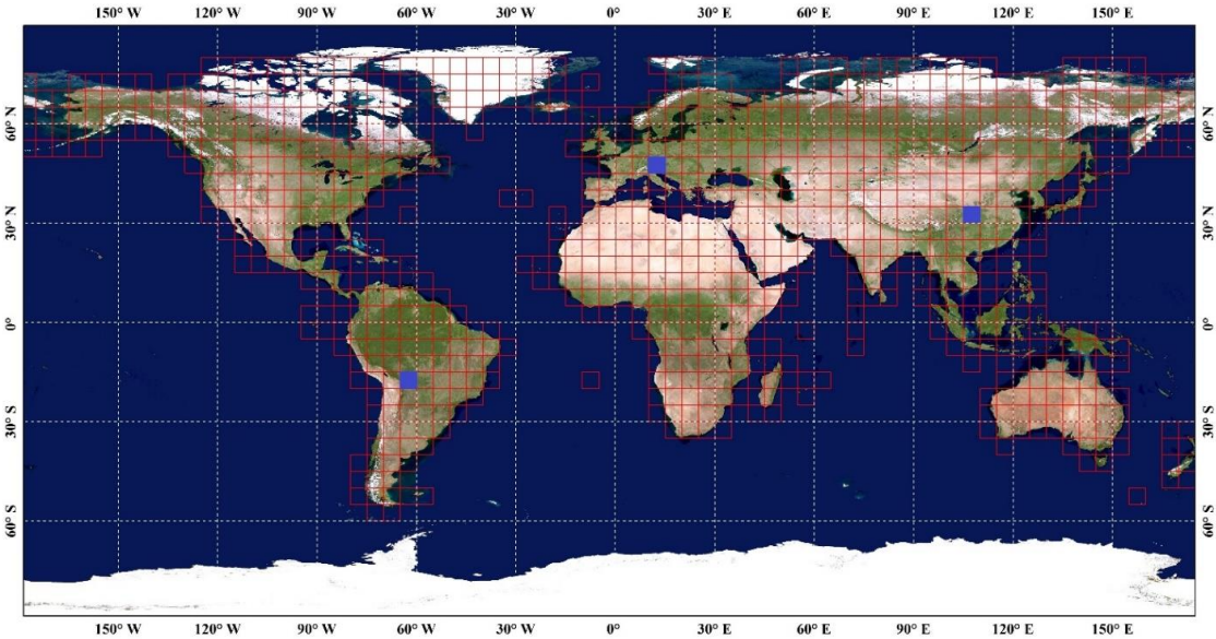
Figure 4. Overview of the 5°x5°geographical tiles used for local adaptive modelling. Three blue rectangular tiles were used for comparing GLC_FCS30 with other land-cover products. The background imagery came from the National Aeronautics and Space Administration ( https://visibleearth.nasa.gov ).
