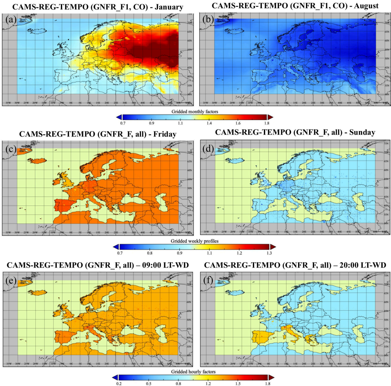
1370 Figure 7: CAMS-REG-TEMPO (0.1x0.05 deg) monthly (a, b), weekly (c, d) and hourly (e, f) scale factor maps. Monthly factors correspond to the meteorological dependent profiles computed for CO exhaust gasoline emissions (GNFR_F1) for January and August (climatology of 2010-2017). Weekly factors are represented for Friday and Sunday. Hourly factors are represented for weekdays (WD) at 09:00 and 20:00 local time (LT). Administrative boundaries are derived from the Micro World Data Bank (MWDB2, 2011).
