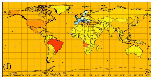
CAMS-GLOB-TEMPO (ind) - August
