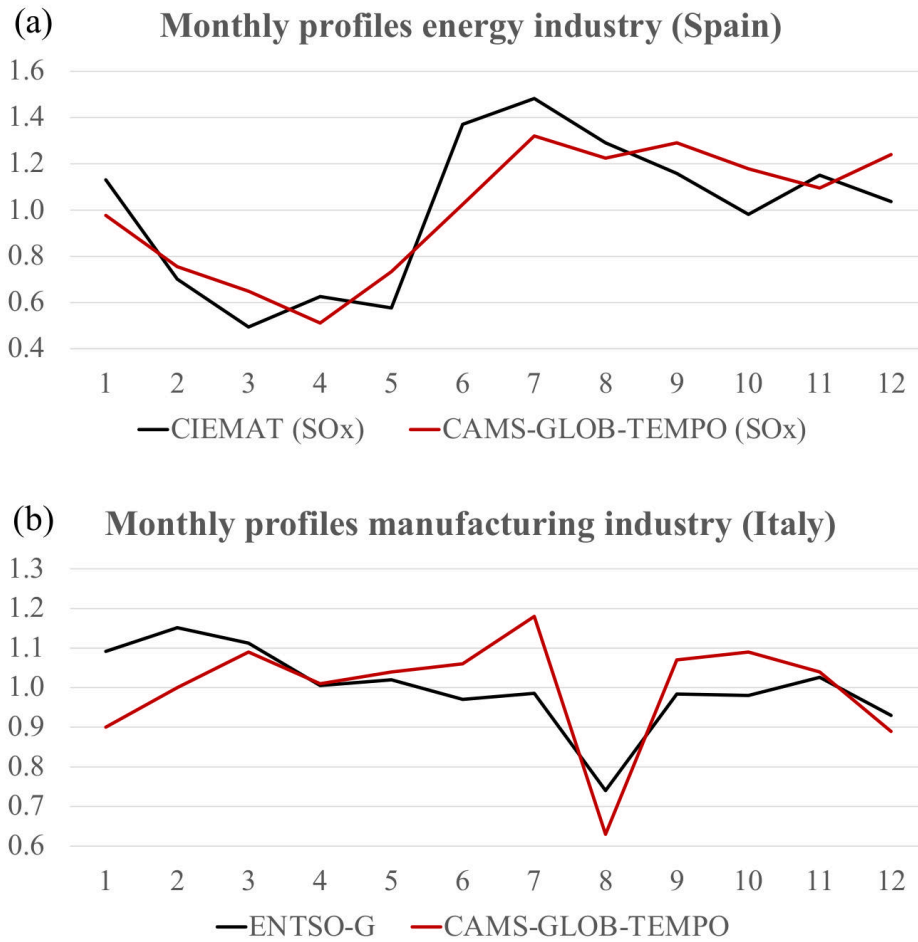
1380 Figure 9: (a) Comparison between monthly temporal factors for SO x energy industry emissions derived from power plant emission measurements (CIEMAT, personal communication) and reported by CAMS-GLOB-TEMPO for Spain. (b) Comparison between monthly temporal factors for manufacturing industry emissions derived from real-world measurements of industrial natural gas consumption (ENTSO-G, 2020) and reported by CAMS-GLOB-TEMPO for Italy.
