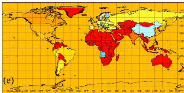
CAMS-GLOB-TEMPO (ind) - January
