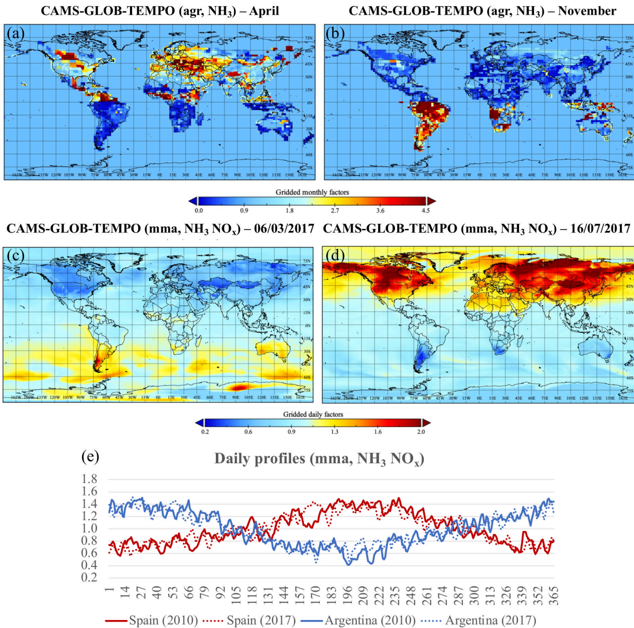
1375 Figure 8: CAMS-GLOB-TEMPO (0.1x0.1 deg) monthly (a, b) and daily (c, d) scale factor maps for agriculture (agr) NH 3 emissions and livestock (mma) NH 3 and NO x emissions for April and November and 2017/03/06 and 2017/07/16, respectively. Daily factors for livestock emissions (mma) obtained over Spain and Argentina for 2010 and 2017 (e). Administrative boundaries are derived from the Micro World Data Bank (MWDB2, 2011).
