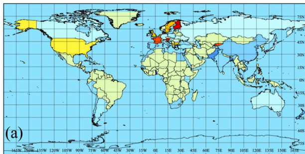
CAMS-GLOB-TEMPO (ene, NMVOC) - January
