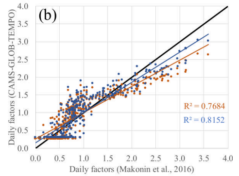
Figure 10: (a) Comparison between daily temporal factors obtained in a location in Vancouver (Canada) for 2013 from real-world measurements of residential natural gas consumption (Makonin et al., 2016) and from the residential/commercial gridded temporal profiles reported by CAMS-GLOB-TEMPO. Two versions of the CAMS-GLOB-TEMPO temporal factors are shown as a function of the base temperature ( T_b ) assumed when applying the Heating Degree Day approach (18 °C in orange and 15.5°C in blue). (b) scatter plot showing the trend lines and R^2 values obtained from the comparison between measurement-based and CAMS-GLOB-TEMPO daily factors.
