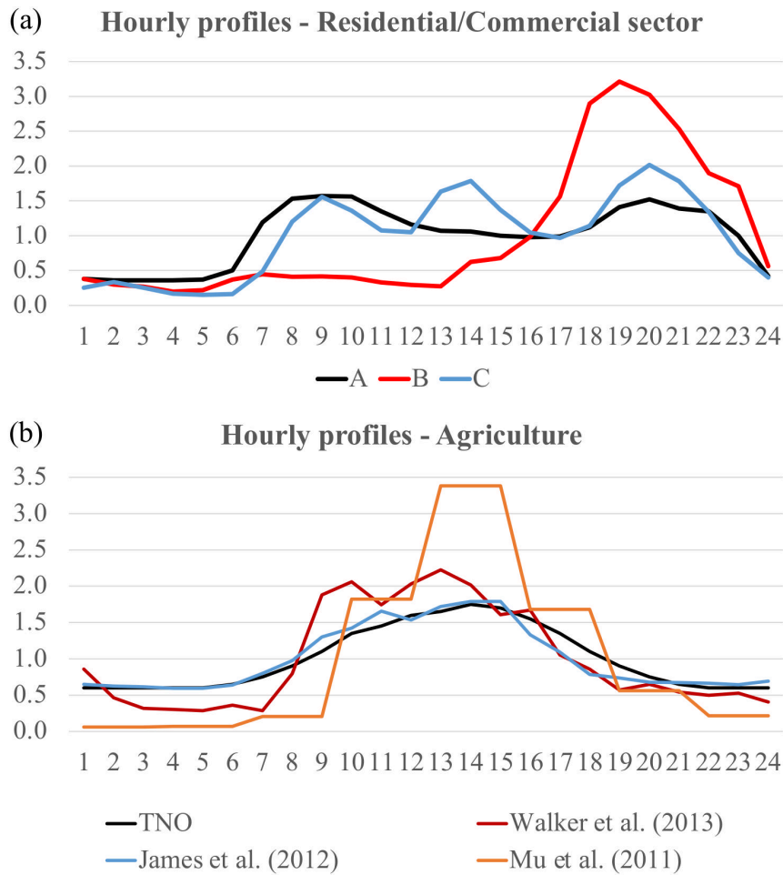
1335 Figure 2: (a) Proposed hourly temporal profiles for the residential/commercial combustion sector where profile A refers to NO x , SO x and CH 4 emissions in urban/rural areas of developed and developing countries, profile B refers to PM 10 , PM 2.5 , CO, CO 2 , NMVOC and NH 3 in urban/rural areas of developed countries, and profile C refers to all pollutants in rural areas of developing countries. (b) Comparison between the hourly temporal profile proposed by TNO for agricultural emissions (Denier van der Gon et al., 2011) and the three measurement-based temporal profiles reported by Walker et al. (2013) derived from NH 3 flux measurements performed in a fertilized corn canopy in North Carolina, James et al. (2012) based on direct NH 3 measurements performed in a mechanically ventilated swine barn, and Mu et al. (2011) derived from active fire satellite observations.
