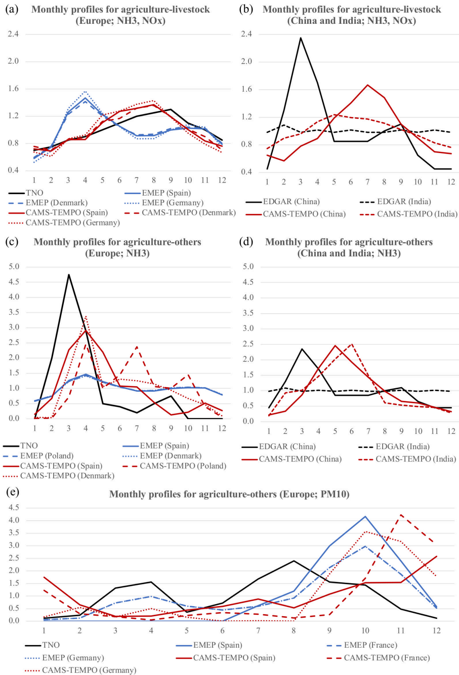
1415 Figure 15: Comparison of monthly profiles for agricultural emissions developed in the present work (CAMS-TEMPO) with profiles from EDGAR, EMEP and TNO for selected countries and categories: NH 3 livestock emissions in Europe (a) and China and India (b), NH 3 other agricultural emissions in Europe (c) and China and India (d), PM 10 other agricultural emissions in Europe (e).
