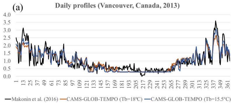
Figure 10: (a) Comparison between daily temporal factors obtained in a location in Vancouver (Canada) for 2013 from real-world measurements of residential natural gas consumption (Makonin et al., 2016) and from the residential/commercial gridded temporal profiles reported by CAMS-GLOB-TEMPO. Two versions of the CAMS-GLOB-TEMPO temporal factors are shown as a function of the base temperature ( T_b ) assumed when applying the Heating Degree Day approach (18 °C in orange and 15.5°C in blue). (b) scatter plot showing the trend lines and R^2 values obtained from the comparison between measurement-based and CAMS-GLOB-TEMPO daily factors.
