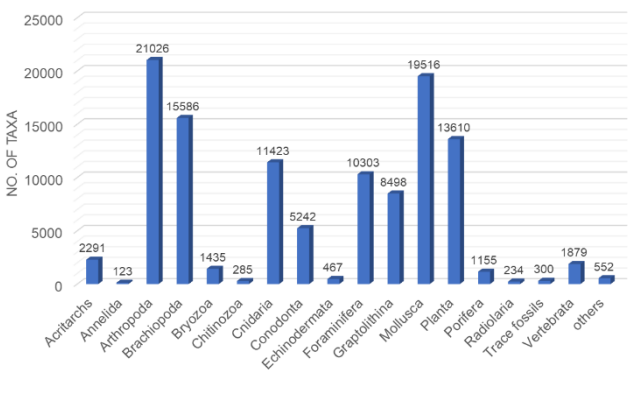
(c) Number of taxa
