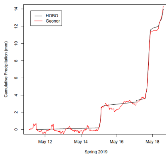
Fig. 1. Comparison between precipitation accumulation at a HOB0 tipping bucket rain gauge and a Geonor weighing gauge at Nipika Mountain Resort, 11-19 May 2019.
