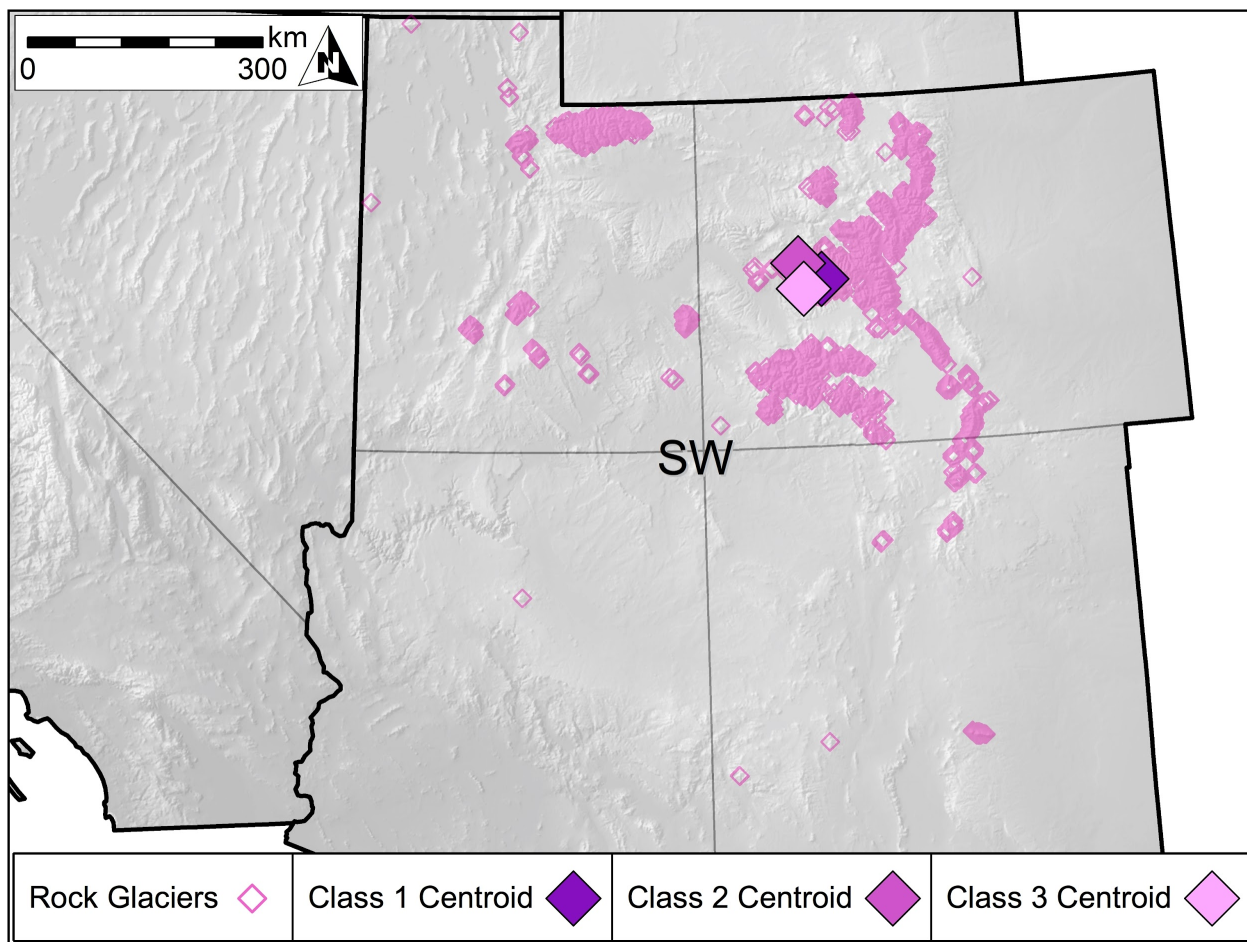
Figure 76: Locations of SW Regionregion rock glacier inventory features ( n = 4870 ), as well as centroids for Class 1 ( n = 3291 ), Class 2 ( n = 1133 ) and Class 3 ( n = 446 ) features. Rock glaciers of the SW Regionregion are largest and most densely concentrated in the Front Range and San Juan Mountains of Colorado and the Uinta Mountains of Utah.
