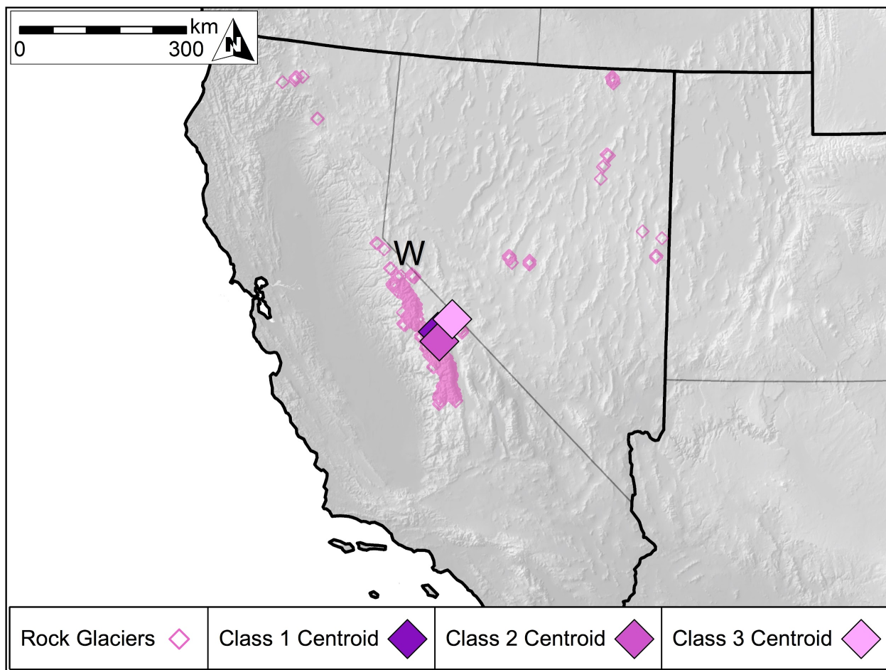
Figure 87: Locations of W Region rock glacier inventory features (n = 817), as well as centroids for Class 1 (n = 552), Class 2 (n = 181) and Class 3 (n = 84) features. Rock glaciers of the W Region are largest and most densely concentrated in the Sierra Nevada of California.
