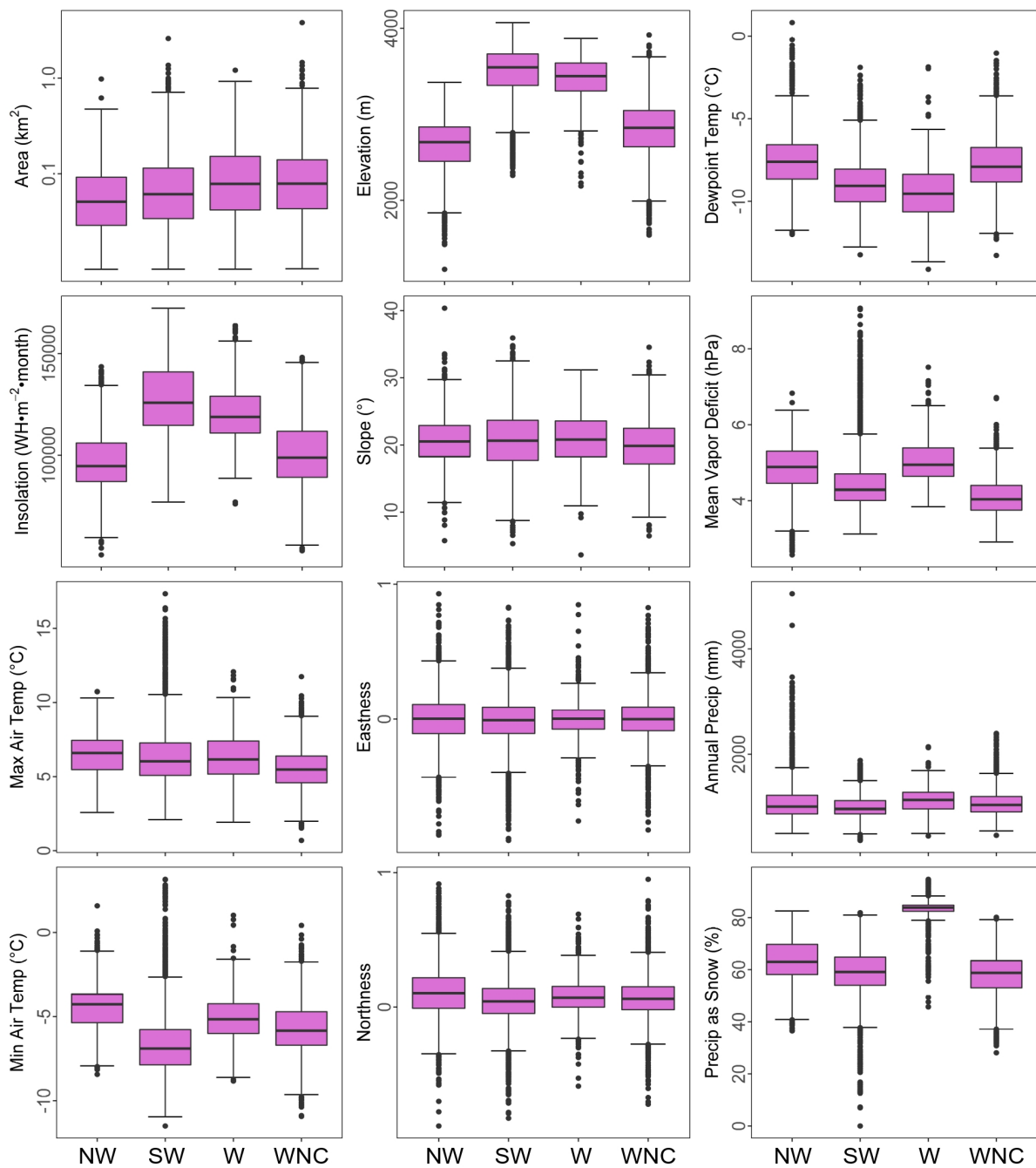
765 | Figure 54: Geographic characteristics of rock glaciers by NOAA Climate Region. Boxplot whiskers represent 1.5 times the interquartile range, outliers beyond those values are shown by solid dots.
