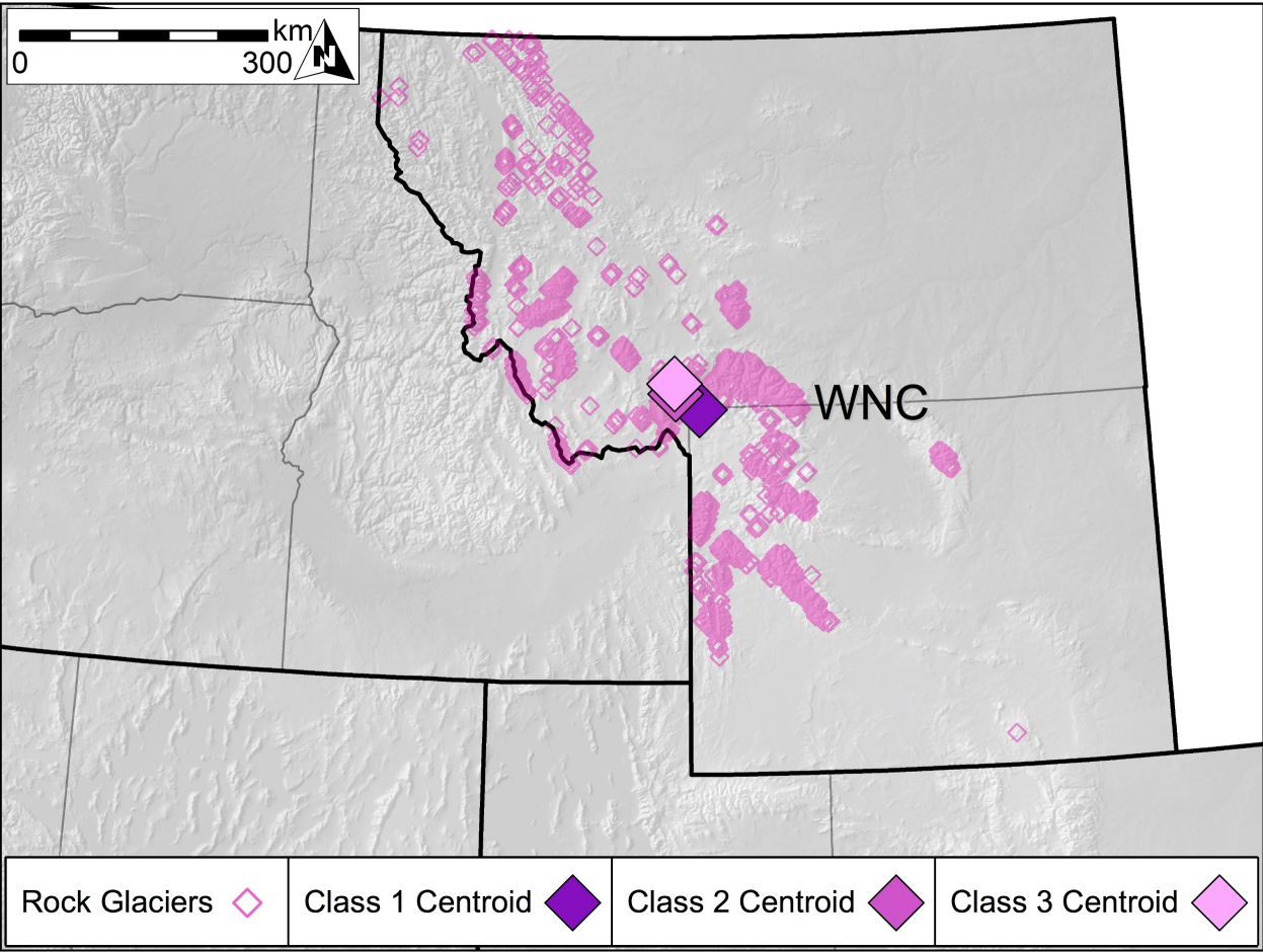
Figure 98: Locations of WNC Regionregion rock glacier inventory features ( n = 26522663 ), as well as centroids for Class 1 ( n = 19064916 ), Class 2 ( n = 589590 ) and Class 3 ( n = 157 ) features. Rock glaciers of the WNC Regionregion are largest and most densely concentrated in the Beartooth Mountains of Montana and the Absaroka Range of Wyoming.
