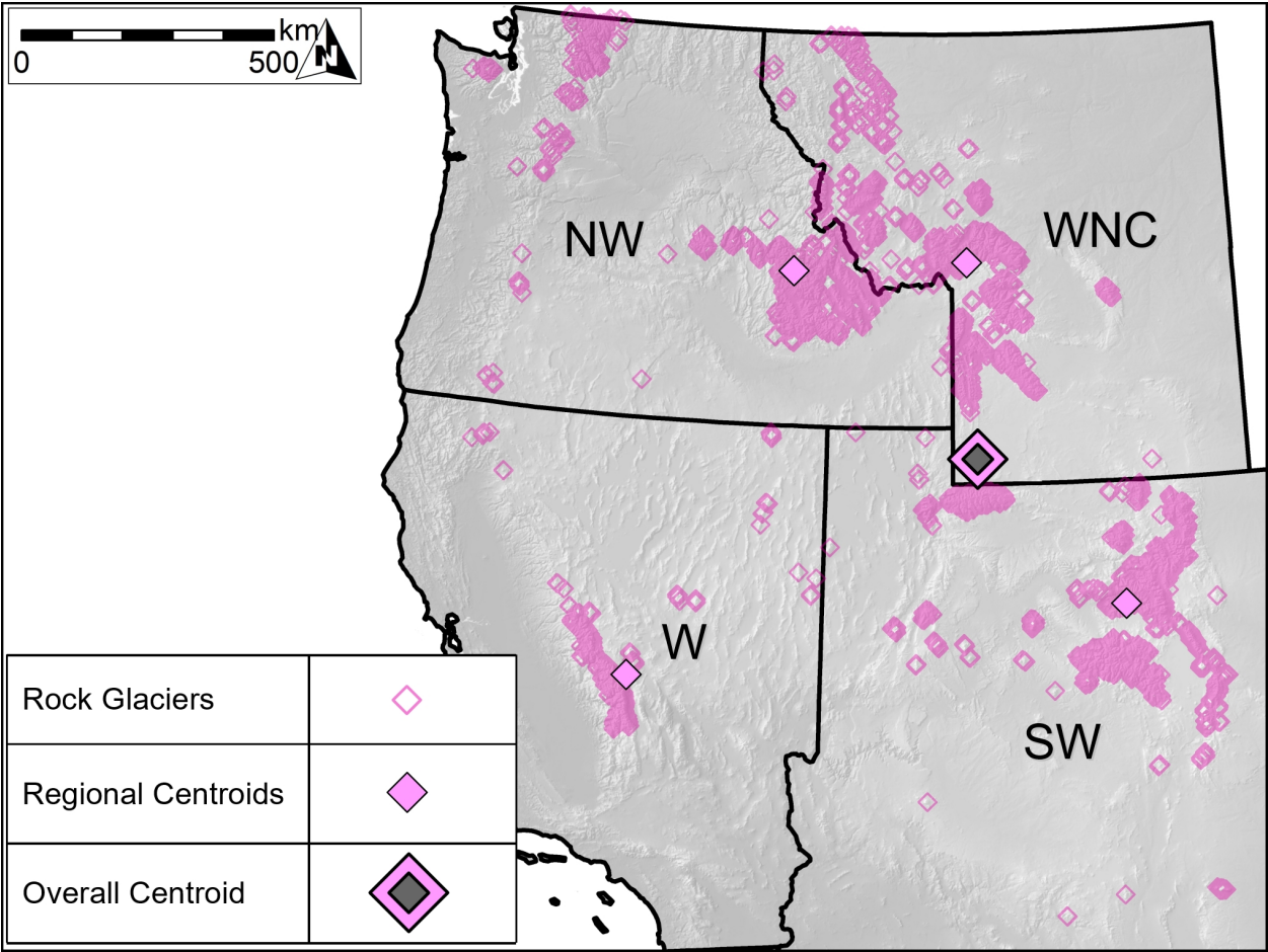
675 | Figure 32: Locations of rock glacier inventory features ( n = 10,332,343 ), as well as centroids for the entire inventory and NOAA Climate Region subsets. The largest rock glaciers, as well as highest rock glacier densities, are found in the relatively arid Southern Rocky Mountains. The Sierra Nevada of California and Uinta Mountains of Utah, climatologically similar to the Southern Rockies, also host large rock glaciers at high densities. Rock glaciers of the humid Cascade Mountains are smaller and less densely distributed, and only a few pockets of rock glaciers are found south of 35^{\circ} N latitude. However, the western U.S. is generally defined by mountainous, high elevation terrain, and rock glaciers are found in all 11 western states.
