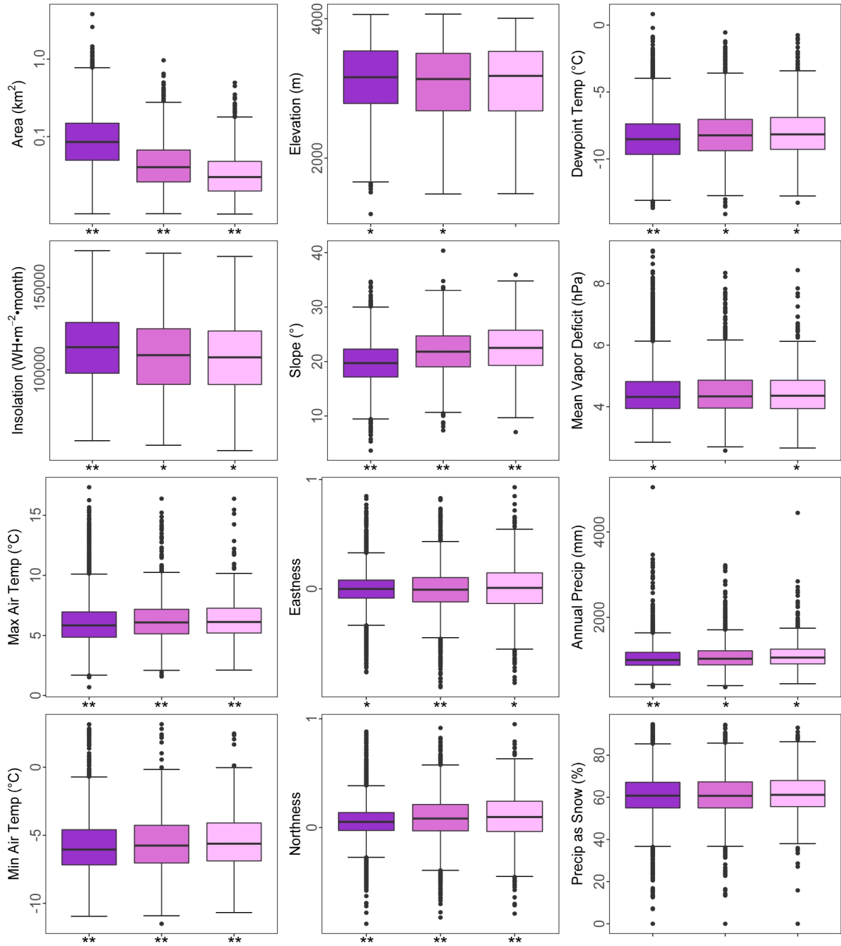
Figure 43: Geographic characteristics of Class 1 (dark purple, n = 70427052), Class 2 (magenta, n = 24152416) and Class 3 (light pink, n = 875) rock glaciers. Statistically significant differences (Tukey's HSD test, \alpha = 0.05 ) are denoted with asterisks (different from one = *, different from both = **). Boxplot whiskers represent 1.5 times the interquartile range, outliers beyond those values are shown by solid dots.
