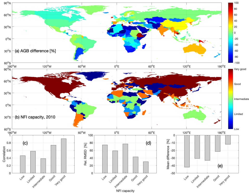
660 Figure 8. Difference between country AGB from our map and FRA, expressed relative to the FRA AGB (a), NFI capacities for the year 2010 (Romijn et al., 2015) (b), Pearson's correlation coefficient (c), relative RMSD (d) and mean difference (e) between map estimates of country AGB and values from the FRA for NFI capacity level. Number of countries per NFI capacity level: 51 (low), 30 (limited), 26 (intermediate), 37 (good) and 23 (very good).
