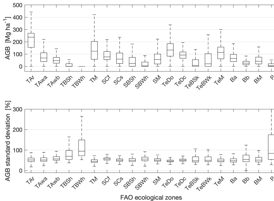
550 Figure 6. Box plot diagram of AGB (top) and its standard deviation by FAO global ecological zone. On each box, the central mark indicates the median, the bottom and top edges delimit the interquartile range, and the whisker delimits the 1-99 percentile range. Labels of global ecological zones: TAR: Tropical rain forest; TAwa: Tropical moist deciduous forest; TAwb: Tropical dry forest; TBSh: Tropical shrubland; TBWh: Tropical desert; TM: Tropical mountain systems; SCf: Subtropical humid forest; SCs: Subtropical dry forest; SBSH: Subtropical steppe; SBWh: Subtropical desert; SM: Subtropical mountain systems; TeDo: Temperate 555 oceanic forest; TeDc: Temperate continental forest; TeBSk: Temperate steppe; TeBWk: Temperate desert; TeM: Temperate mountain systems; Ba: Boreal coniferous forest; Bb: Boreal tundra woodland; BM: Boreal mountain systems; P: Polar.
