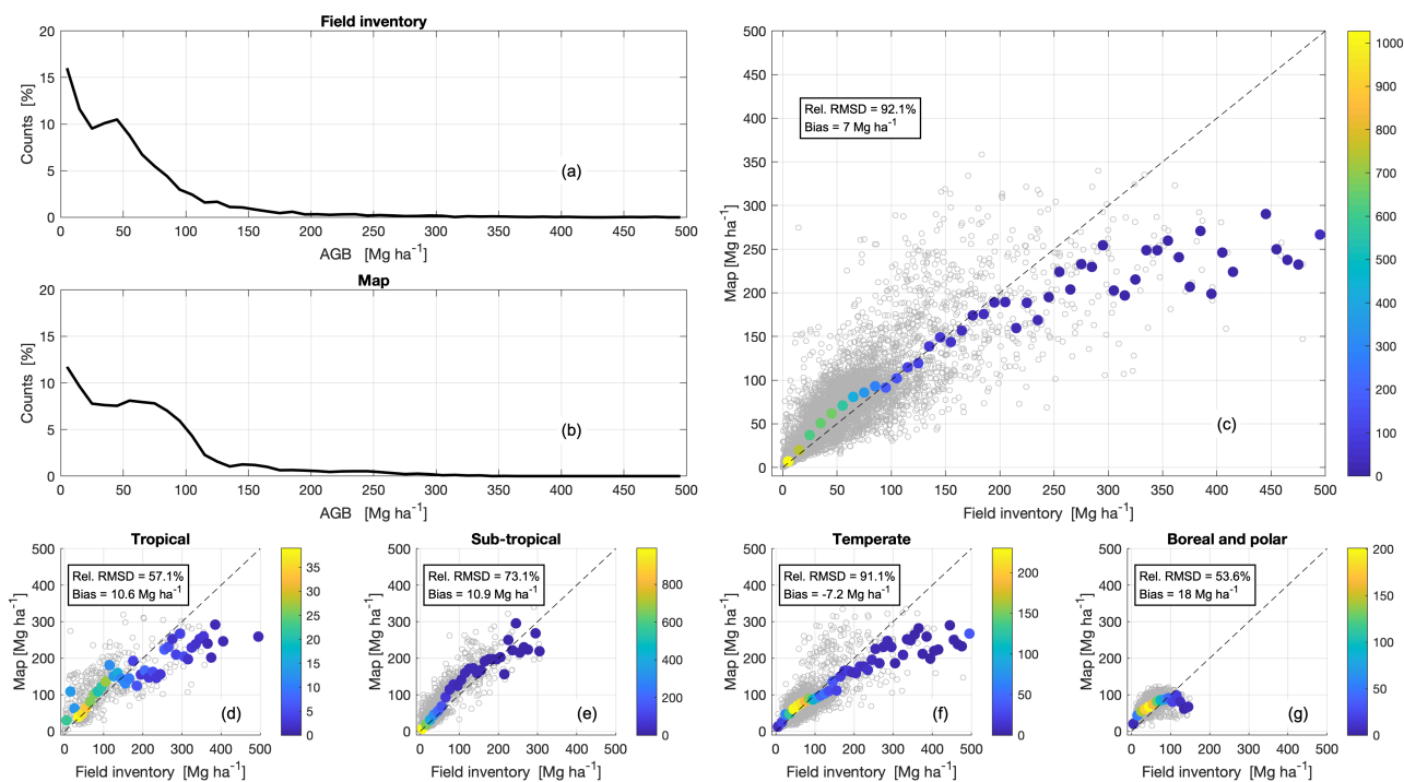
495 Figure 5. Histograms of AGB from the field inventory database (a) and the map (b) for 0.1° grid cell values. (c) Scatterplot of map AGB against field inventory values for 0.1° grid cells (grey circles); the filled circles show the median AGB of the map values in each 10 Mg ha -1 wide interval of field inventory AGB values. The colour bar represents the number of grid cells within a given AGB interval. Similar scatterplots are given for the tropical zone (d), the sub-tropical zone (e), the temperate zone (f) and the boreal and polar zones (g) according to the FAO Global Ecological Zones. On each scatterplot, we report the root mean squared difference (RMSD) between map and field inventory AGB relative to the mean value of the reference AGB and the bias, i.e., the difference between mean values of the map AGB and the reference AGB. To improve presentation and because of the paucity of grid cells with AGB above 500 Mg ha -1 , axes are truncated at 500 Mg ha -1 .
