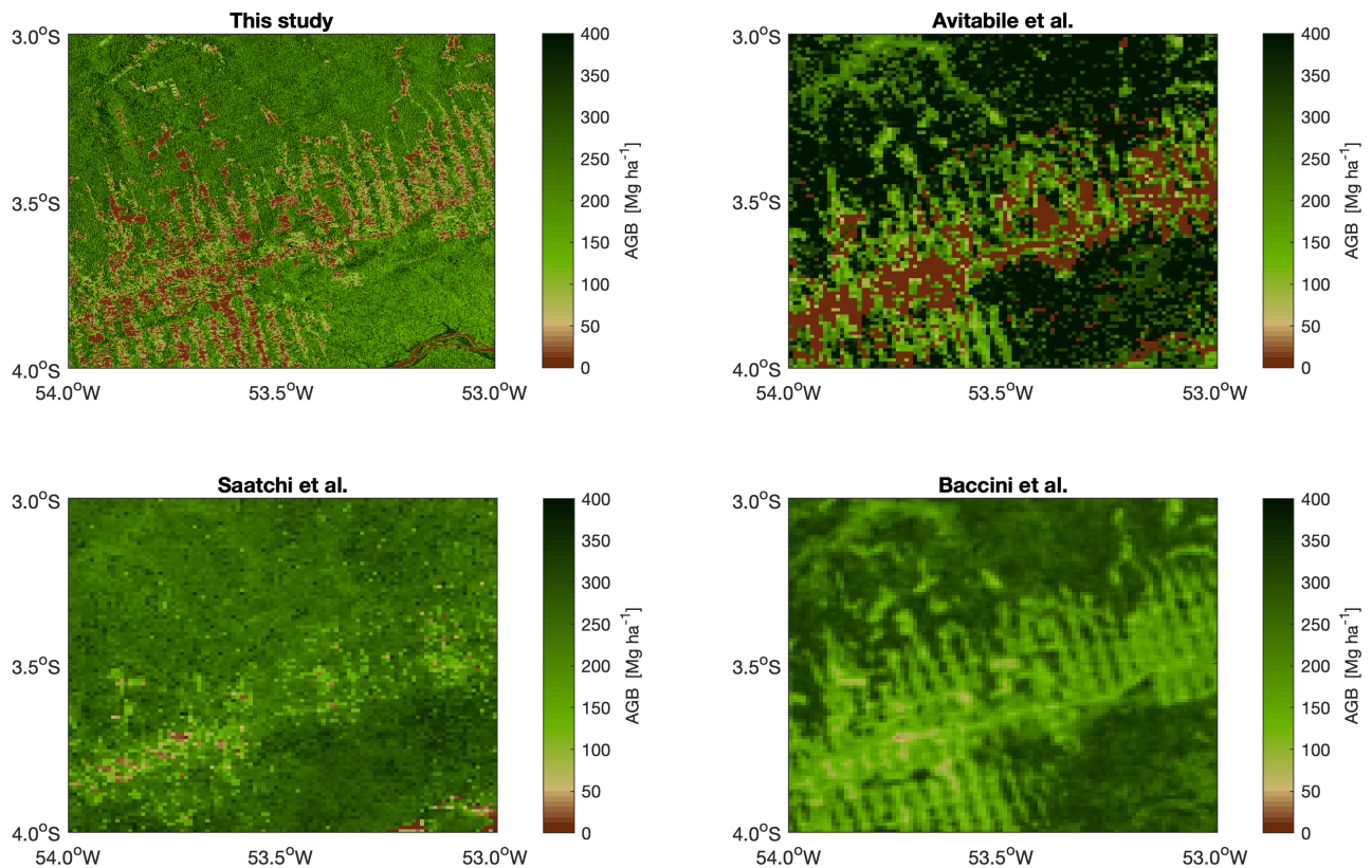
475 Figure 4. AGB estimates by this study (top left), Avitabile et al. (2016) (top right), Saatchi et al. (2011b) (bottom left) and Baccini et al. (2012) (bottom right) for a 1^\circ \times 1^\circ area in the state of Pará, Brazil.
