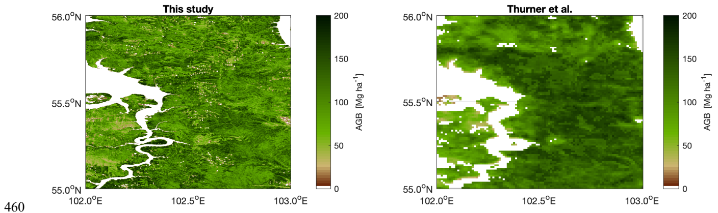
Figure 3. AGB estimates from this study (left) and from Thurner et al. (Thurner et al., 2014) for a 1^\circ \times 1^\circ area in Central Siberia.
