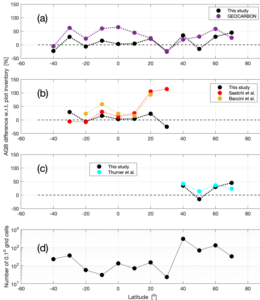
Figure 11. Relative difference of AGB from maps and plot inventory data averaged over the 0.1° grid cells validation cells (a, b and c). The number of grid cells stratified by 10°-wide latitude intervals is illustrated in (d).
