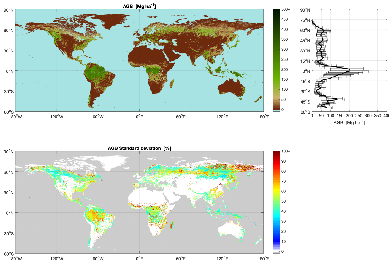
425 Figure 2. Map estimates of AGB (top panel) and AGB standard deviation expressed relative to the AGB (bottom panel). The colour bar of the AGB map has been truncated at 500 Mg ha -1 to increase contrast. Similarly, the colour bar of the AGB relative standard deviation has been truncated at 100%. The right hand panel shows the profile of average AGB along latitude (thick solid line) and the two-sided average standard deviation of AGB at a given latitude (horizontal bars).
