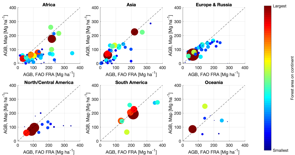
655 Figure 7. Average AGB per country from the FAO FRA 2010 country reports and our map dataset. Countries have been grouped per continent. The size of each circle is proportional to the forest area of the country derived from the CCI Land Cover dataset (same scaling across all continents). The colour ramp associated to the circles gives a graphical representation of the relative country forest area (different for each continent).
