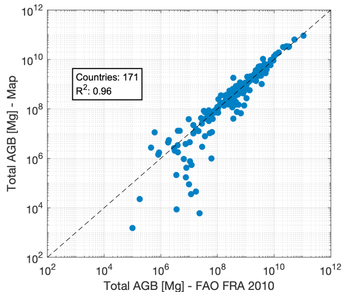
680 Figure 9. Total AGB from the FAO FRA 2010 country reports and from our dataset (see Table S7 for details).
