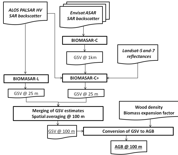
Figure 1. Flowchart of the AGB retrieval approach.
