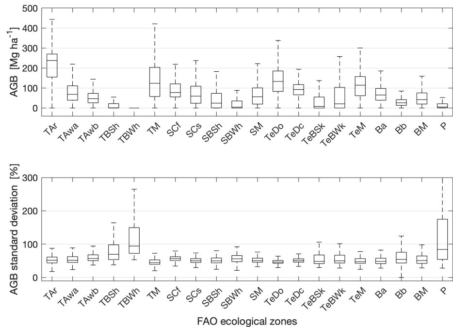
Figure 6. Box plot diagram of AGB (top) and its standard deviation by FAO global ecological zone. On each box, the central mark indicates the median, the bottom and top edges delimit the interquartile range, and the whisker delimits the 1-99 percentile range. Labels of global ecological zones: TAr: Tropical rain forest; TAwa: Tropical moist deciduous forest; TAwb: Tropical dry forest; TBSh: Tropical shrubland; TBWh: Tropical desert; TM: Tropical mountain systems; SCf: Subtropical humid forest; SCs: Subtropical dry forest; SBSH: Subtropical steppe; SBWh: Subtropical desert; SM: Subtropical mountain systems; TeDo: Temperate oceanic forest; TeDc: Temperate continental forest; TeBSk: Temperate steppe; TeBWk: Temperate desert; TeM: Temperate mountain systems; Ba: Boreal coniferous forest; Bb: Boreal tundra woodland; BM: Boreal mountain systems; P: Polar.
