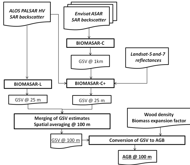
Figure 1. Flowchart of the AGB retrieval approach.
