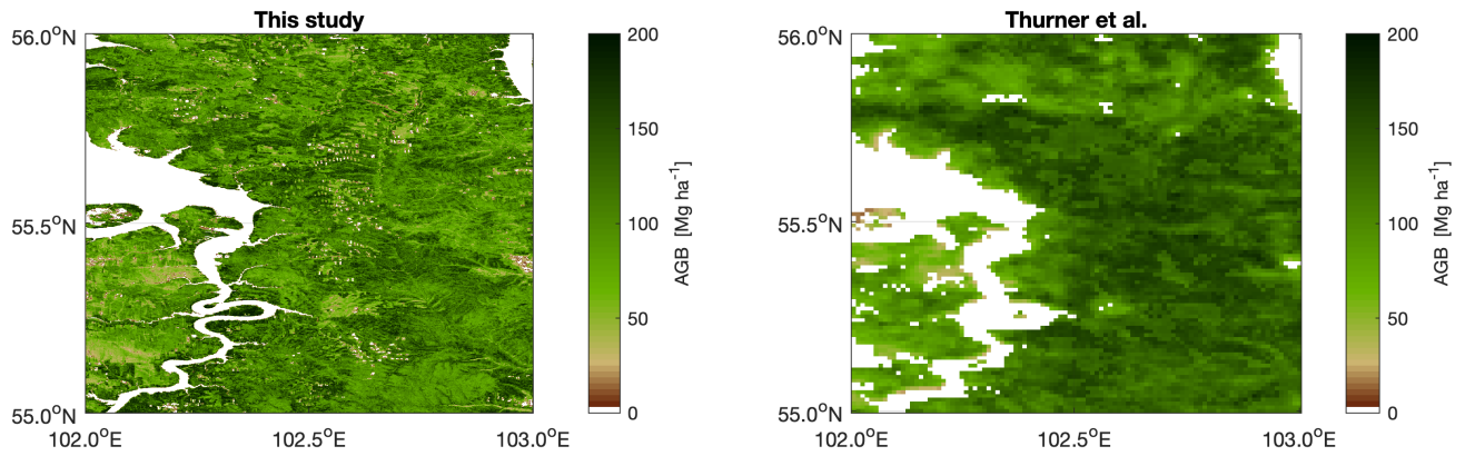
460 Figure 3. AGB estimates from this study (left) and from Thurner et al. (Thurner et al., 2014) for a 1° × 1° area in Central Siberia.
