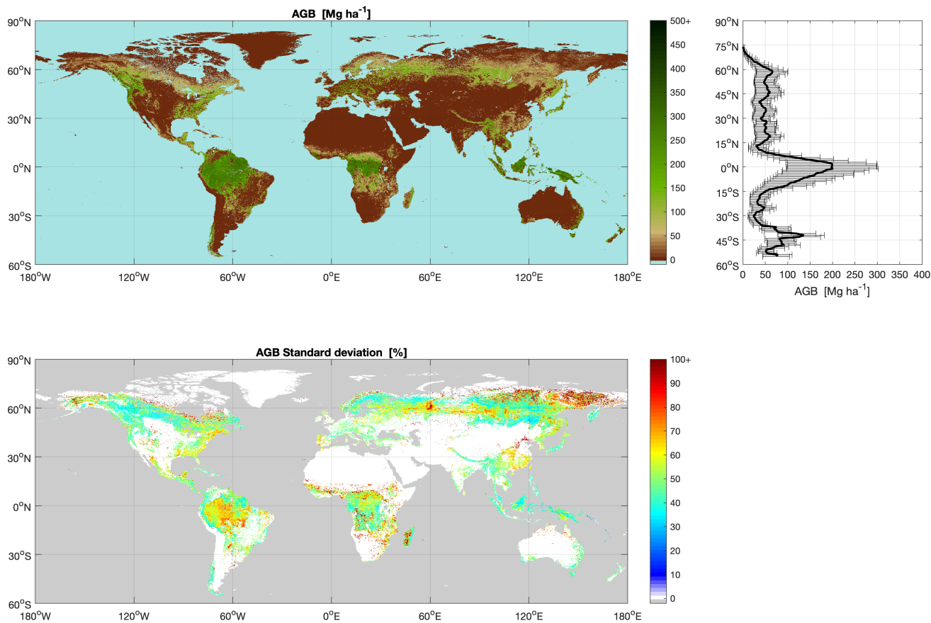
Figure 2. Map estimates of AGB (top panel) and AGB standard deviation expressed relative to the AGB (bottom panel). The colour bar of the AGB map has been truncated at 500 \text{ Mg ha}^{-1} to increase contrast. Similarly, the colour bar of the AGB relative standard deviation has been truncated at 100%. The right hand panel shows the profile of average AGB along latitude (thick solid line) and the two-sided average standard deviation of AGB at a given latitude (horizontal bars).
