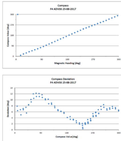
Fig. 2. calibration of one of the compasses
