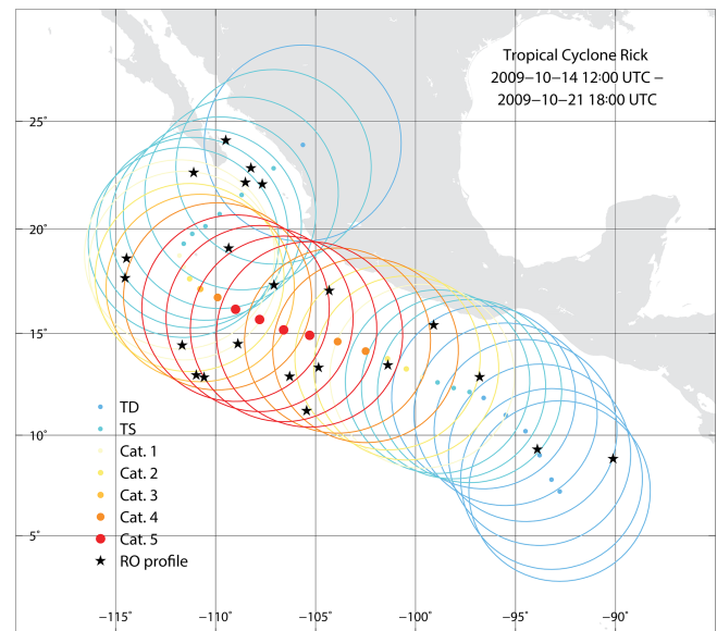
Figure 1. An example of co-location of TC with RO profiles (black stars) based on Hurricane Rick developed between 14 and 21 October 2009. Dots present the TC eye position, whilst circles mark the 500 km co-location criterion. Colours indicate the intensity of TC.
