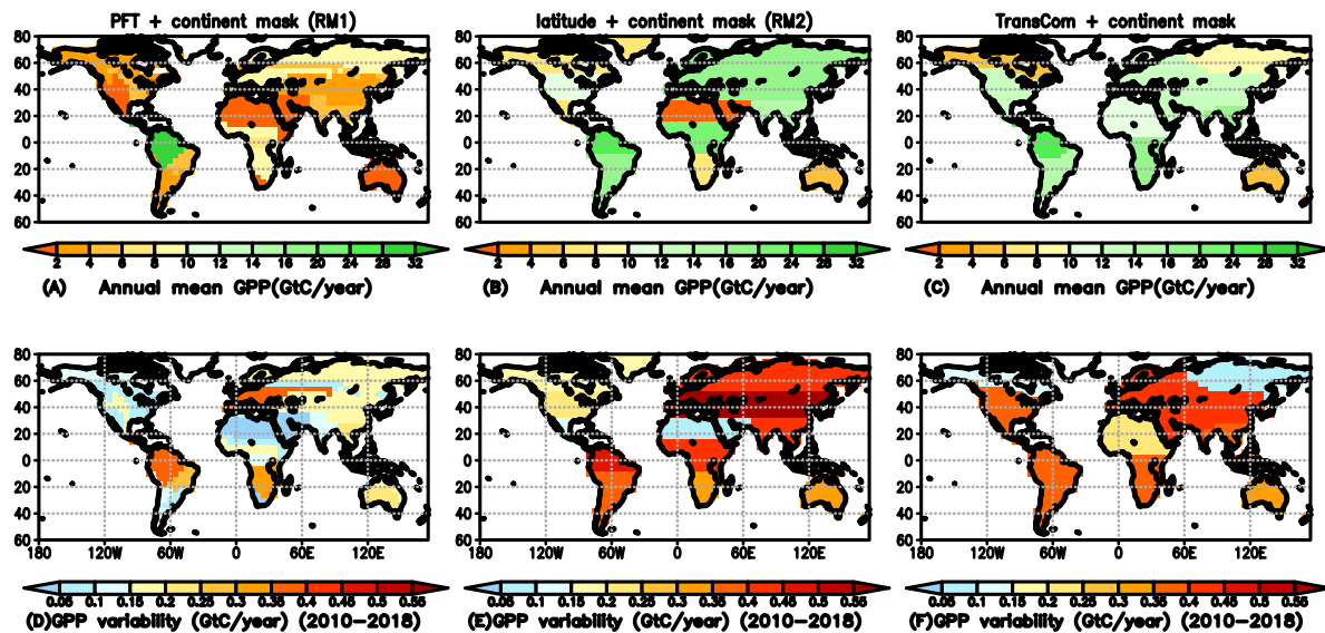
Figure B4 Regional mean FIUXSAT GPP and its variability between 2010 –2018. (A, B, and C) Regional mean GPP aggregated with the three regional masks; (D, E, and F) GPP variability between 2010 –2018. Unit: GtC/year.
