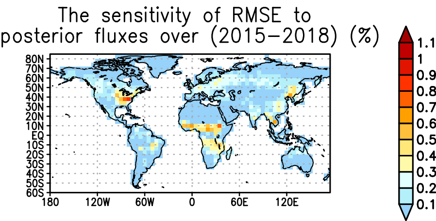
Figure B5 The relative sensitivity of root mean square errors (RMSE) of posterior CO 2 (Figure 9 in the main text) relative to NBE at every grid point. The adjoint model is carried out over Sep 2014–Dec 2018.
