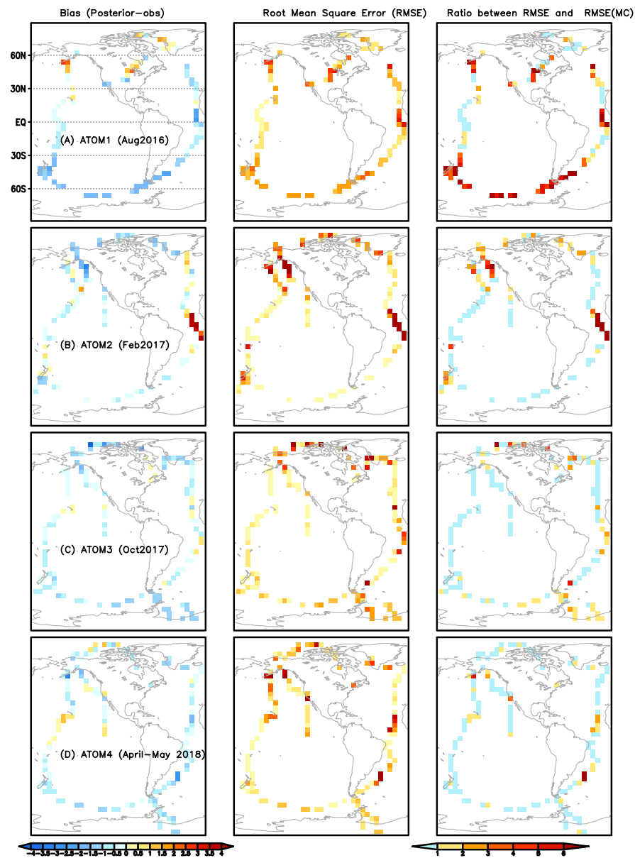
Figure: 10 Left column: the mean differences between posterior CO 2 and aircraft observations from ATOM 1–4 aircraft campaigns between 1–5 km (A–D). Middle column: the Root Mean Square Errors (RMSE) between aircraft observations and posterior CO 2 between 1–5 km. The color bar is the same as the left column. Right column: the ratio between RMSE and RMSE MC based on ensemble CO 2 from the Monte Carlo uncertainty estimation method.
