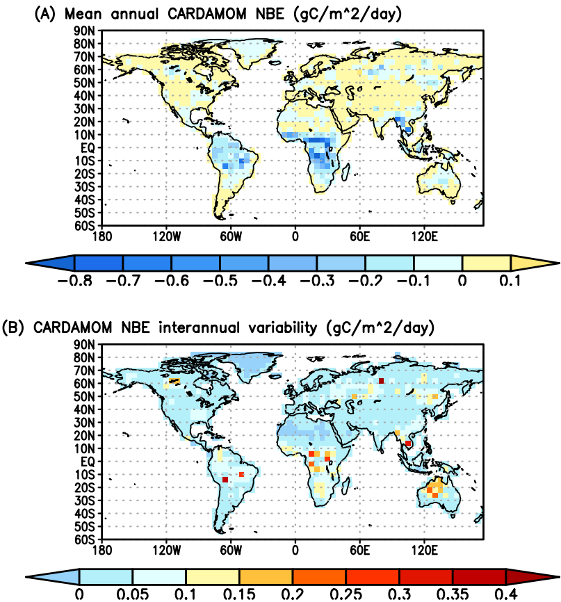
711 712 Figure B1 Annual mean net biosphere exchanges from CARDAMOM (A) and its interannual 713 variability between 2010 and 2017 (B).
