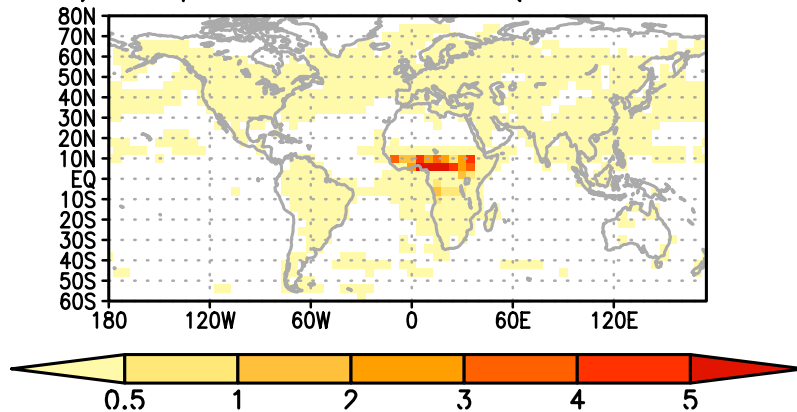
Figure B8 The relative sensitivity of RMSE of posterior \text{CO}_2 to NBE over land and air-sea net carbon exchange over ocean at every grid point. The RMSE is calculated against aircraft \text{CO}_2 observations from ATom-1 (A) and ATom-2 (B) between 40^\circ\text{W} – 0^\circ , 20^\circ\text{S} – 20^\circ\text{N} . The adjoint model is carried out over June – August 2016 (A) and Dec 2016 – Feb 2017 (B). Unit: %.
