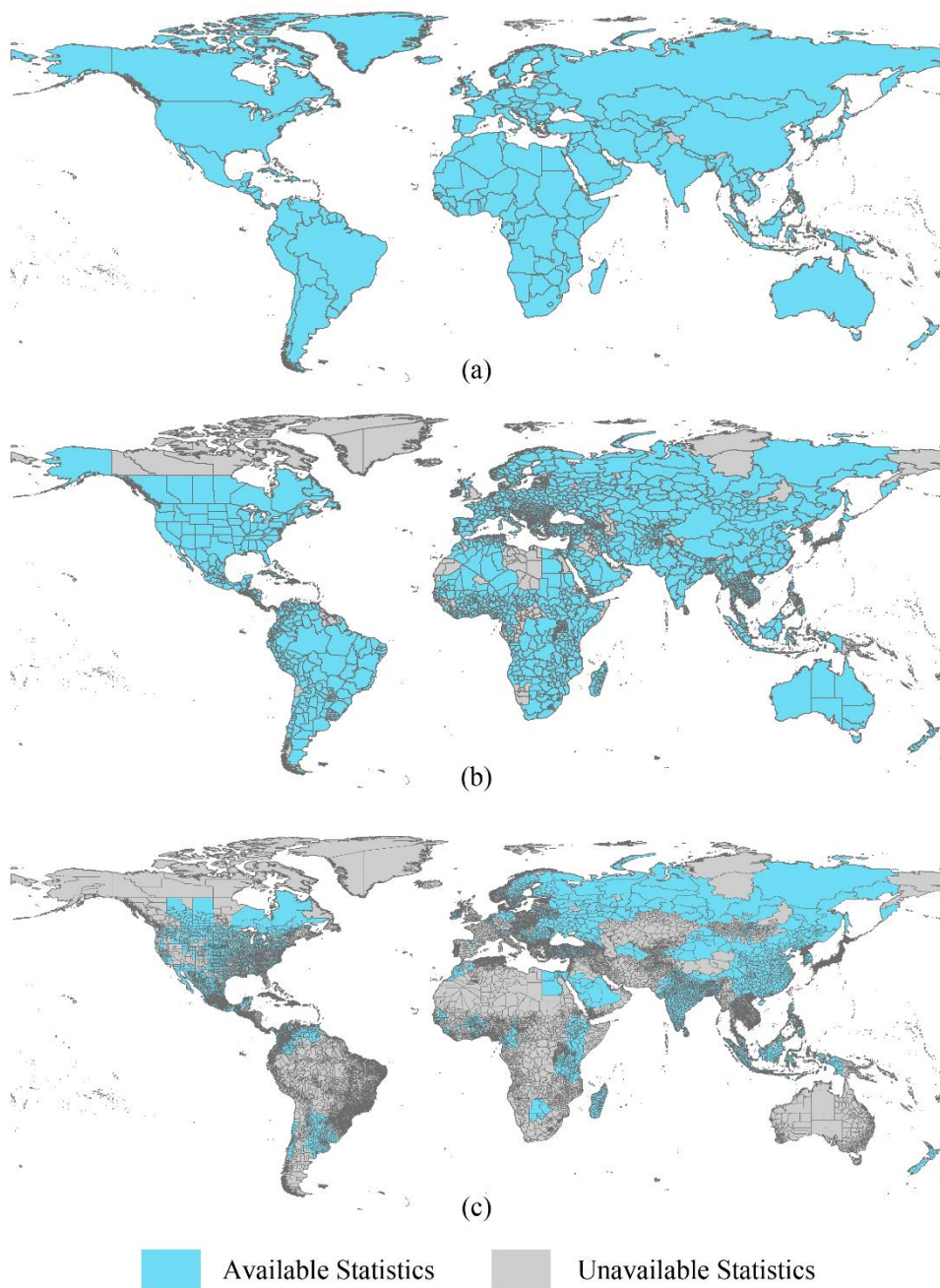
Figure 1: The statistics of cropland area at the national (a), first subnational (b), and second subnational (c) levels.
