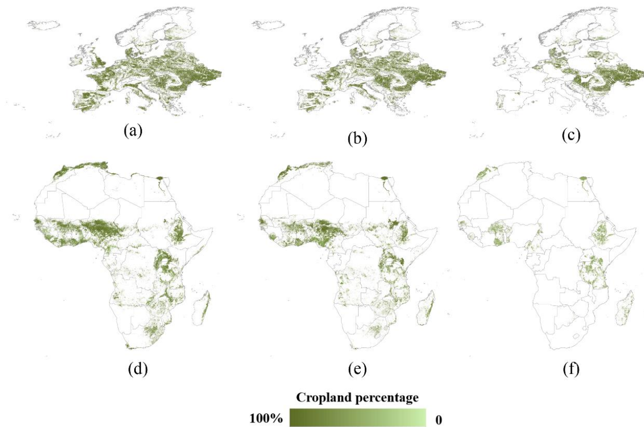
650 Figure 5: Statistics allocation results in Europe and Africa: (a) and (d) are the national allocation results; (b) and (e) are the first subnational allocation results, (c) and (f) are the second subnational allocation results.
