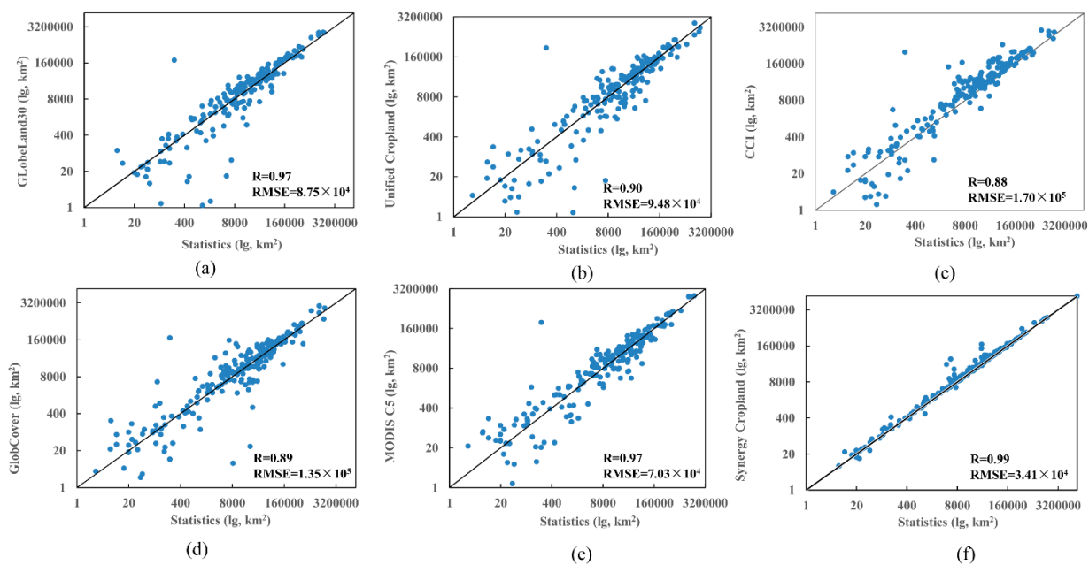
Figure 7: The consistency analysis between cropland areas estimated from products and statistics: (a) GlobeLand30, (b) Unified Cropland, (c) CCI-LC, (d) GlobCover 2009, (e) MODIS C5, and (f) synergy map.
