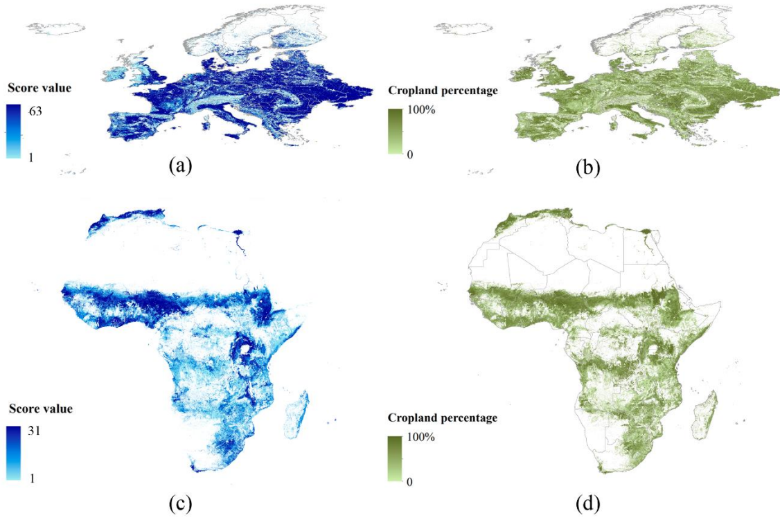
Figure 4: Agreement ranking score maps and average cropland percentages in Europe and Africa: (a) and (b) are the score map and cropland percentage of Europe; (c) and (d) are the score map and cropland percentage of Africa.
