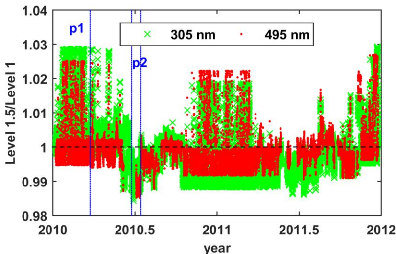
575 Figure 6: Ratio between the Level 1.5 and the Level 1 irradiances, at 305 nm (green x) and 495 nm (red dots). Two different periods have been marked on the graph in order to assist further discussion: p1 at the beginning of 2010 and p2 at mid-2010. The two wavelengths refer to the average of a band, over \pm 5 nm around the central wavelength.
