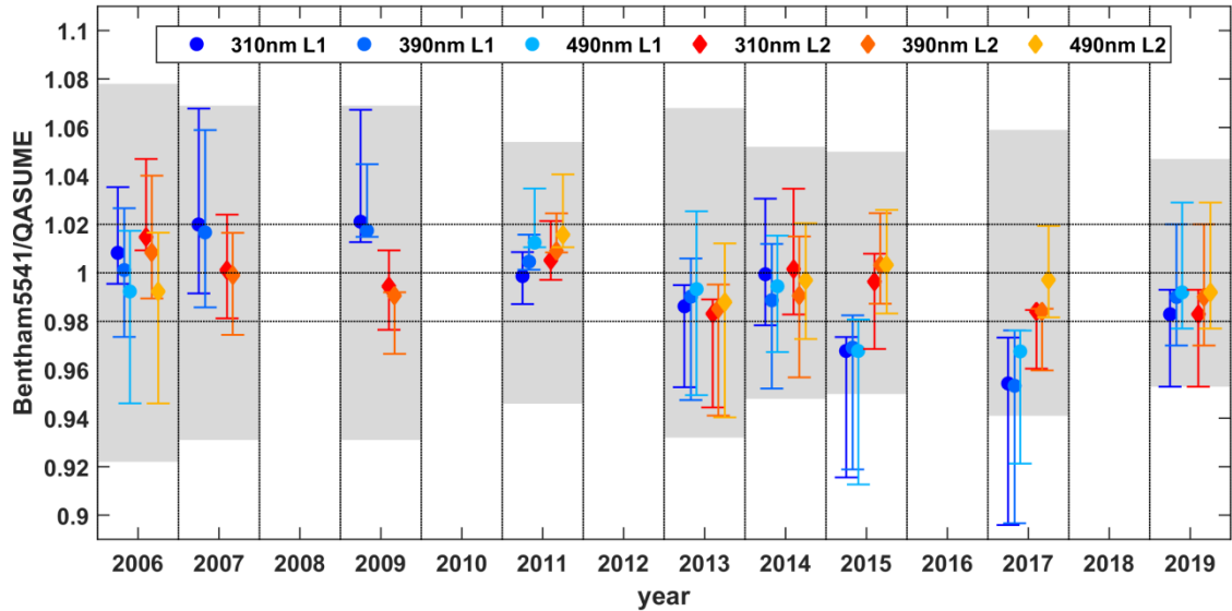
Figure 8: Average ratio between the measurements of Bentham5541 and QASUME at 310 nm, 390 nm, and 490 nm, and the corresponding 5/95 percentiles Shaded grey areas represent the combined expanded uncertainty of the Bentham5541 Level 2 and the QASUME spectra for each intercomparison.
