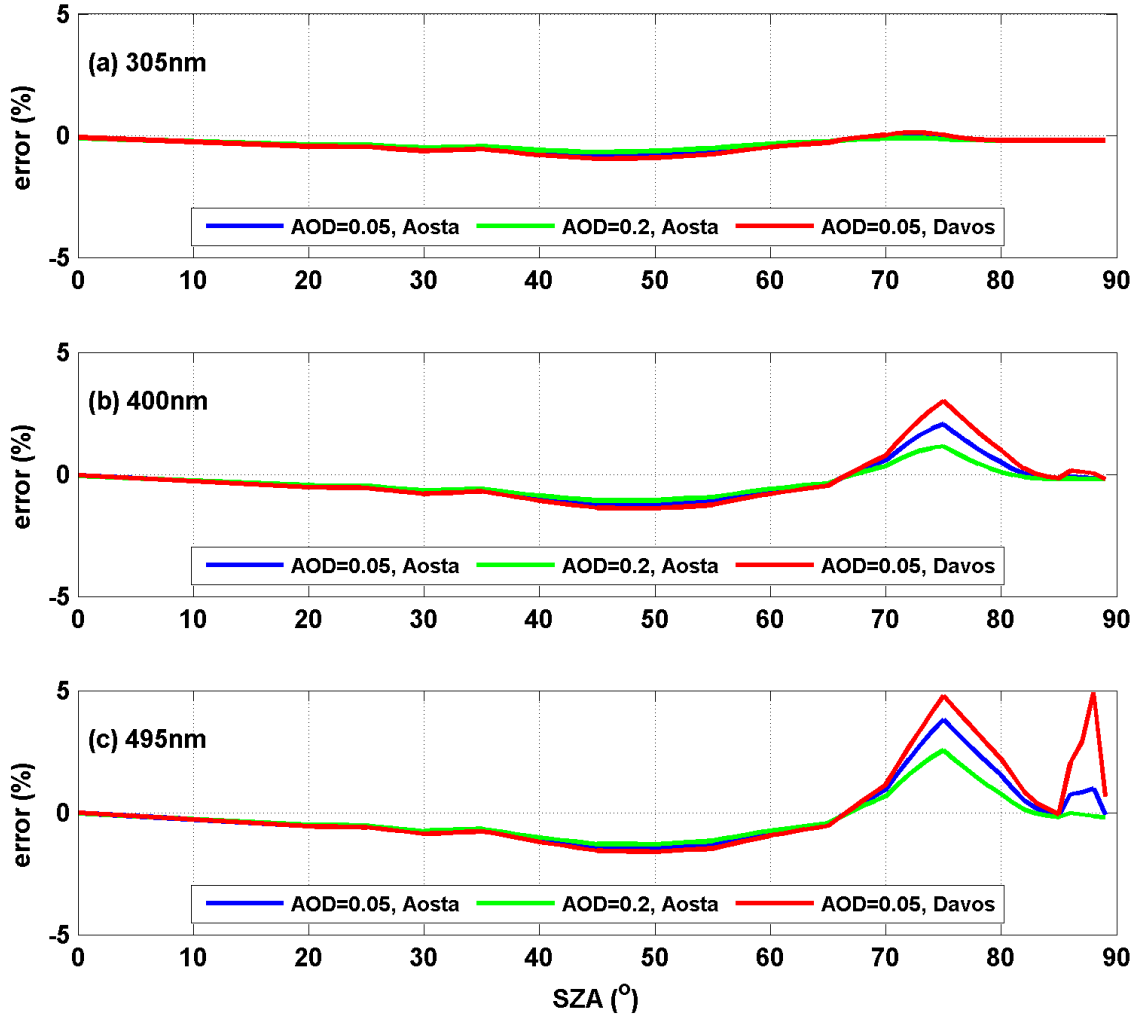
Figure 4: Modeled error in the measured global irradiance for three different wavelengths: (a) 305 nm, (b) 400 nm, and (c) 495 nm. The results are for AAO (for AOD at 500 nm equal to 0.05 and 0.2) and the PMOD-WRC (for AOD at 500 nm equal to 0.05).
