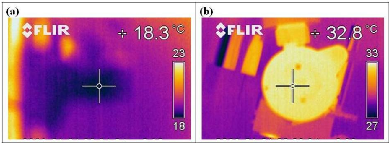
Figure 2: Temperature of the OH (a) in the morning with the internal heating turned off, and (b) with the internal heating turned on. The temperature stabilization system warms the diffuser uniformly as shown in Fig. 2, where two different pictures taken with the thermal camera (with the temperature stabilization system off (a) and on (b)) are presented. In both the homogeneity in the temperature of the OH is obvious. Fountoulakis et al. (2017) showed that during measurements of the irradiance using 50 Watt lamps (distance between the lamp filament and the diffuser was 5 cm) with a Brewer spectrophotometer, the temperature of the Teflon diffuser was inhomogeneous, and was higher by 5-6°C at the center relative to the edges of the diffuser. At AAO the irradiance from 200 Watt lamps is measured using a KS-J1011 portable field calibrator (PFC) provided by Schreder CMS ( http://www.schreder-cms.com/en/ ). The distance between the lamps' filament and the diffuser is 12 cm for the original setup, and can be increased to 30 cm with the use of an extender. Measurements with the thermal camera in AAO showed that even when the extender is not used during measurements of the irradiance from the lamps, the temperature variations over the diffuser are below 2°C. In all cases discussed above the temperature recorded by the thermistor, and the temperature measured by the thermal camera agreed within 1°C.
