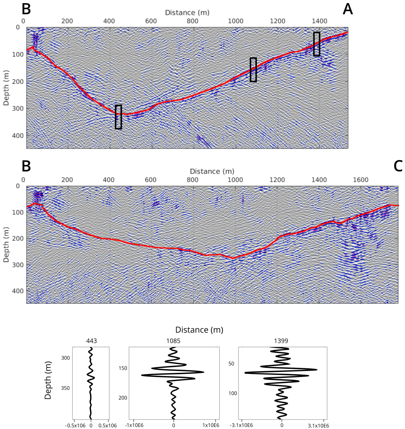
Figure 3. Resulting radargrams showing the manually interpreted bedrock in red. The x-axis shows the distance covered during the measurements. The y-axis represents the estimated bedrock depth in meters. The lower plot depicts A-scope examples of the attenuation of the signal at different depth from B to A.
