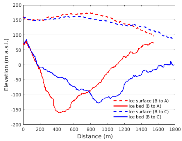
Figure 4. Ice surface and glacier bed elevation along the profiles shown in Figure 3.
