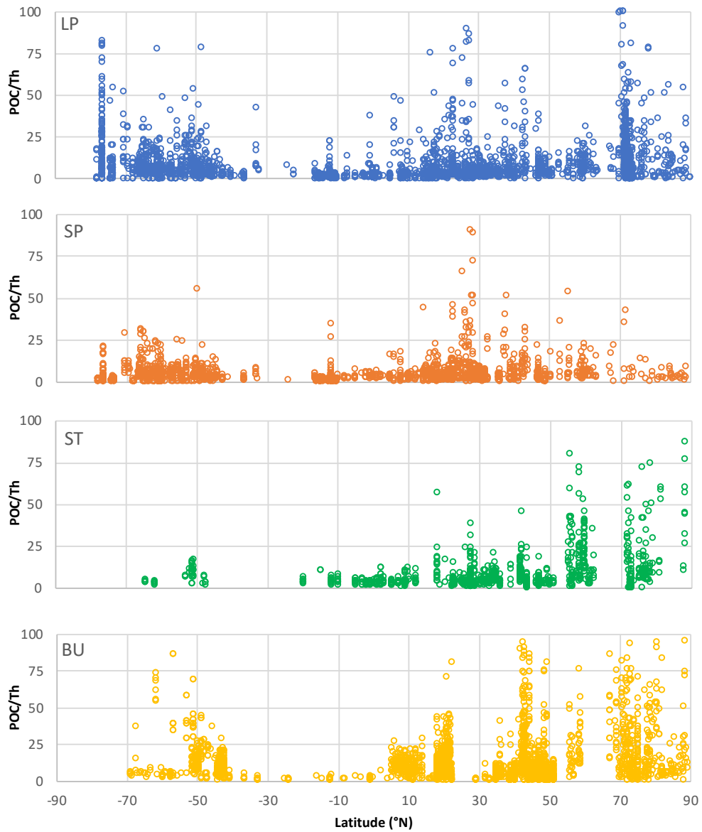
Figure 5: Latitudinal variability of the POC/Th ratios (<100 \mu\text{mol/dpm} ) grouped by large particles (LP), small particles (SP), sediment trap particles (ST) and bulk particles (BU).
