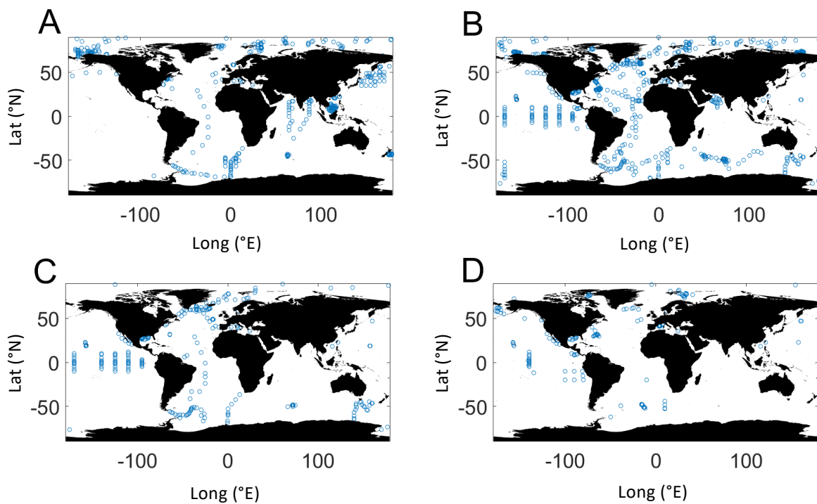
Figure 1: Maps showing the distribution of POC/Th ratios measured on (A) bulk particles, (B) large particles, (C) small particles, and (D) particles from sediment traps. See main text for details, section 3.1 Data classification.
