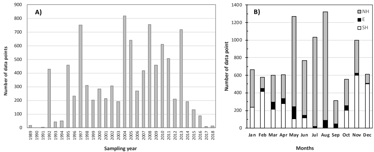
Figure 3: A) Histogram of data sampled between 1989 and 2018. See Table 1 for details. B) Number of samples per month of the year grouped as per samples collected in the Northern Hemisphere (NH; grey), Southern Hemisphere (SH; white) or Equator (E; -10^{\circ} to 10^{\circ} N; black).
