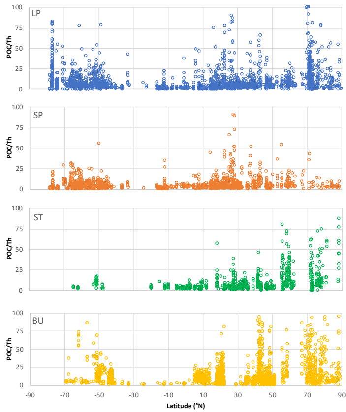
Figure 5: Latitudinal variability of the POC/Th ratios ( <100 \mu\text{mol/dpm} ) grouped by large particles (LP), small particles (SP), sediment trap particles (ST) and bulk particles (BU).
