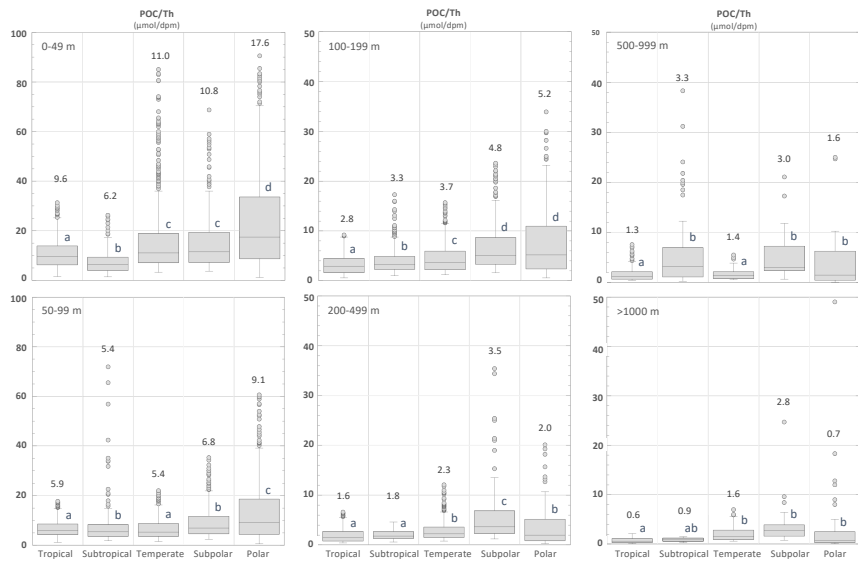
Figure 4: POC/Th ratios variability (box whisker plots) of 90% of the data sorted by climate zones and depth. The values shown on top of each box represent their median. Box plots within the same depth range (e.g., 0-49 m) sharing a letter are not significantly different. Note the different scale used between the 0 to 99 m and the 100 to >1000 m plots.
