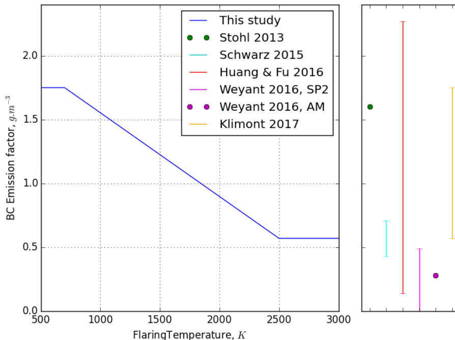
Figure 3. Left: BC emission factor function used in the present study. The emission factor is bounded by the extremes of the range used in the GAINS model ( 0.5 - 1.75 \text{ g} \times \text{m}^{-3} ) (Klimont et al., 2017) and scaled as a function of the flaring temperature, used as an indication of combustion completeness. Right: For comparison purposes, the EFs derived by Stohl et al. (2013); Schwarz et al. (2015); Huang and Fu (2016), Weyant et al. (2016) (using the Single Particle Soot Photometer, SP2, or the Particle Soot Absorption Photometer, AM) and Klimont et al. (2017).
