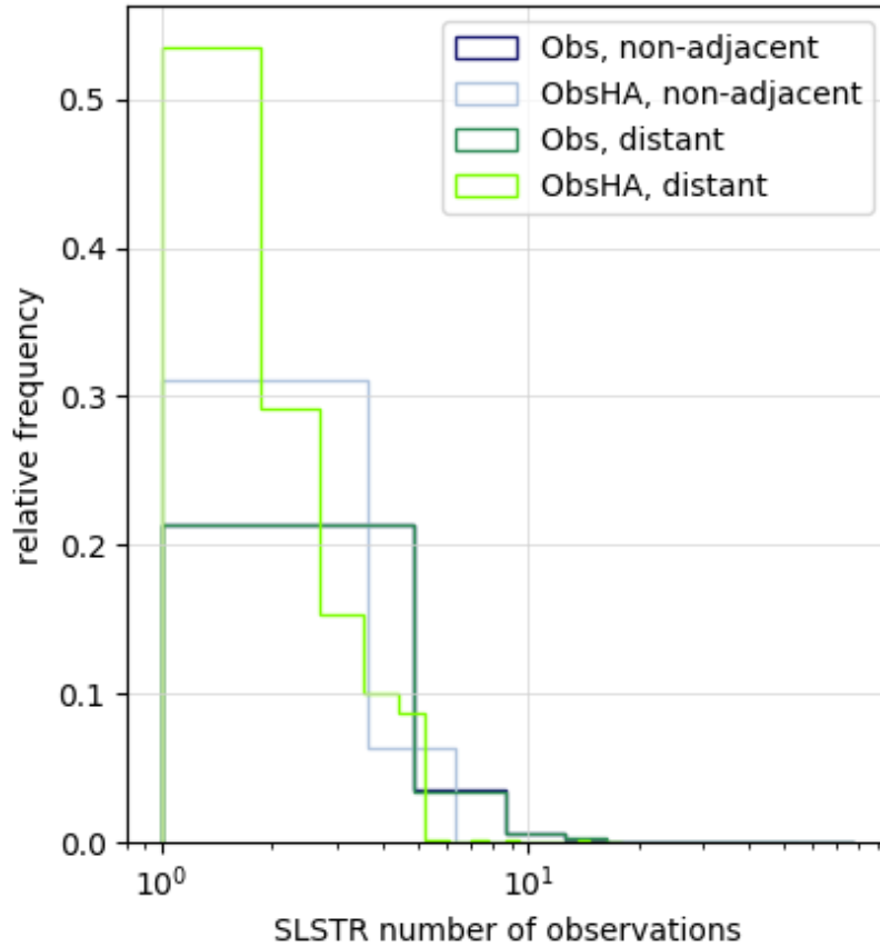
Figure 20. Number of SLSTR-based observations and high-accuracy observations distributions at VNF non-adjacent (the VNF flaring location is \geq 2 grid cells away from the closest SLSTR-based flaring location) and distant ( >4 grid cells away) locations. The diminute number of observations at distant locations supports the argument that our methodology has a tendency to undersample low activity flares when compared to VNF. Our analysis shows that the undersampling is due to less observation opportunities by SLSTR, which can be traced back to a slightly earlier overpass time and a much smaller swath.
