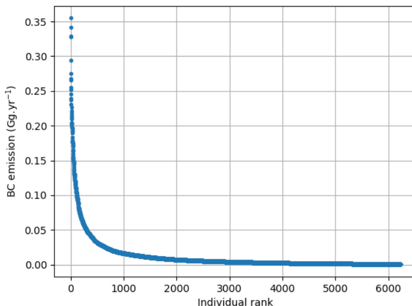
Figure 14. Flaring BC emissions (best estimate, Gg per year) for each individual flaring location (6232 in total).
