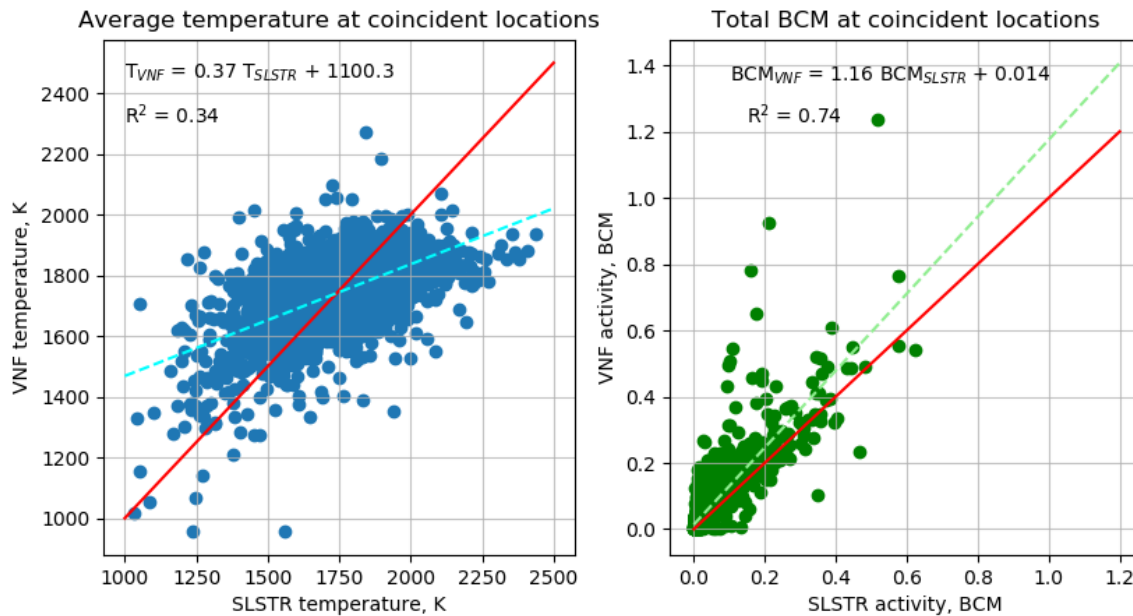
Figure 17. Comparison of the average temperature and the total BCM retrieved by VIIRS Nightfire and the SLSTR-based method at the 2964 coincident flaring locations. The red line represents the 1:1 relationship. The dashed line represents the linear regression between both methodologies.
