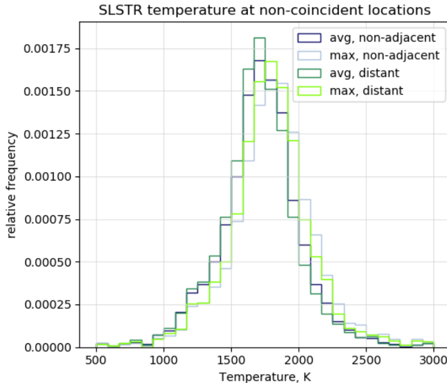
Figure 19. Average and maximum SLSTR-based temperature distributions at VNF VNF non-adjacent (the VNF flaring location is \geq 2 grid cells away from the closest SLSTR-based flaring location) and distant ( >4 grid cells away) locations. The similar temperature distribution between the different types of flaring sites supports the argument that the discrepancy in the number of flaring sites is not due to the temperature criterion, but to the observation criterion, which can be traced back to less observation opportunities.
