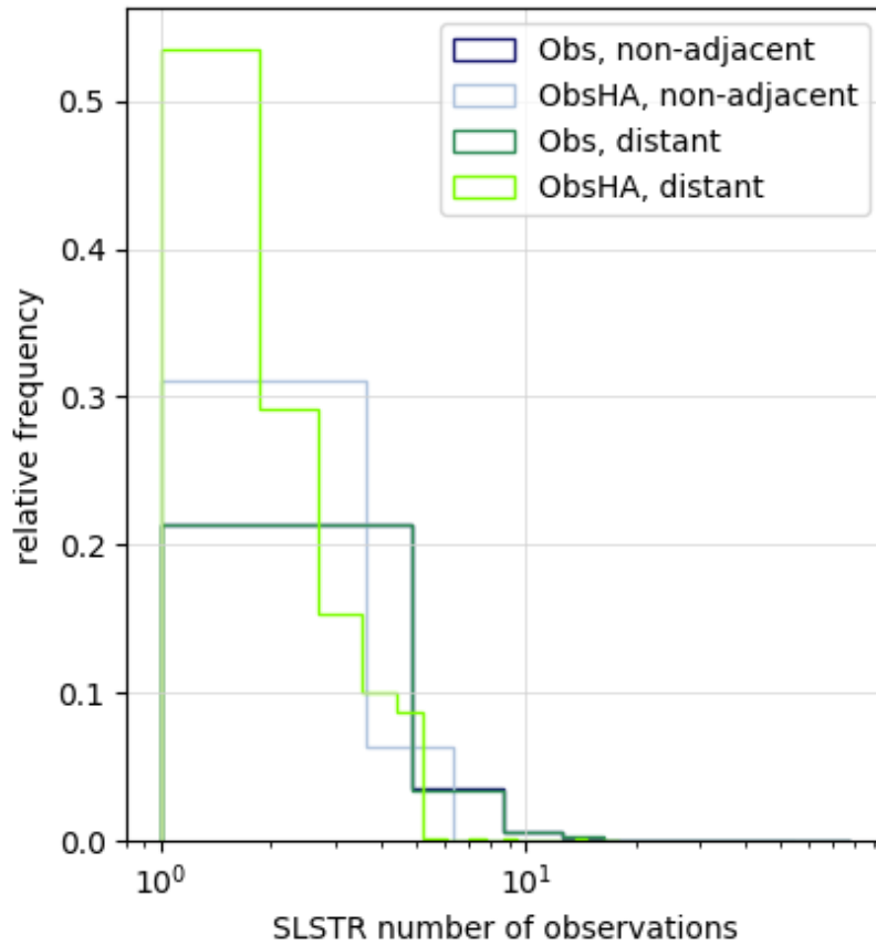
Figure 20. Number of SLSTR-based observations and high-accuracy observations distributions at VNF non-adjacent (the VNF flaring location is \geq 2 grid cells away from the closest SLSTR-based flaring location) and distant ( >4 grid cells away) locations. The diminute number of observations at distant locations supports the argument that our methodology has a tendency to undersample low activity flares when compared to VNF. Our analysis shows that the undersampling is due to less observation opportunities by SLSTR, which can be traced back to a slightly earlier overpass time and a much smaller swath.
