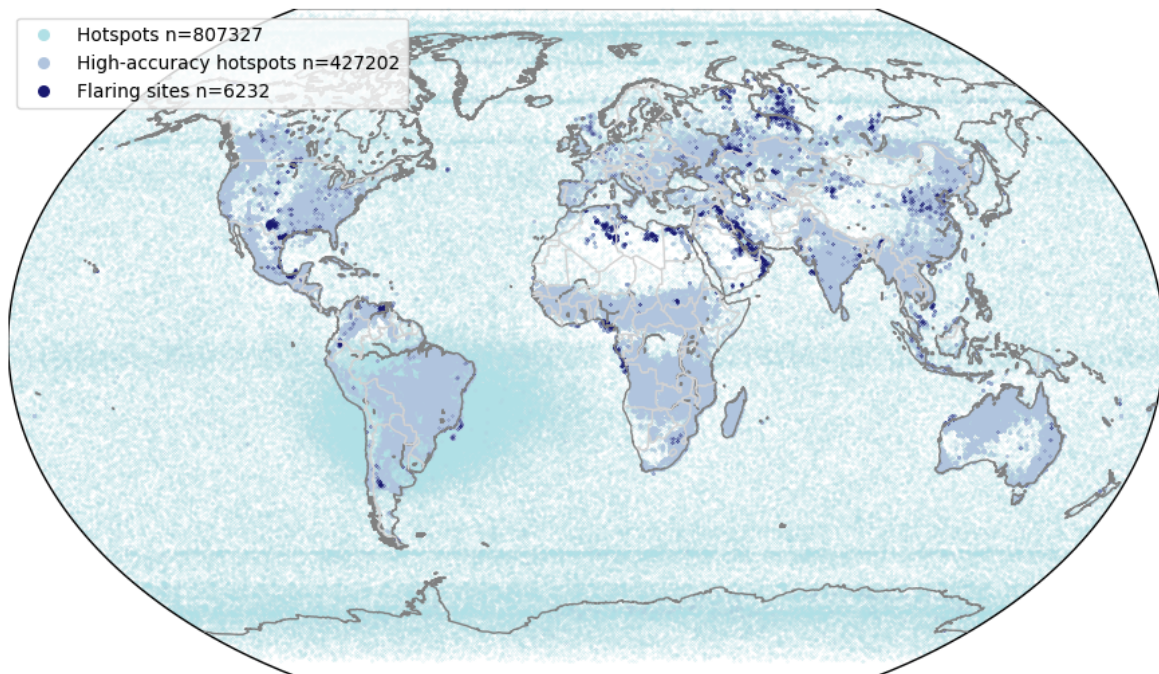
Figure 4. Location of all the 807327 hot spots (all detections database filtered for spurious signals, see Figure 1), of all the 427202 high-accuracy hot spots (hot spots filtered for cloudiness and accuracy of the Planck curve fitting, see Figure 1) and of all the 6232 flaring locations (grid cells with at least 5 high-accuracy hot spots and a maximum retrieved temperature above 1500 K), detected in 2017.
