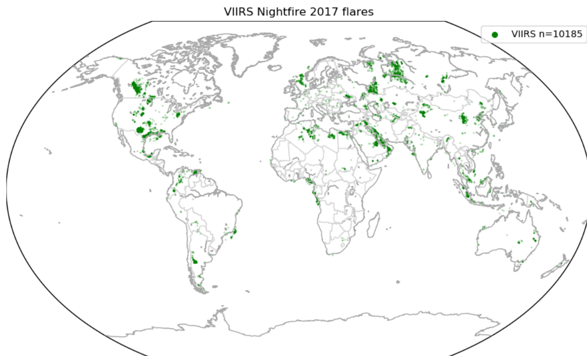
Figure 16. VIIRS Nightfire flaring locations for 2017. We considered every record in the VIIRS Nightfire data as a flare, i.e. "upstream" (10009), "downstream oil" (718) and "downstream gas" (101). After gridding, 10185 cells were populated and are considered as flaring sites. A detailed spatial analysis between these locations and those found by our methodology is shown in Figure 18
