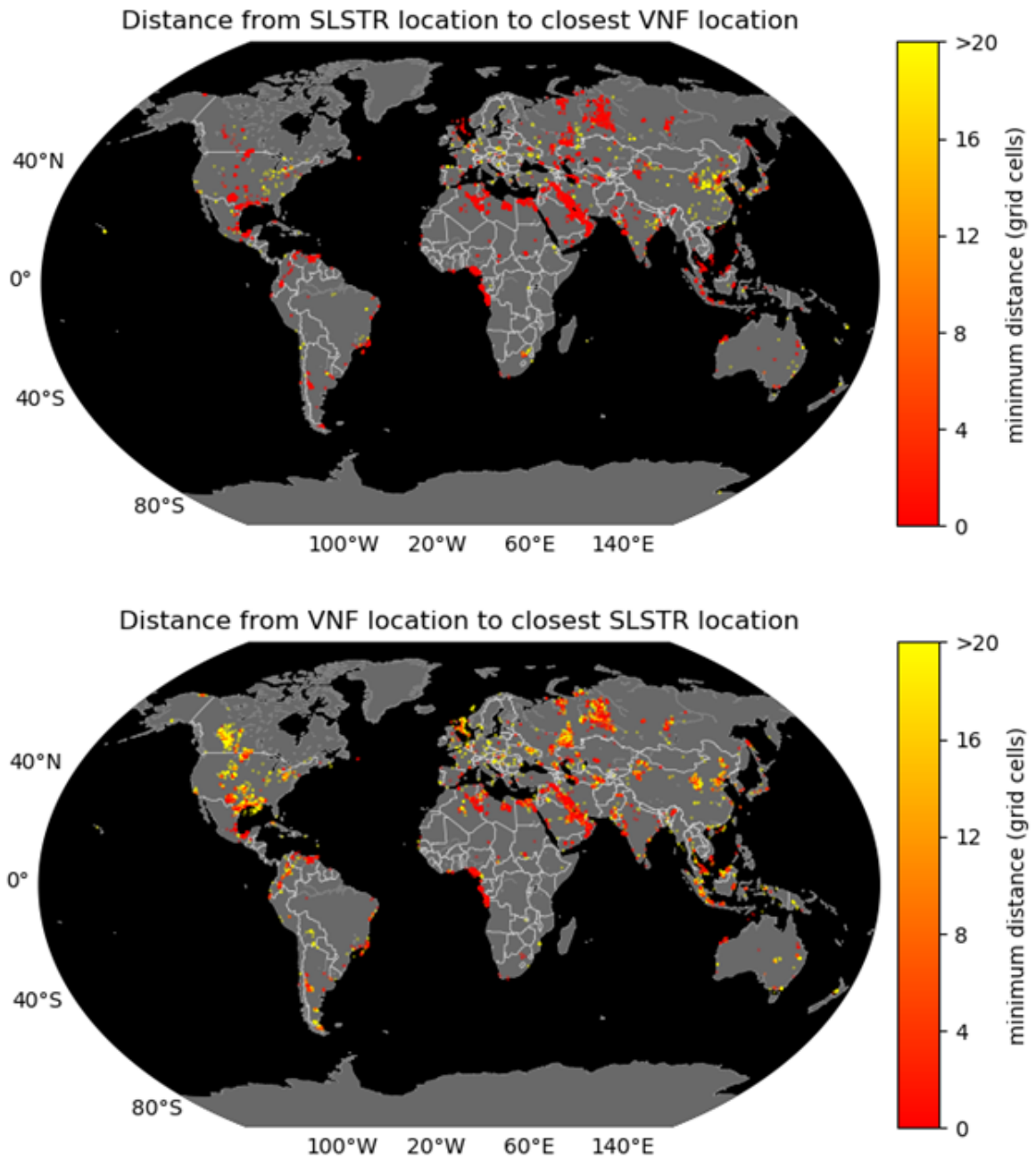
Figure 18. Minimum distance from a SLSTR flaring locations at the closest VNF flaring location (upper map). Minimum distance from a VNF flaring locations at the closest SLSTR flaring location (lower map). The distances are measured in grid cells ( 0.025^\circ \times 0.025^\circ global grid). Of the 6232 VNF flaring sites, 2964 are coincident with SLSTR flaring sites and 2562 are directly adjacent. Of the 10185 VNF flaring sites, 2964 are coincident with SLSTR flaring sites and 1507 are directly adjacent.
