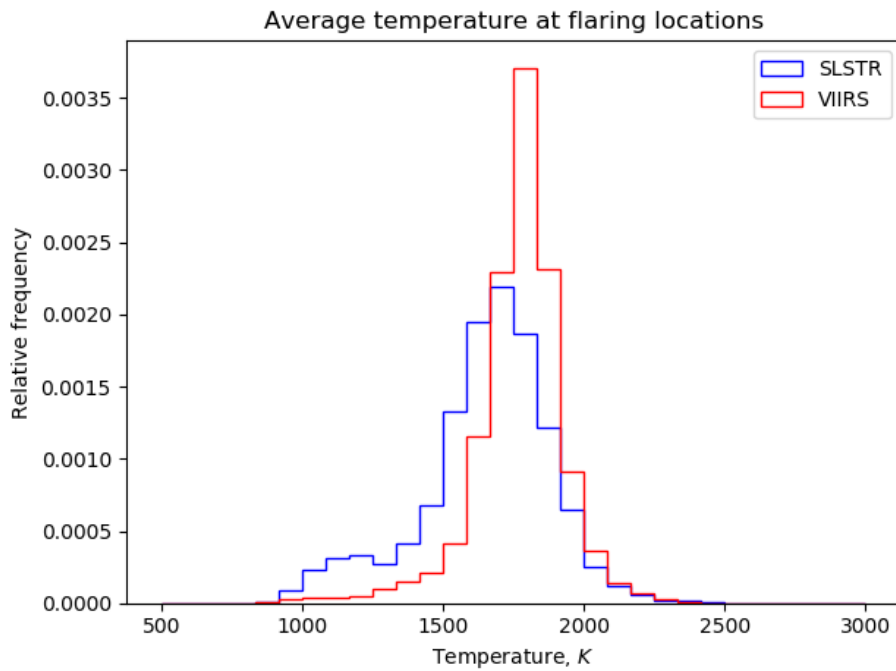
Figure 21. Comparison of the average retrieved temperature at the flaring locations for VIIRS Nightfire (locations shown in Figure 16 in red) and for SLSTR (locations shown in Figure 4 in blue). Relative frequency is used to ensure comparability independently of the total number of observations (6232 flaring locations for SLSTR, 10185 flaring locations for VIIRS Nightfire).
