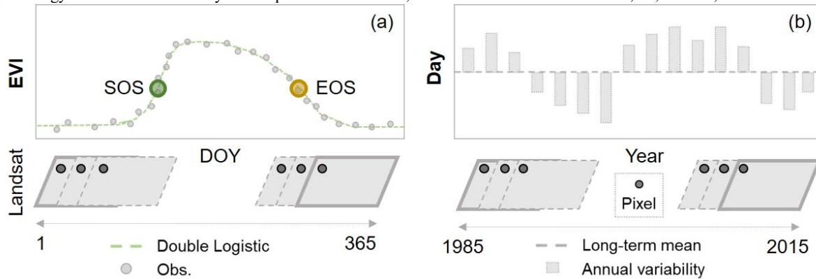
10 Fig. 1: The proposed framework for deriving long-term (1985-2015) mean vegetation phenology indicators (start of season-SOS and end of season - EOS) (a) and their annual variabilities (b).
