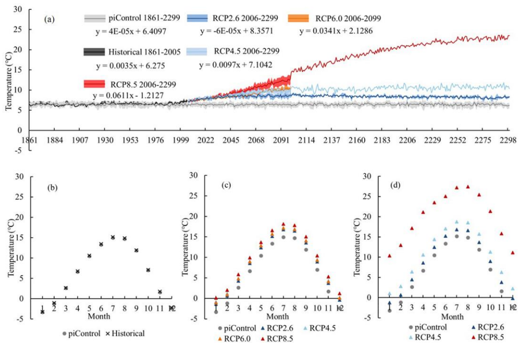
Figure 3 Inter-annual (a) and long-term averaged monthly dynamics (b-d) of the surface air temperature in the upper Yangtze River basin: comparison of the piControl scenario with the anthropogenic climate change scenarios (periods: a: 1861 - 2299; b: 1861 - 2005; c: 2006 - 2099; and d: 2100 - 2299)
